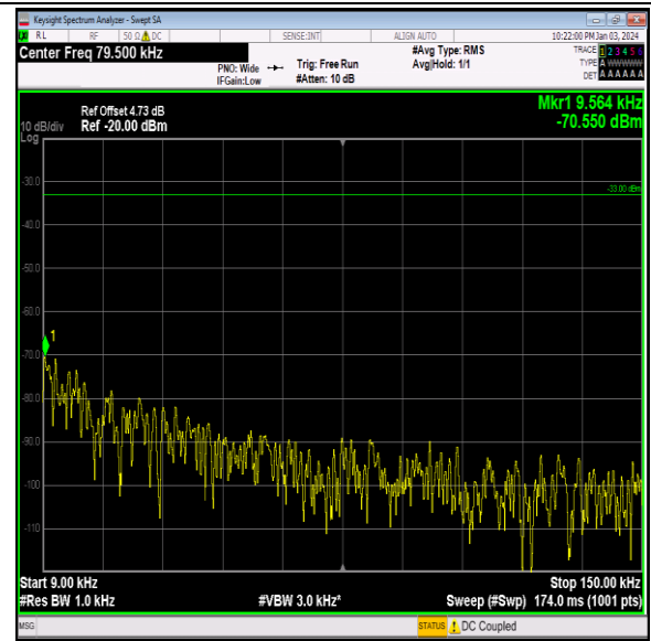
Band26_3MHz_QPSK_26775_1RB#0_0.009~0.15_0.009~ 0.15
