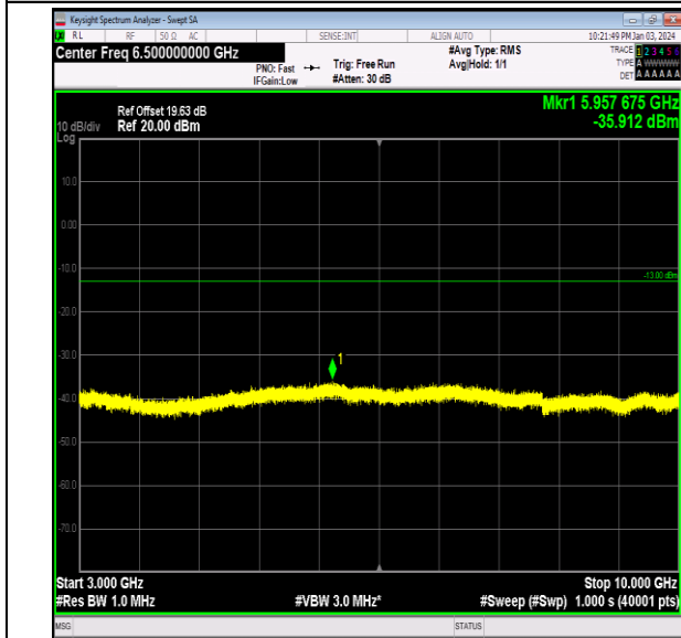
Band26_3MHz_64QAM_26740_1RB#0_3000~10000_300 0~10000
