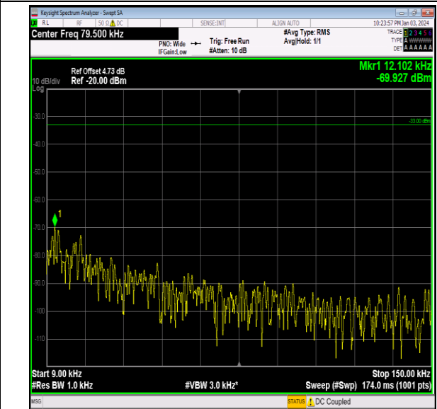
Band26_3MHz_64QAM_26775_1RB#0_0.009~0.15_0.009 ~0.15
