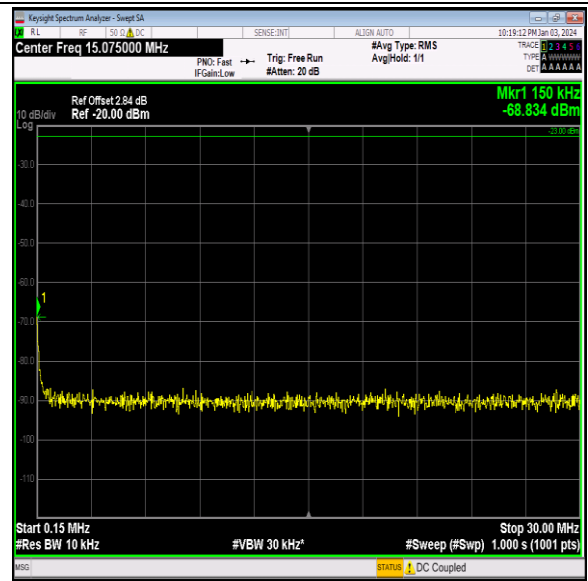
Band26_3MHz_QPSK_26740_1RB#0_0.15~30_0.15~30
