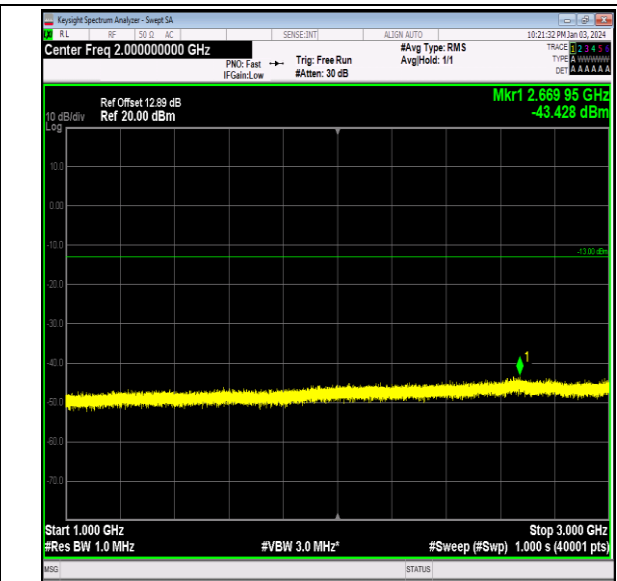
Band26_3MHz_64QAM_26740_1RB#0_1000~3000_1000 ~3000
