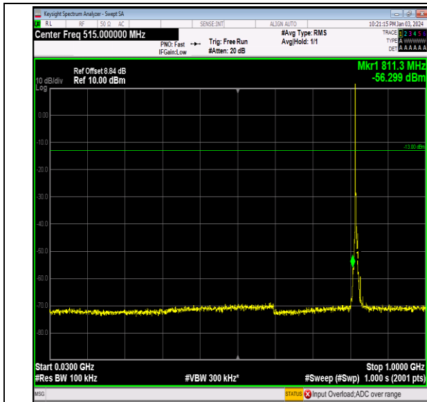
Band26_3MHz_64QAM_26740_1RB#0_30~1000_30~100 0
