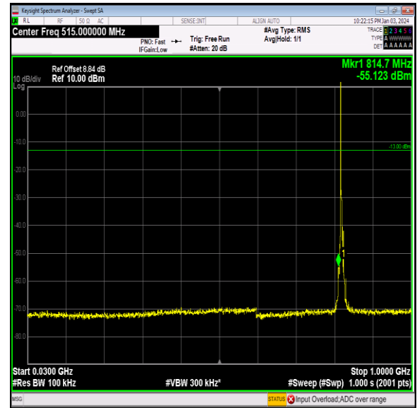
Band26_3MHz_QPSK_26775_1RB#0_30~1000_30~1000
