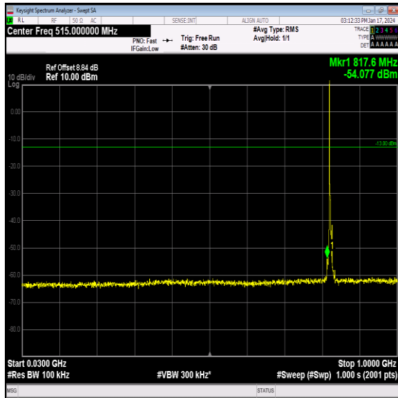
Band26_3MHz_16QAM_26805_1RB#0_30~1000_30~100 0
