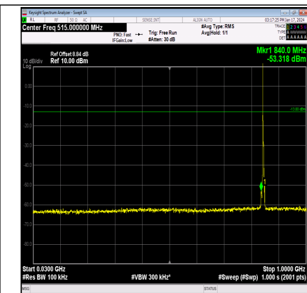
Band26_3MHz_QPSK_27025_1RB#0_30~1000_30~1000
