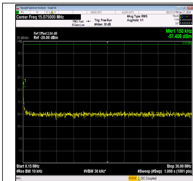
Band26_3MHz_QPSK_27025_1RB#0_0.15~30_0.15~30
