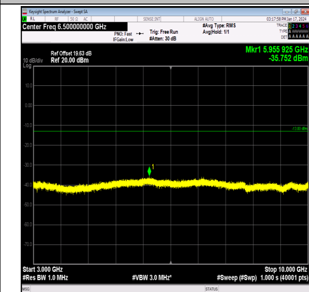
Band26_3MHz_QPSK_27025_1RB#0_3000~10000_3000~10000
