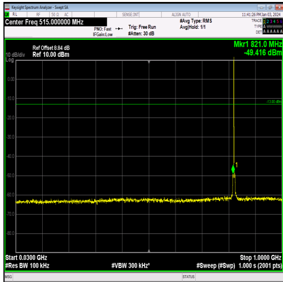
Band26_1.4MHz_QPSK_26797_1RB#0_30~1000_30~100 0
