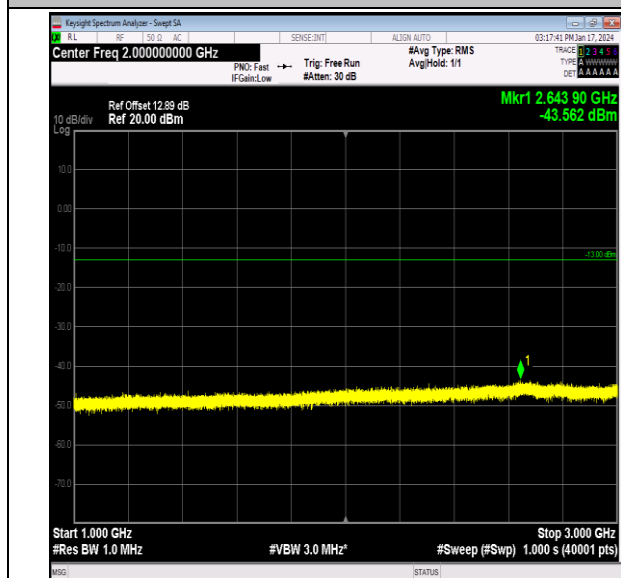
Band26_3MHz_QPSK_27025_1RB#0_1000~3000_1000~3000
