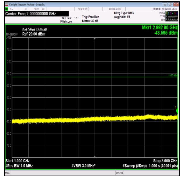
Band26_1.4MHz_QPSK_26797_1RB#0_1000~3000_1000 ~3000
