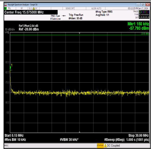
Band26_3MHz_16QAM_26805_1RB#0_0.15~30_0.15~30
