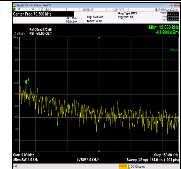
Band26_3MHz_QPSK_27025_1RB#0_0.009~0.15_0.009~0.15
