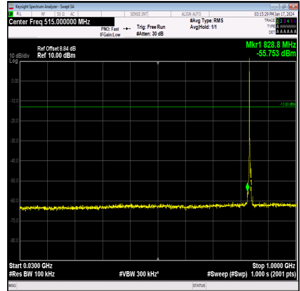
Band26_3MHz_16QAM_26915_1RB#0_30~1000_30~100 0
