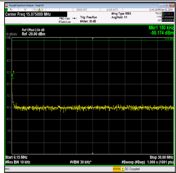
Band26_1.4MHz_QPSK_26797_1RB#0_0.15~30_0.15~30
