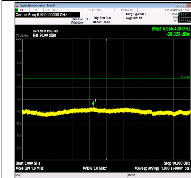
Band26_3MHz_QPSK_26915_1RB#0_3000~10000_3000~10000
