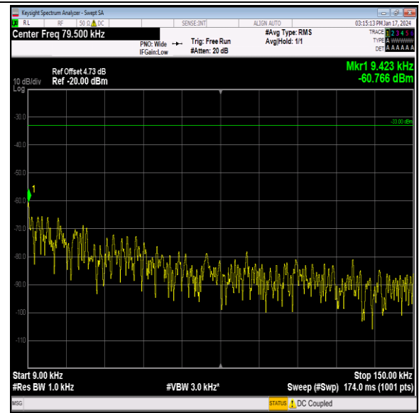
Band26_3MHz_16QAM_26915_1RB#0_0.009~0.15_0.009 ~0.15
