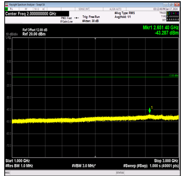
Band26_3MHz_16QAM_26805_1RB#0_1000~3000_1000 ~3000
