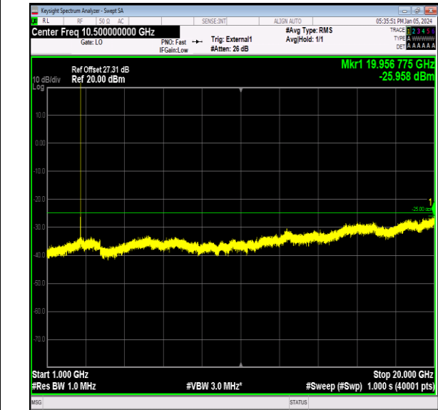
Band41_5MHz_64QAM_41215_1RB#0_1000~20000_100 0~20000
