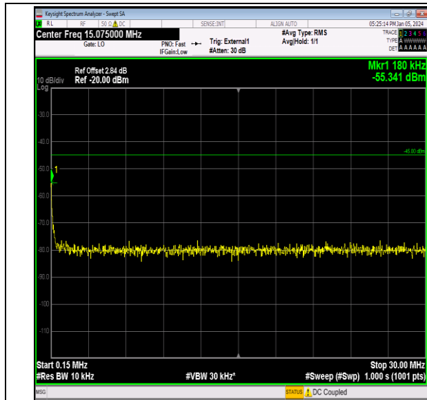
Band41_5MHz_QPSK_40640_1RB#0_0.15~30_0.15~30
