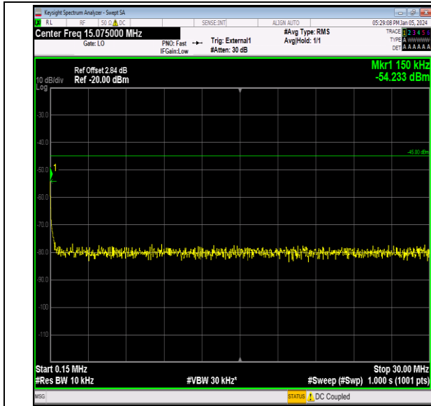
Band41_5MHz_64QAM_40640_1RB#0_0.15~30_0.15~30
