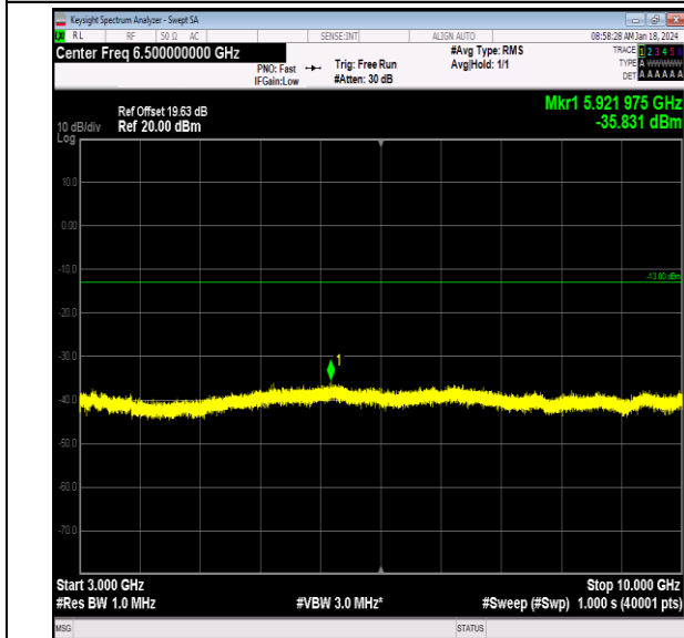
Band26_15MHz_64QAM_26865_1RB#0_3000~10000_30 00~10000
