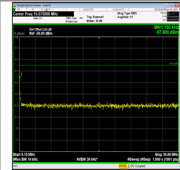
Band41_5MHz_64QAM_41215_1RB#0_0.15~30_0.15~30
