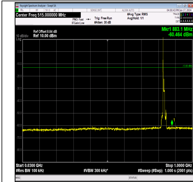
Band26_10MHz_64QAM_26915_1RB#0_30~1000_30~10 00
