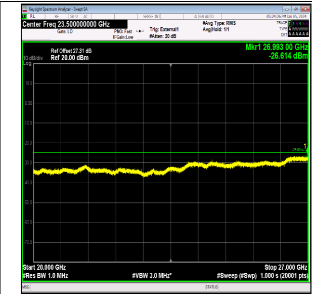
Band41_5MHz_64QAM_40065_1RB#0_20000~27000_20 000~27000
