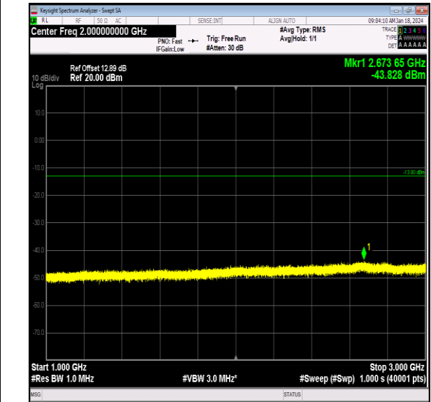
Band26_15MHz_64QAM_26965_1RB#0_1000~3000_100 0~3000
