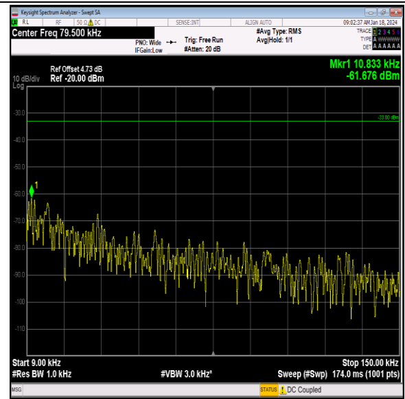
Band26_15MHz_16QAM_26965_1RB#0_0.009~0.15_0.00 9~0.15
