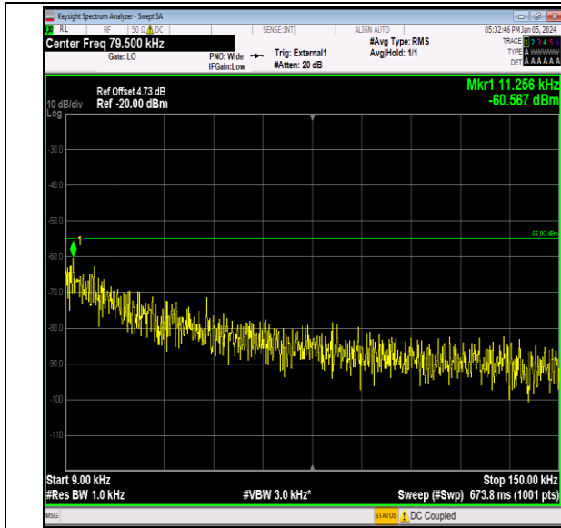
Band41_5MHz_16QAM_41215_1RB#0_0.009~0.15_0.009 ~0.15
