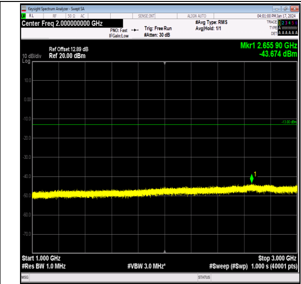
Band26_10MHz_64QAM_26915_1RB#0_1000~3000_100 0~3000
