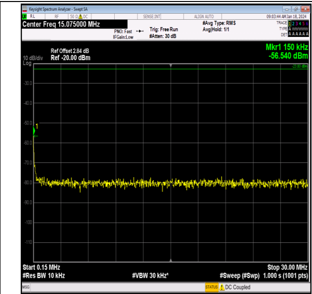
Band26_15MHz_64QAM_26965_1RB#0_0.15~30_0.15~3 0
