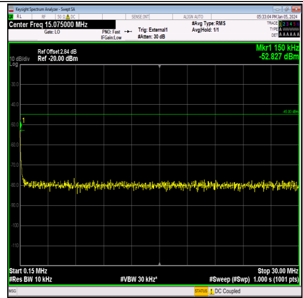
Band41_5MHz_16QAM_41215_1RB#0_0.15~30_0.15~30
