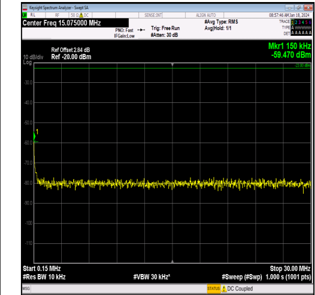
Band26_15MHz_64QAM_26865_1RB#0_0.15~30_0.15~3 0
