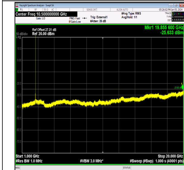
Band41_5MHz_QPSK_40640_1RB#0_1000~20000_1000 ~20000
