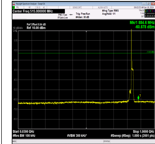
Band26_15MHz_64QAM_26965_1RB#0_30~1000_30~10 00
