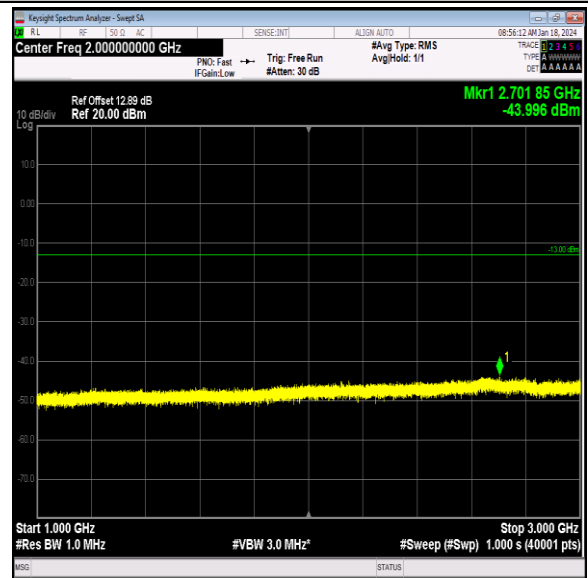
Band26_15MHz_QPSK_26865_1RB#0_1000~3000_1000 ~3000
