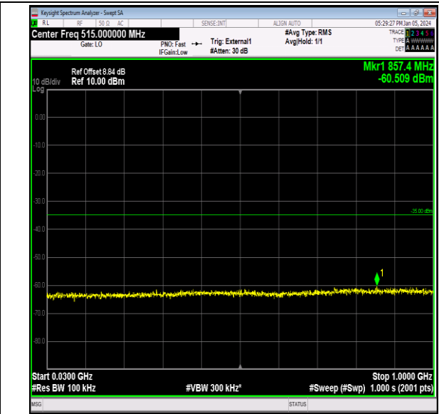
Band41_5MHz_64QAM_40640_1RB#0_30~1000_30~1000 0
