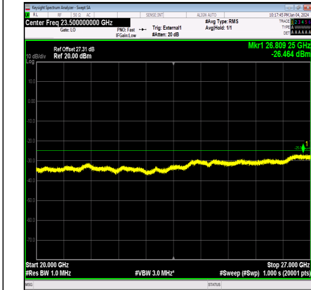
Band41_5MHz_64QAM_40590_1RB#0_20000~27000_20 000~27000
