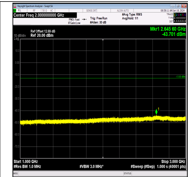
Band26_15MHz_64QAM_26865_1RB#0_1000~3000_100 0~3000
