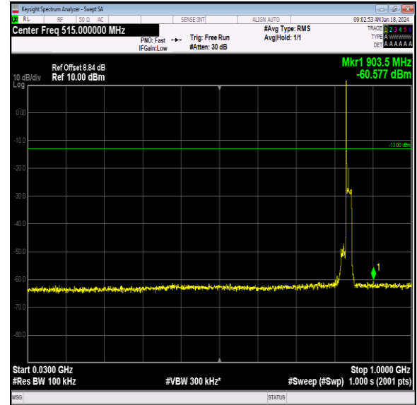
Band26_15MHz_16QAM_26965_1RB#0_30~1000_30~10 00
