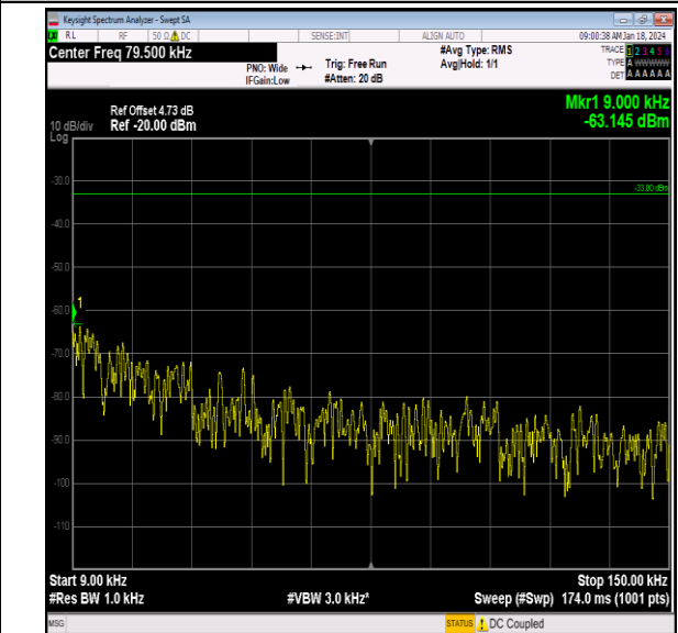
Band26_15MHz_64QAM_26915_1RB#0_0.009~0.15_0.00 9~0.15
