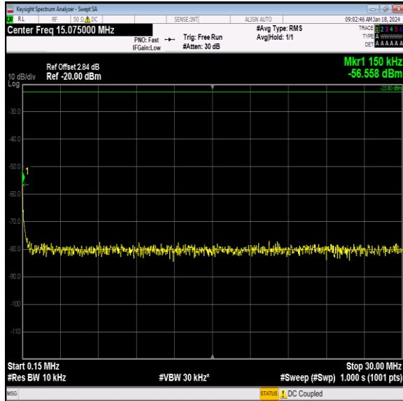
Band26_15MHz_16QAM_26965_1RB#0_0.15~30_0.15~3 0
