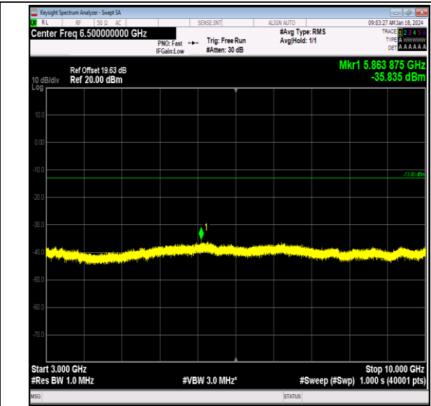
Band26_15MHz_16QAM_26965_1RB#0_3000~10000_30 00~10000
