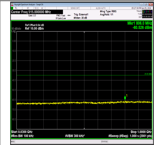
Band41_5MHz_16QAM_40640_1RB#0_30~1000_30~1000 0
