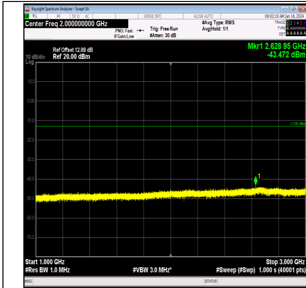
Band26_15MHz_16QAM_26965_1RB#0_1000~3000_100 0~3000
