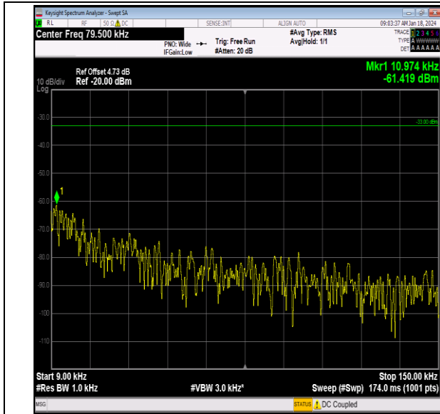
Band26_15MHz_64QAM_26965_1RB#0_0.009~0.15_0.00 9~0.15
