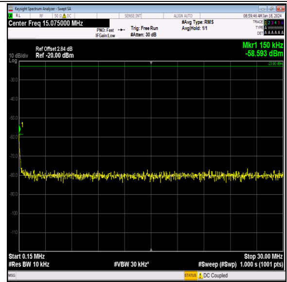
Band26_15MHz_16QAM_26915_1RB#0_0.15~30_0.15~3 0
