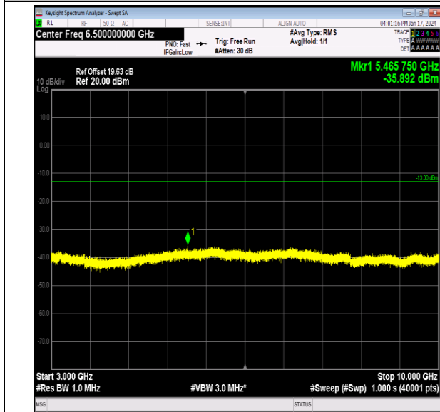
Band26_10MHz_64QAM_26915_1RB#0_3000~10000_30 00~10000
