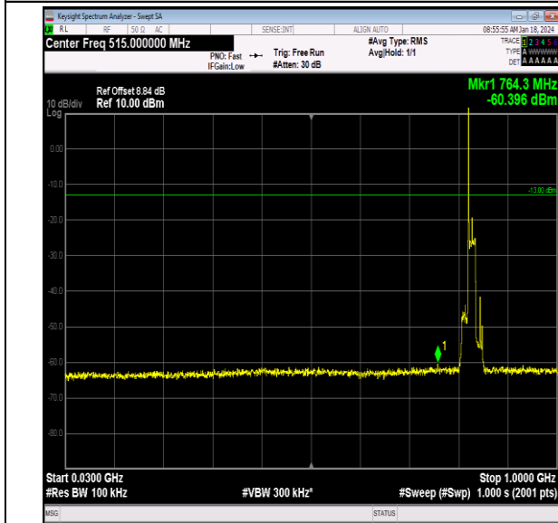
Band26_15MHz_QPSK_26865_1RB#0_30~1000_30~100 0
