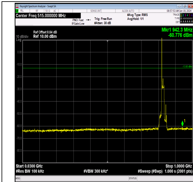
Band26_15MHz_64QAM_26865_1RB#0_30~1000_30~10 00
