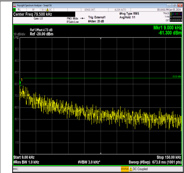
Band41_5MHz_QPSK_40065_1RB#0_0.009~0.15_0.009~0.15
