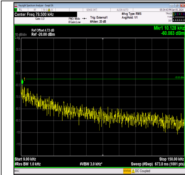
Band41_5MHz_64QAM_41215_1RB#0_0.009~0.15_0.009 ~0.15
