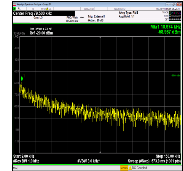
Band41_5MHz_64QAM_40640_1RB#0_0.009~0.15_0.009 ~0.15
