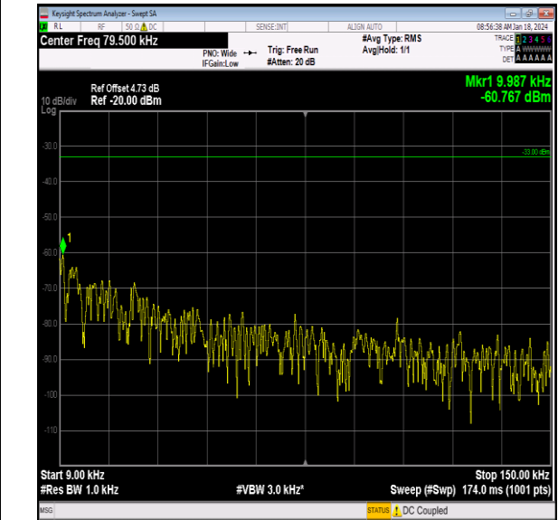
Band26_15MHz_16QAM_26865_1RB#0_0.009~0.15_0.00 9~0.15
