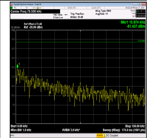
Band26_10MHz_64QAM_26990_1RB#0_0.009~0.15_0.00 9~0.15
