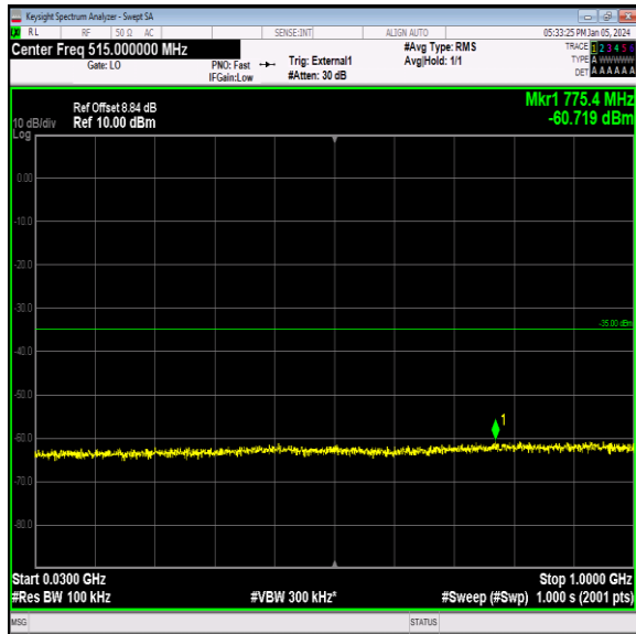
Band41_5MHz_16QAM_41215_1RB#0_30~1000_30~100 0
