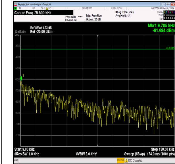
Band26_15MHz_64QAM_26865_1RB#0_0.009~0.15_0.00 9~0.15
