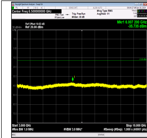
Band26_15MHz_64QAM_26965_1RB#0_3000~10000_3000~10000
