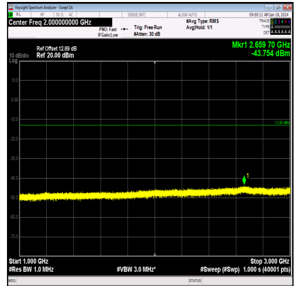
Band26_15MHz_16QAM_26915_1RB#0_1000~3000_100 0~3000
