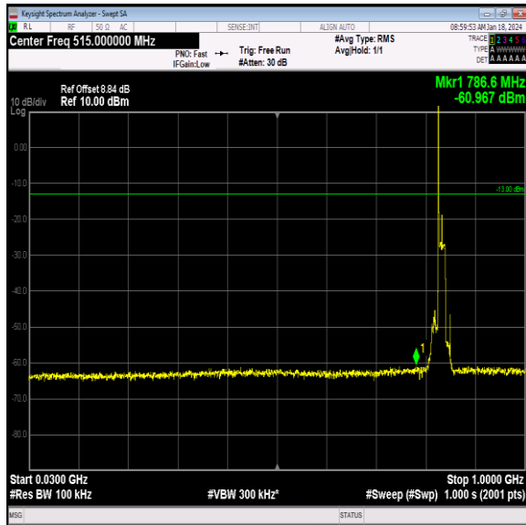
Band26_15MHz_16QAM_26915_1RB#0_30~1000_30~10 00
