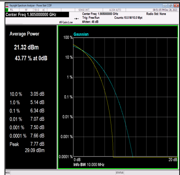
Band2-10MHz-64QAM-19150-50RB#0-PASS
