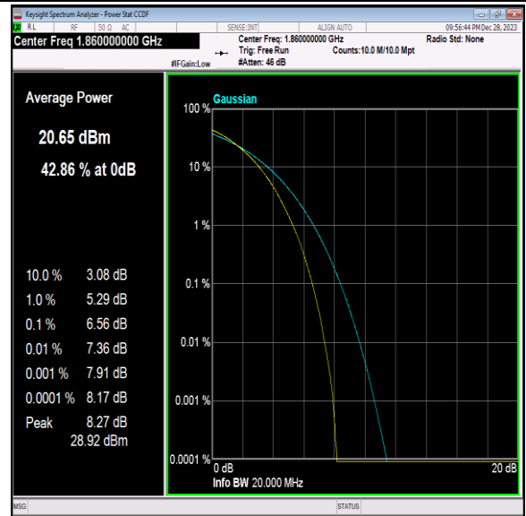
Band2-20MHz-64QAM-18700-100RB#0-PASS
