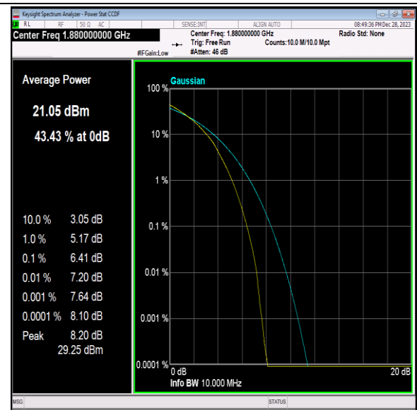
Band2-10MHz-64QAM-18900-50RB#0-PASS
