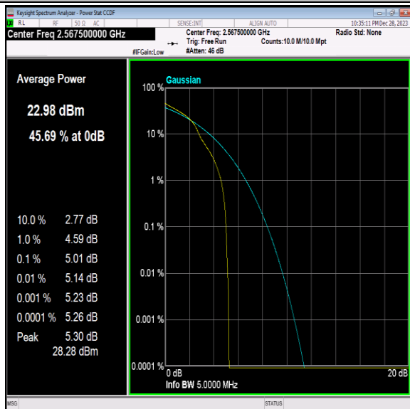
Band7-5MHz-16QAM-21425-1RB#0-PASS
