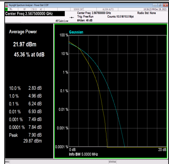
Band7-5MHz-16QAM-21425-25RB#0-PASS
