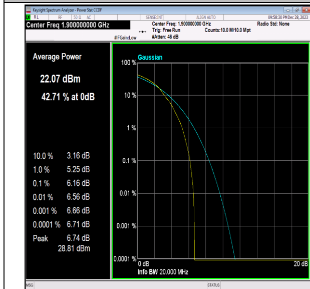
Band2-20MHz-64QAM-19100-1RB#0-PASS
