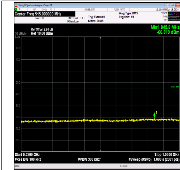
Band41_20MHz_QPSK_40140_1RB#0_30~1000_30~100 0
