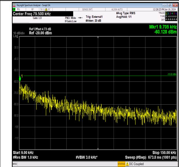
Band41_20MHz_QPSK_40640_1RB#0_0.009~0.15_0.009 ~0.15
