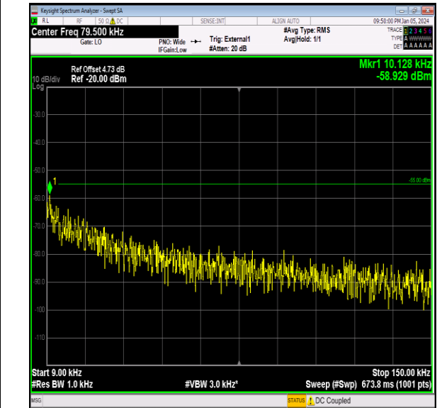
Band41_10MHz_QPSK_40640_1RB#0_0.009~0.15_0.009 ~0.15
