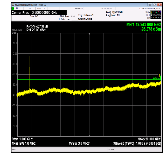
Band41_20MHz_QPSK_40140_1RB#0_1000~20000_100 0~20000
