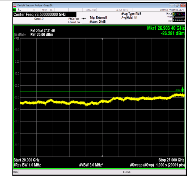
Band41_10MHz_64QAM_40090_1RB#0_20000~27000_2 0000~27000
