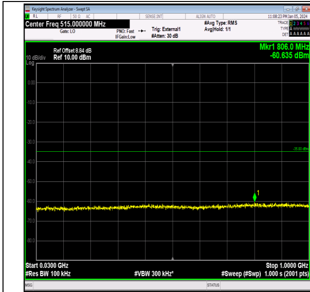
Band41_15MHz_QPSK_40640_1RB#0_30~1000_30~100 0
