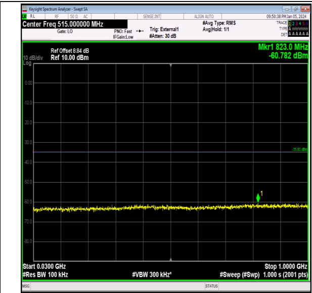
Band41_10MHz_QPSK_40640_1RB#0_30~1000_30~100 0
