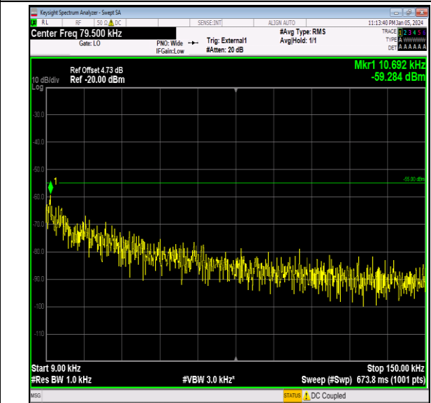
Band41_15MHz_QPSK_41165_1RB#0_0.009~0.15_0.009 ~0.15
