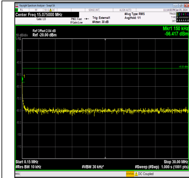
Band41_15MHz_QPSK_41165_1RB#0_0.15~30_0.15~30
