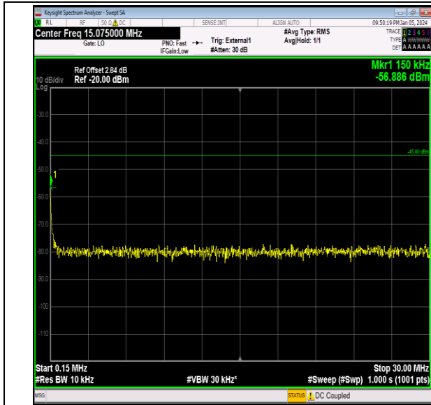
Band41_10MHz_QPSK_40640_1RB#0_0.15~30_0.15~30
