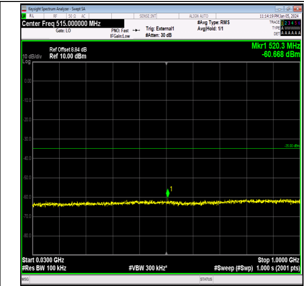
Band41_15MHz_QPSK_41165_1RB#0_30~1000_30~100 0
