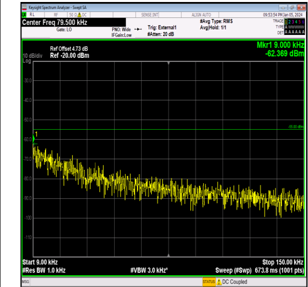
Band41_10MHz_64QAM_40640_1RB#0_0.009~0.15_0.00 9~0.15
