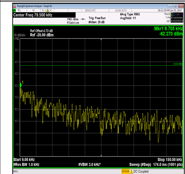
Band66_3MHz_64QAM_132322_1RB#0_0.009~0.15_0.00 9~0.15
