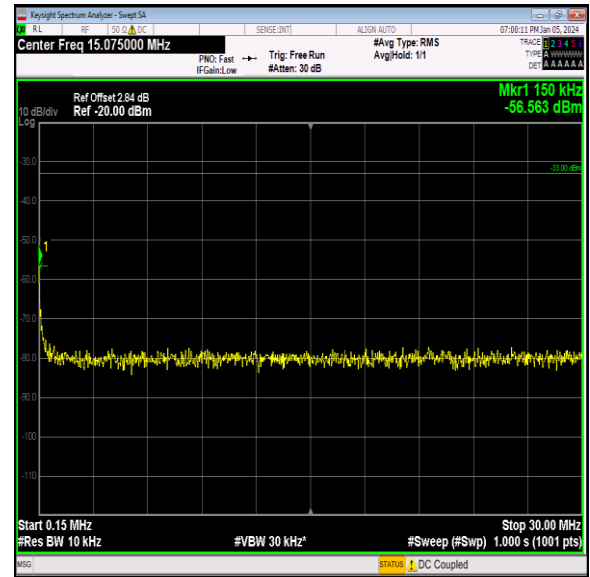
Band66_5MHz_QPSK_132322_1RB#0_0.15~30_0.15~30
