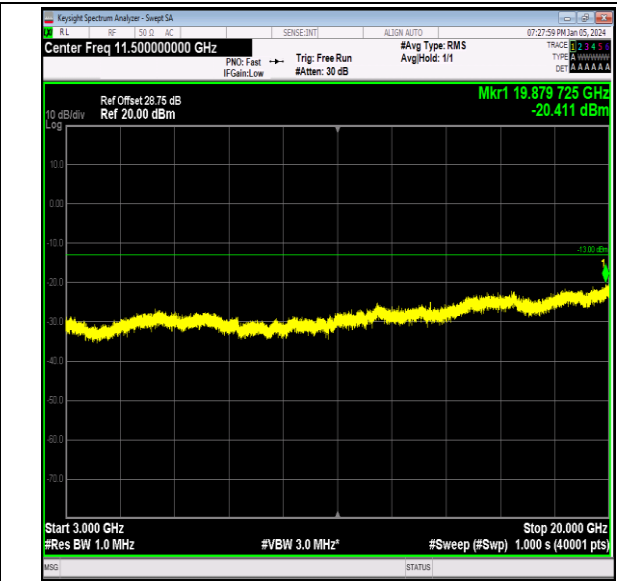
Band66_10MHz_16QAM_132022_1RB#0_3000~20000_3 000~20000
