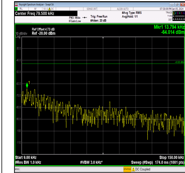
Band66_10MHz_16QAM_132322_1RB#0_0.009~0.15_0.0 09~0.15
