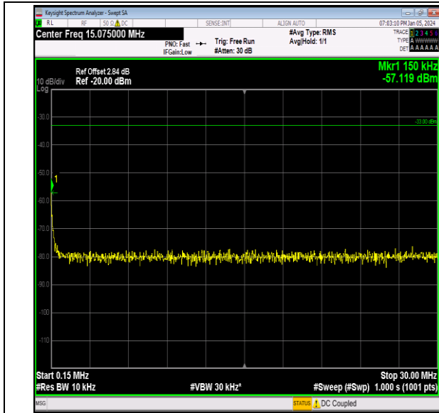
Band66_5MHz_QPSK_132647_1RB#0_0.15~30_0.15~30
