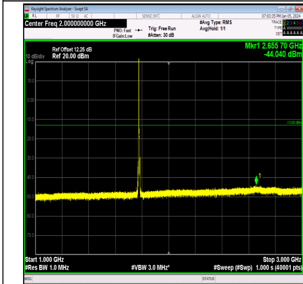
Band66_5MHz_QPSK_132647_1RB#0_1000~3000_1000~3000
