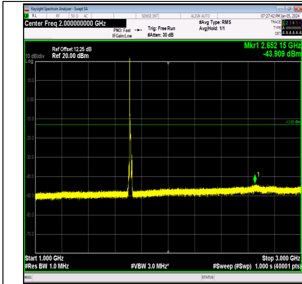
Band66_10MHz_16QAM_132022_1RB#0_1000~3000_10 00~3000
