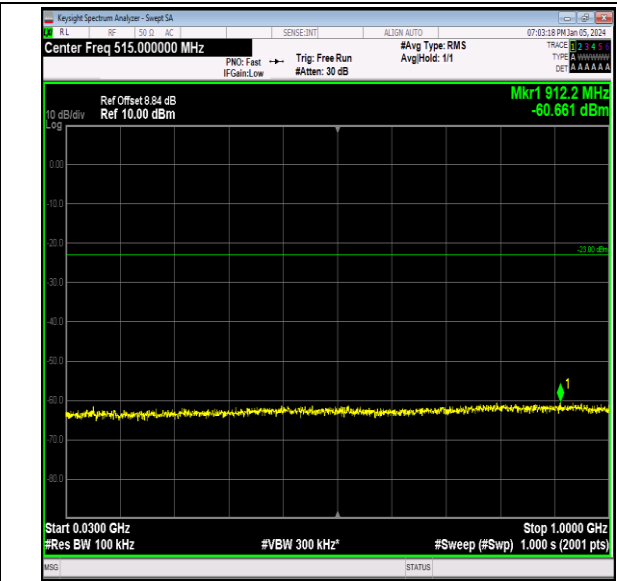
Band66_5MHz_QPSK_132647_1RB#0_30~1000_30~1000
