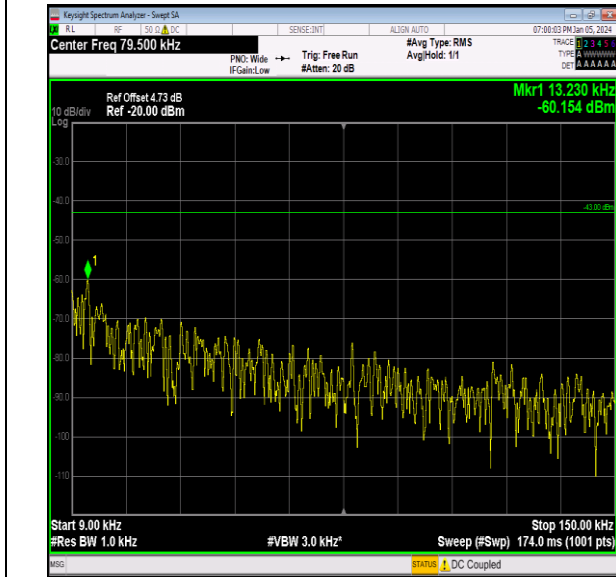
Band66_5MHz_QPSK_132322_1RB#0_0.009~0.15_0.009 ~0.15
