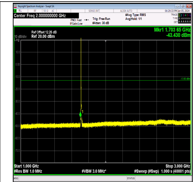
Band66_3MHz_64QAM_131987_1RB#0_1000~3000_100 0~3000
