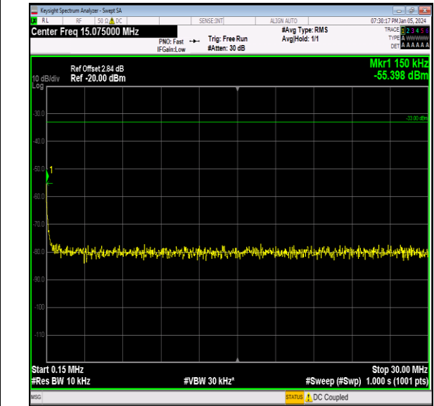
Band66_10MHz_16QAM_132322_1RB#0_0.15~30_0.15~ 30
