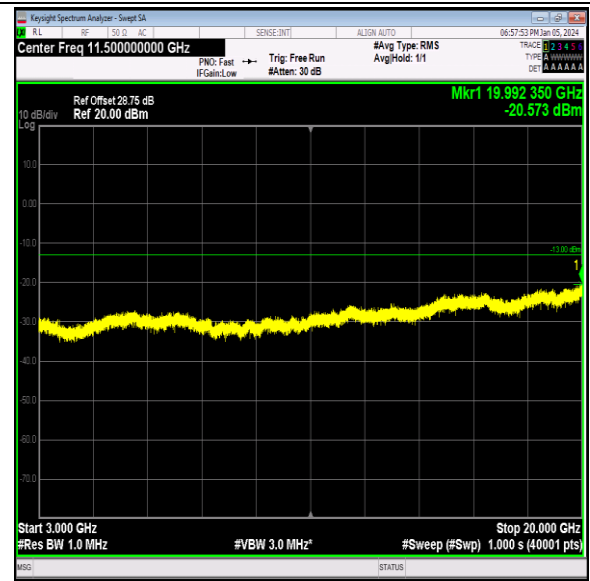
Band66_5MHz_QPSK_131997_1RB#0_3000~20000_300 0~20000
