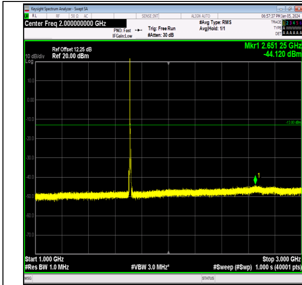
Band66_5MHz_QPSK_131997_1RB#0_1000~3000_1000 ~3000
