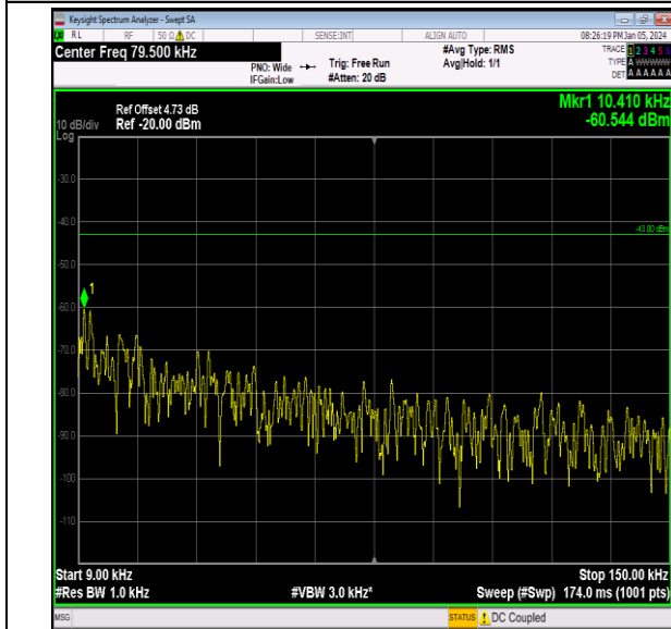
Band66_20MHz_QPSK_132572_1RB#0_0.009~0.15_0.00 9~0.15
