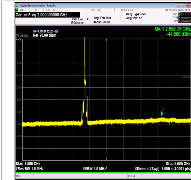
Band66_20MHz_QPSK_132322_1RB#0_1000~3000_100 0~3000
