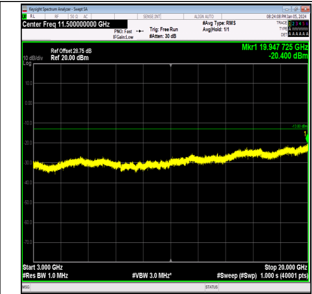
Band66_20MHz_QPSK_132322_1RB#0_3000~20000_30 00~20000
