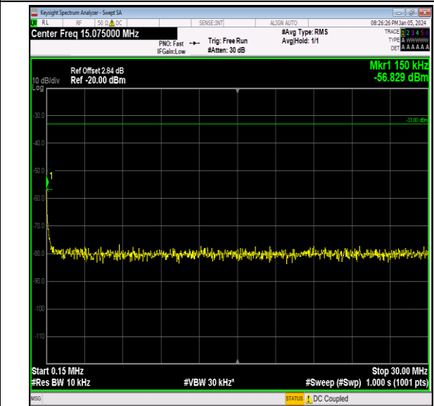
Band66_20MHz_QPSK_132572_1RB#0_0.15~30_0.15~3 0
