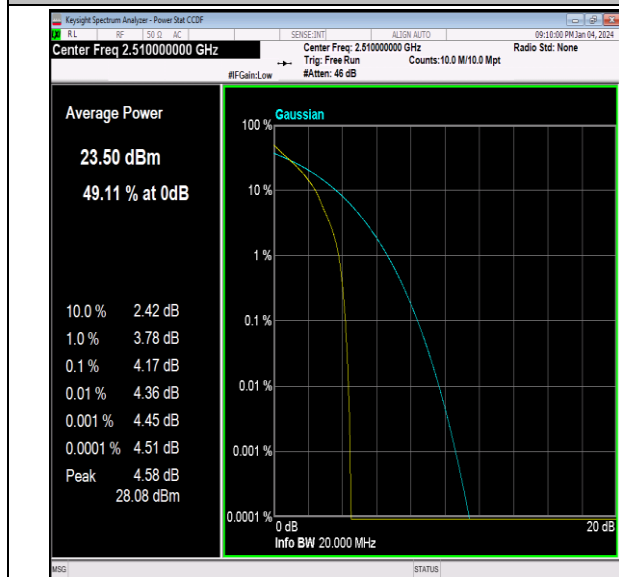
Band7-20MHz-64QAM-20850-1RB#0-PASS
