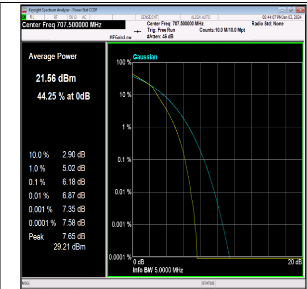
Band12-5MHz-16QAM-23095-25RB#0-PASS
