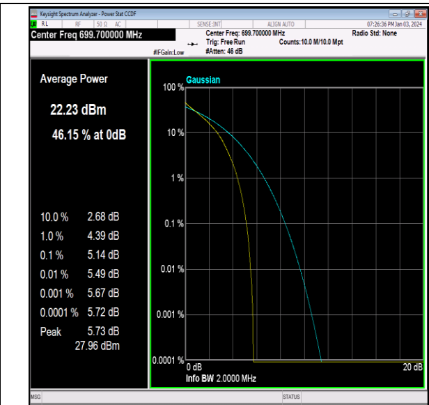
Band12-1.4MHz-64QAM-23017-6RB#0-PASS
