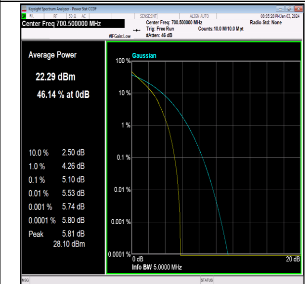
Band12-3MHz-64QAM-23025-15RB#0-PASS
