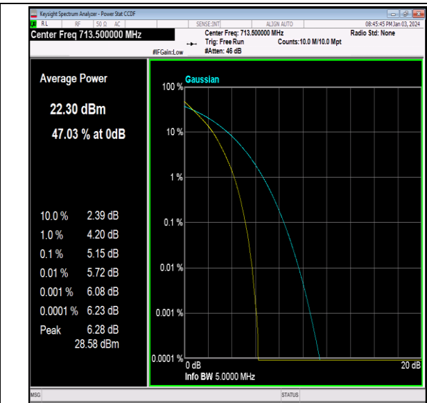
Band12-5MHz-QPSK-23155-25RB#0-PASS
