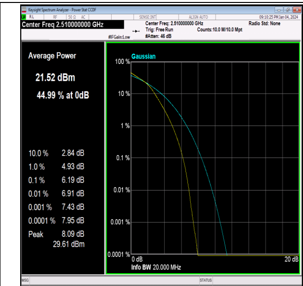
Band7-20MHz-16QAM-20850-100RB#0-PASS
