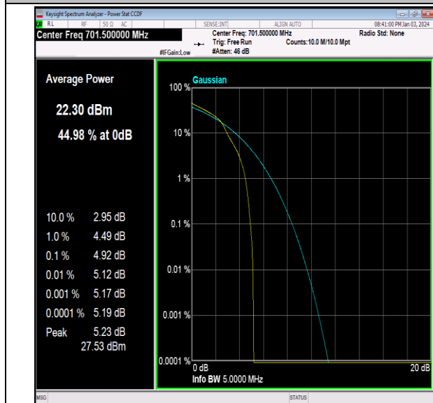
Band12-5MHz-16QAM-23035-1RB#0-PASS
