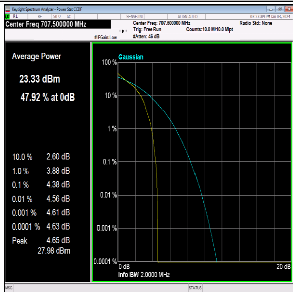
Band12-1.4MHz-QPSK-23095-1RB#0-PASS
