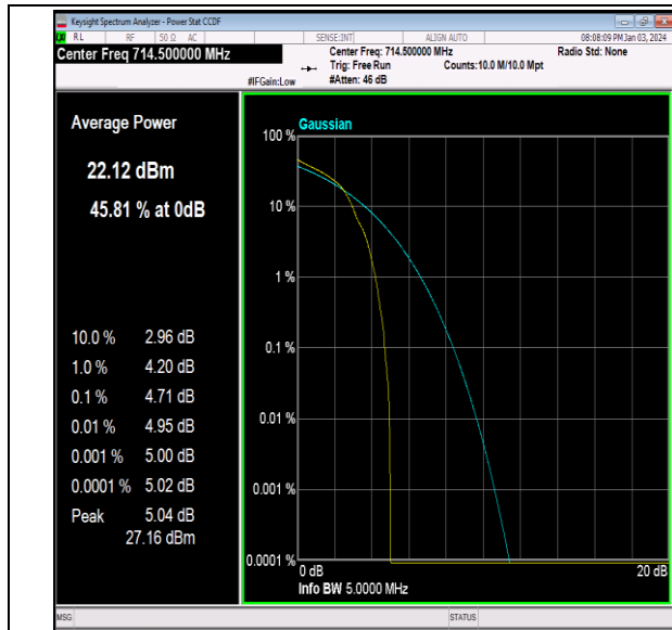
Band12-3MHz-16QAM-23165-1RB#0-PASS
