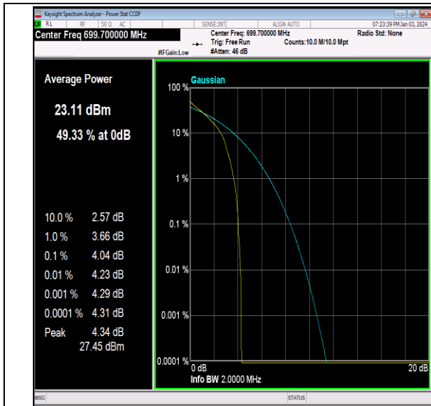
Band12-1.4MHz-QPSK-23017-1RB#0-PASS
