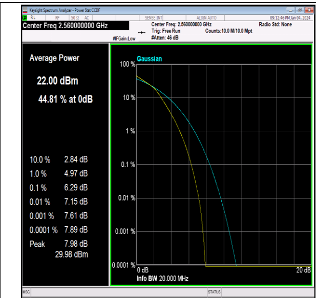
Band7-20MHz-16QAM-21350-100RB#0-PASS
