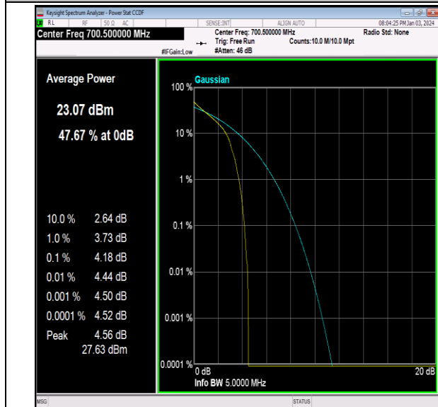
Band12-3MHz-64QAM-23025-1RB#0-PASS
