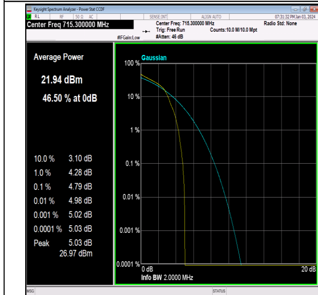
Band12-1.4MHz-16QAM-23173-1RB#0-PASS
