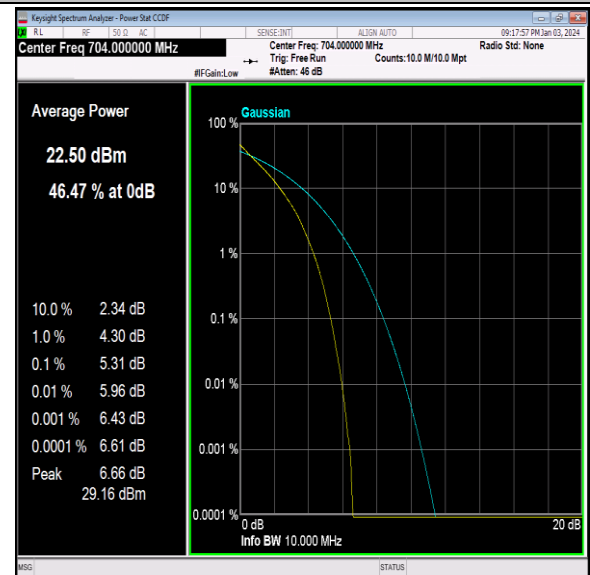
Band12-10MHz-QPSK-23060-50RB#0-PASS
