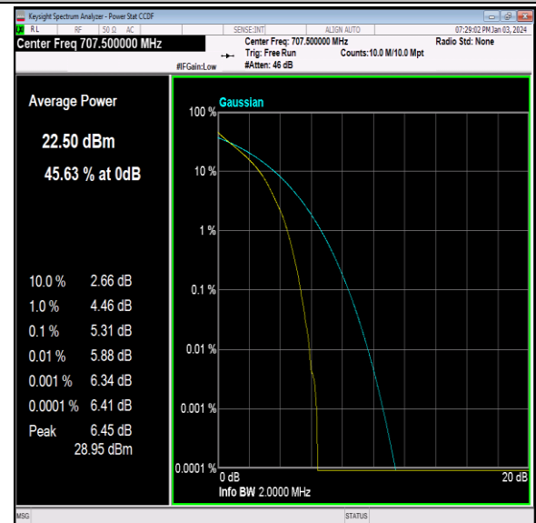
Band12-1.4MHz-QPSK-23095-6RB#0-PASS
