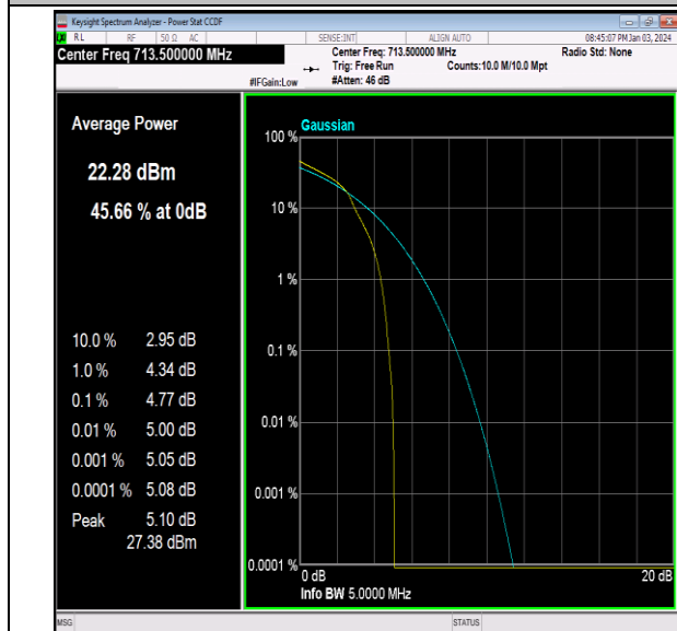
Band12-5MHz-16QAM-23155-1RB#0-PASS
