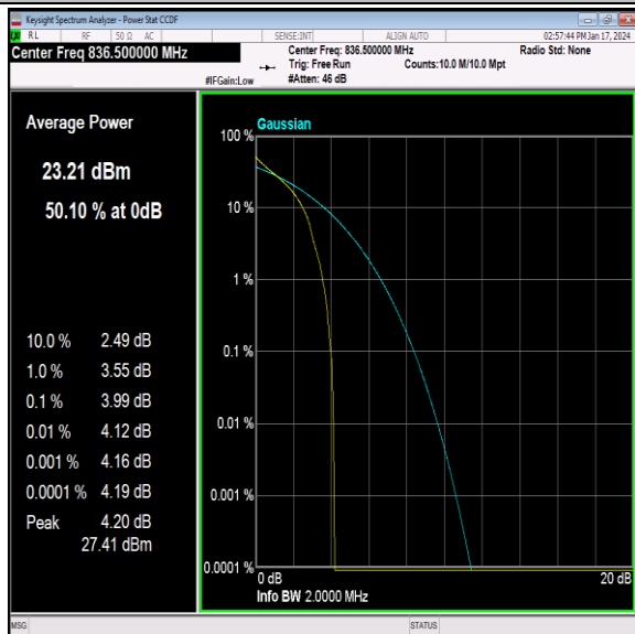
26(824-849)-1.4MHz-QPSK-26915-1RB#0-PASS
