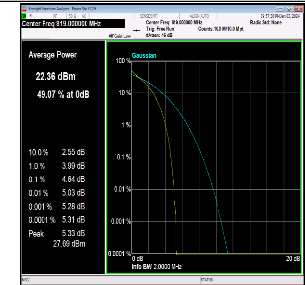
26(814-824)-1.4MHz-QPSK-26740-6RB#0-PASS
