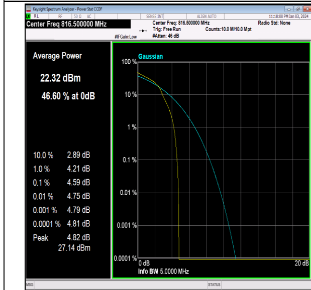
26(814-824)-5MHz-16QAM-26715-1RB#0-PASS
