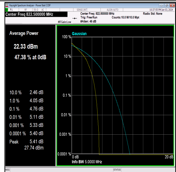
26(814-824)-3MHz-64QAM-26775-15RB#0-PASS
