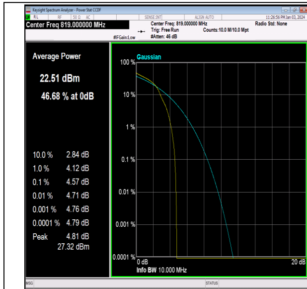
26(814-824)-10MHz-16QAM-26740-1RB#0-PASS
