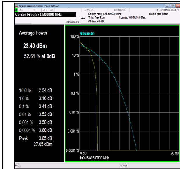
26(814-824)-5MHz-QPSK-26765-1RB#0-PASS
