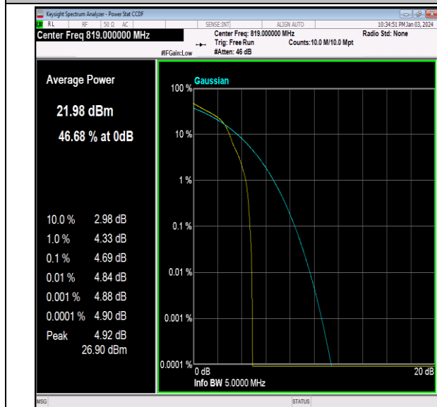
26(814-824)-3MHz-16QAM-26740-1RB#0-PASS
