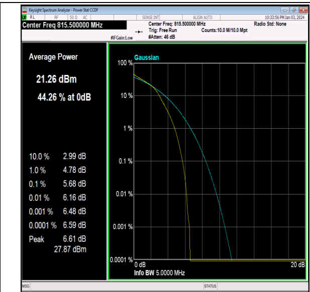
26(814-824)-3MHz-16QAM-26705-15RB#0-PASS
