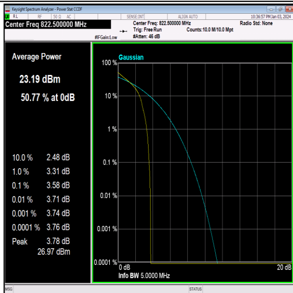
26(814-824)-3MHz-64QAM-26775-1RB#0-PASS
