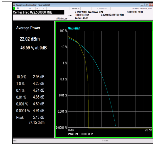
26(814-824)-3MHz-16QAM-26775-1RB#0-PASS
