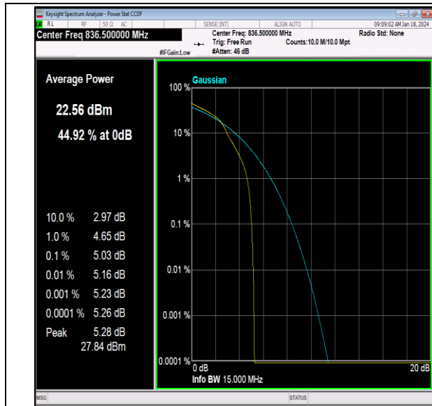
26(824-849)-15MHz-16QAM-26915-1RB#0-PASS
