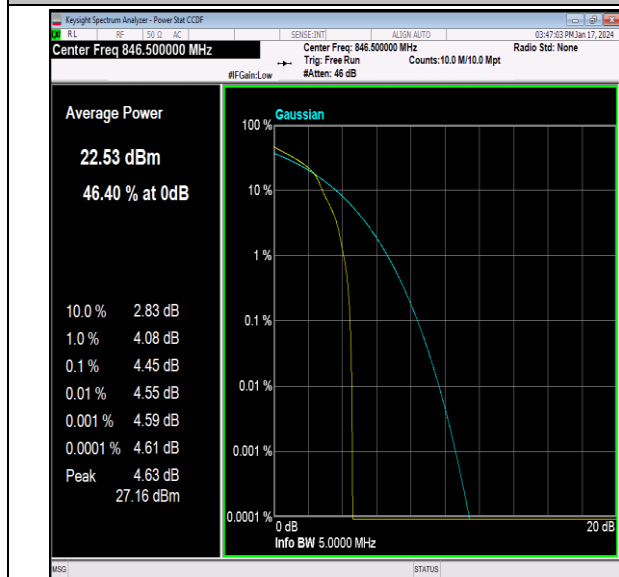
26(824-849)-5MHz-16QAM-27015-1RB#0-PASS
