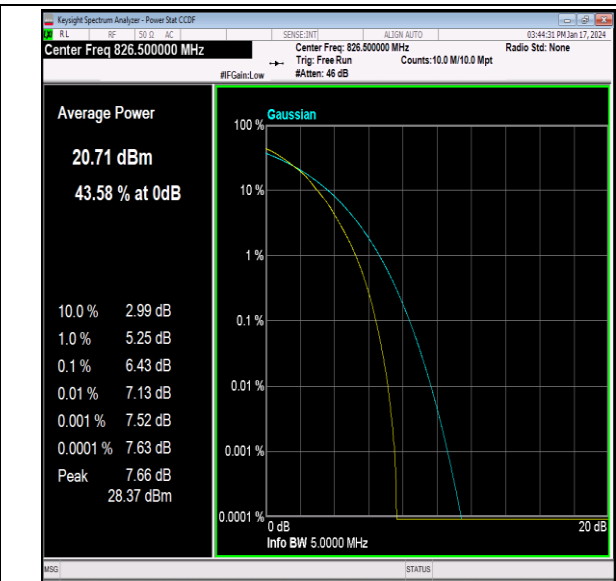
26(824-849)-5MHz-64QAM-26815-25RB#0-PASS
