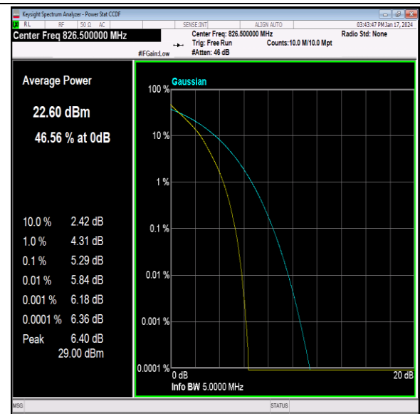
26(824-849)-5MHz-QPSK-26815-25RB#0-PASS
