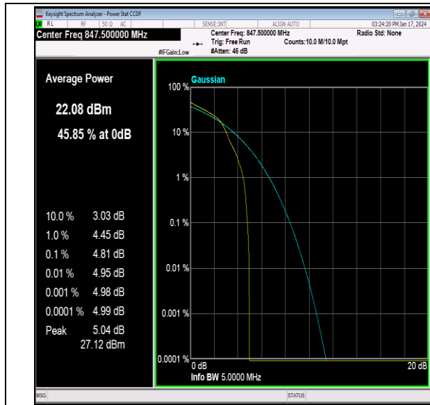
26(824-849)-3MHz-16QAM-27025-1RB#0-PASS
