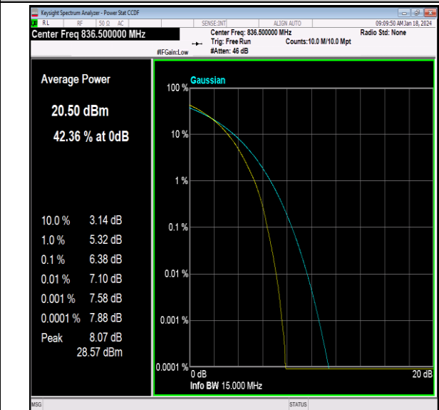
26(824-849)-15MHz-64QAM-26915-75RB#0-PASS
