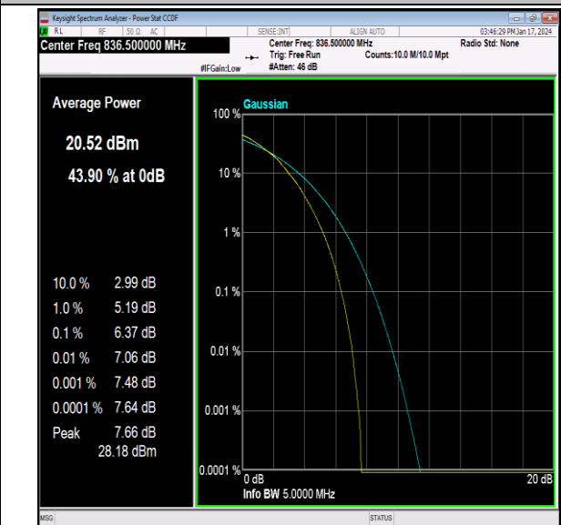
26(824-849)-5MHz-64QAM-26915-25RB#0-PASS
