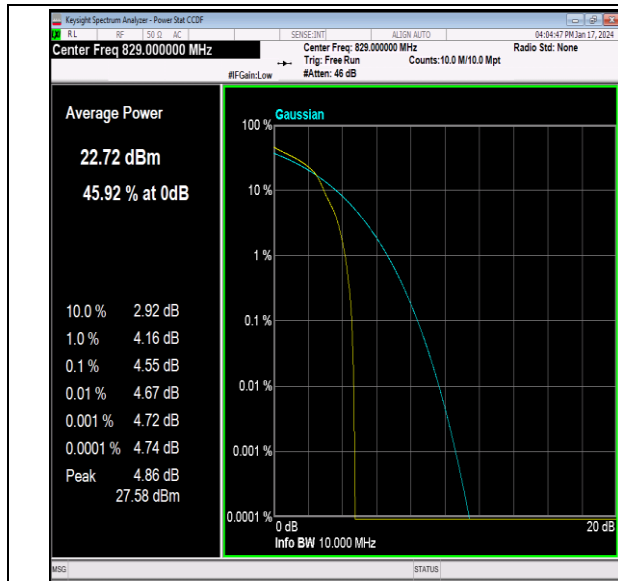
26(824-849)-10MHz-16QAM-26840-1RB#0-PASS
