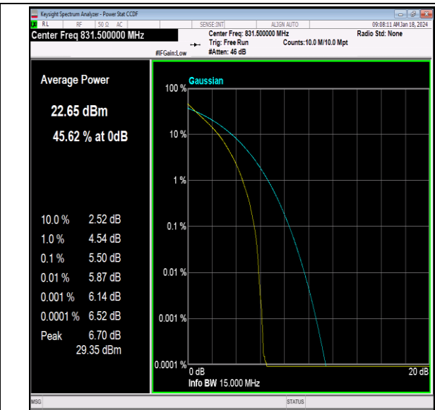
26(824-849)-15MHz-QPSK-26865-75RB#0-PASS
