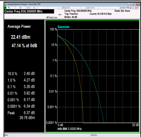
26(824-849)-5MHz-QPSK-26915-25RB#0-PASS
