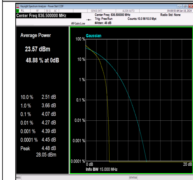
26(824-849)-15MHz-QPSK-26915-1RB#0-PASS
