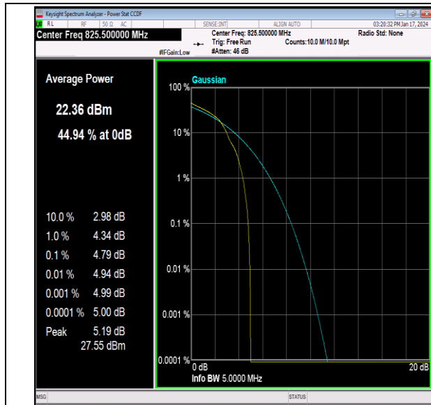
26(824-849)-3MHz-16QAM-26805-1RB#0-PASS
