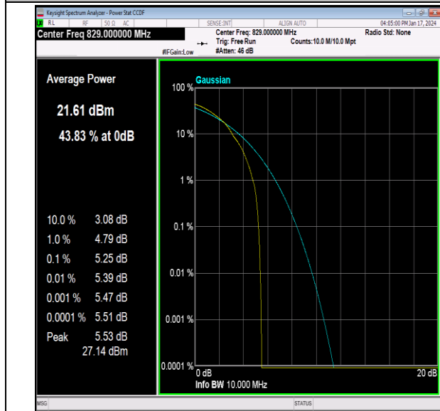
26(824-849)-10MHz-64QAM-26840-1RB#0-PASS
