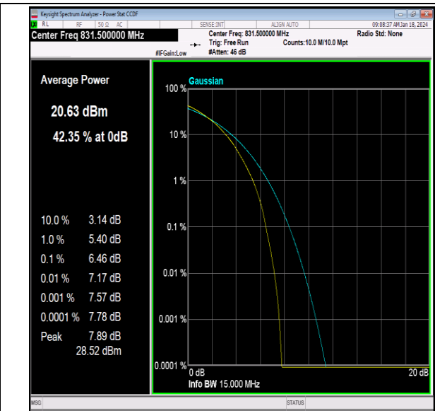
26(824-849)-15MHz-64QAM-26865-75RB#0-PASS
