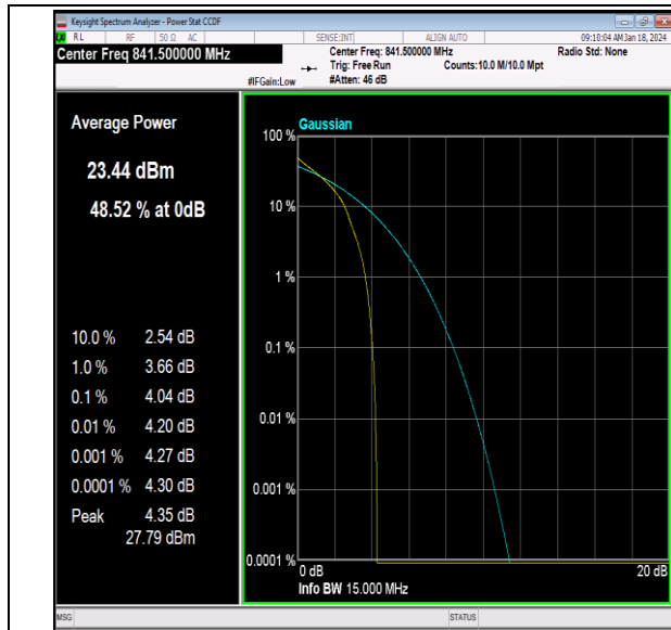
26(824-849)-15MHz-QPSK-26965-1RB#0-PASS
