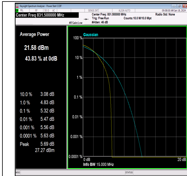
26(824-849)-15MHz-64QAM-26865-1RB#0-PASS
