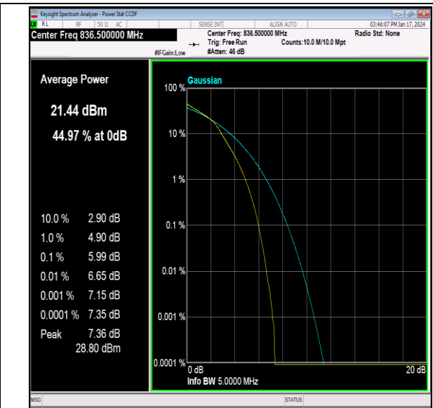
26(824-849)-5MHz-16QAM-26915-25RB#0-PASS
