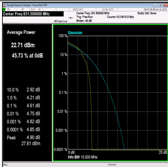
26(824-849)-15MHz-16QAM-26865-1RB#0-PASS
