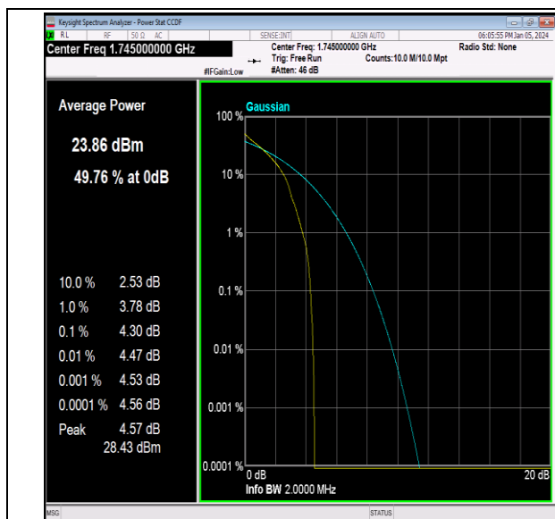
Band66-1.4MHz-QPSK-132322-1RB#0-PASS
