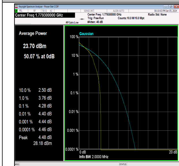
Band66-1.4MHz-QPSK-132665-1RB#0-PASS
