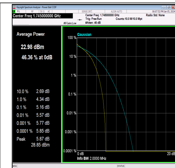
Band66-1.4MHz-QPSK-132322-6RB#0-PASS
