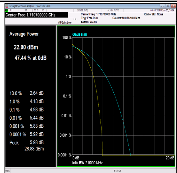
Band66-1.4MHz-QPSK-131979-6RB#0-PASS
