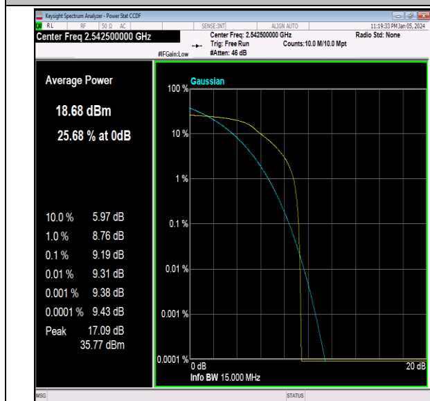
41(2535-2655)-15MHz-QPSK-40115-1RB#0-PASS
