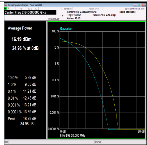
41(2535-2655)-20MHz-64QAM-41140-100RB#0-PASS
