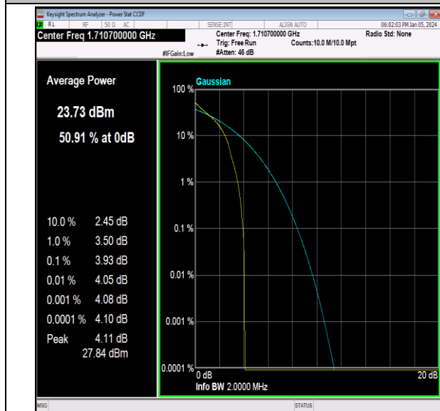
Band66-1.4MHz-QPSK-131979-1RB#0-PASS
