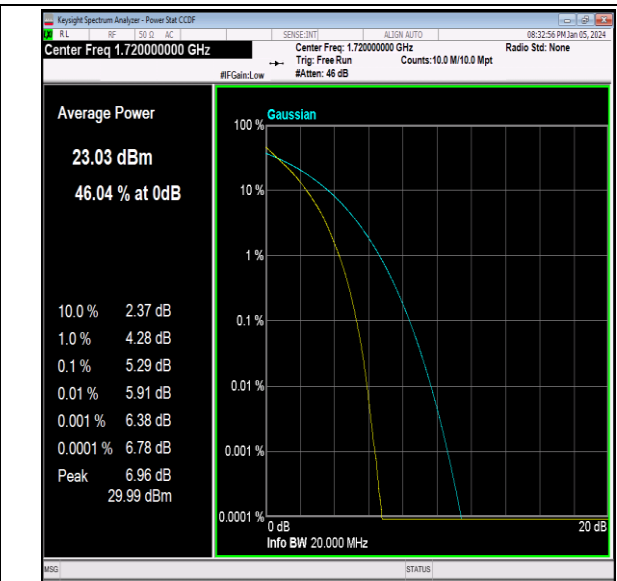
Band66-20MHz-QPSK-132072-100RB#0-PASS
