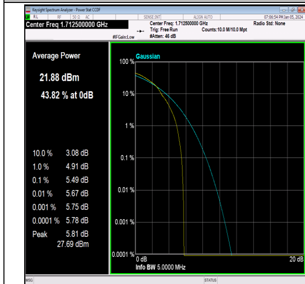
Band66-5MHz-64QAM-131997-1RB#0-PASS
