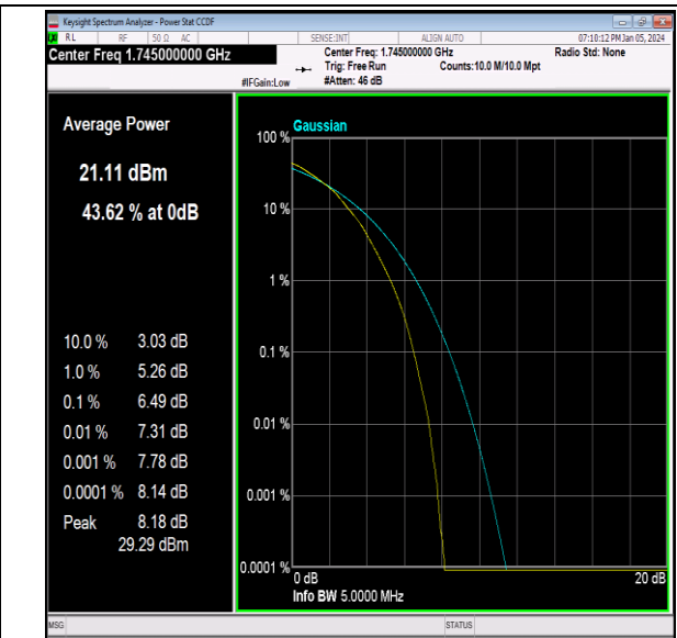
Band66-5MHz-64QAM-132322-25RB#0-PASS
