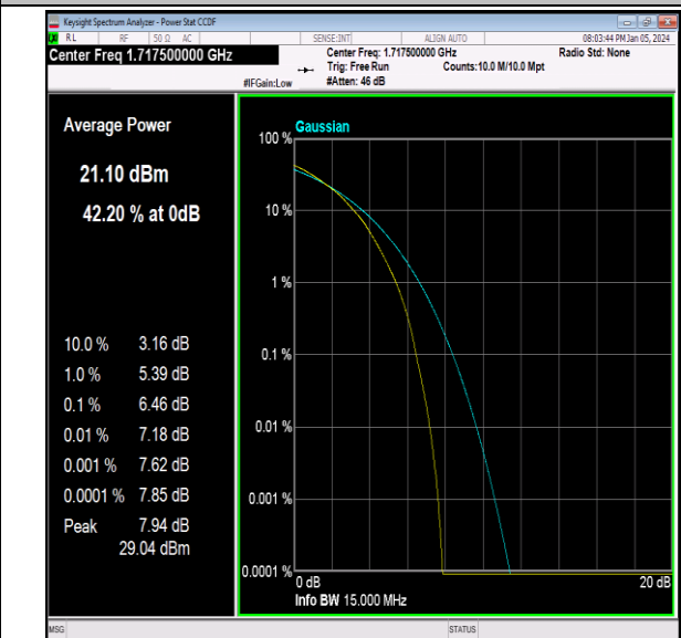
Band66-15MHz-64QAM-132047-75RB#0-PASS
