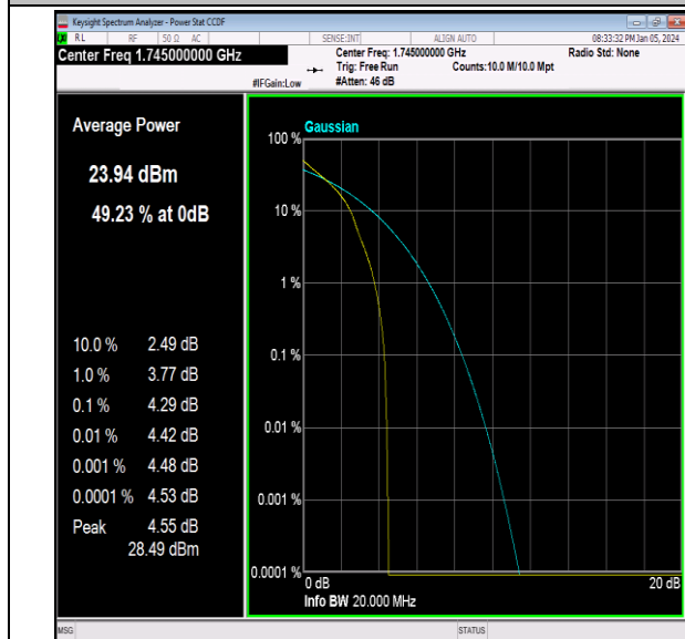
Band66-20MHz-QPSK-132322-1RB#0-PASS
