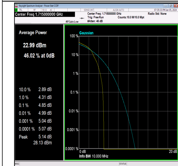
Band66-10MHz-16QAM-132022-1RB#0-PASS
