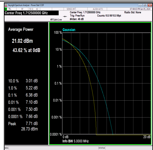
Band66-5MHz-64QAM-131997-25RB#0-PASS
