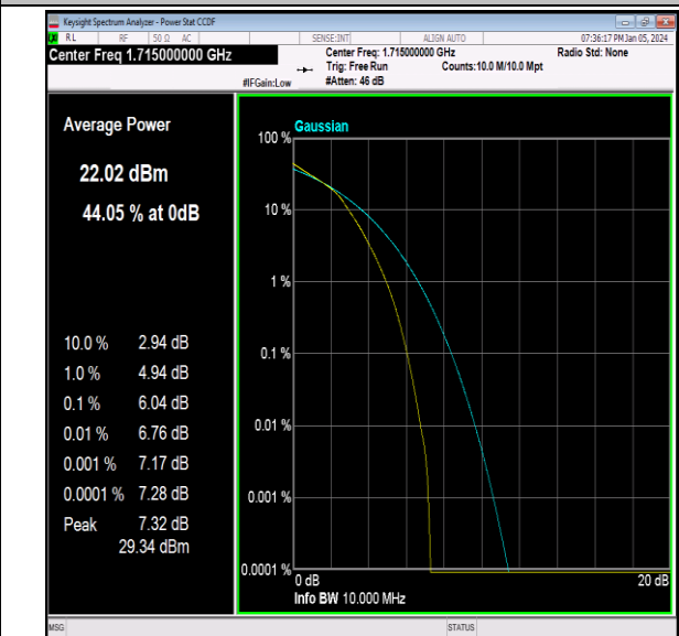
Band66-10MHz-16QAM-132022-50RB#0-PASS
