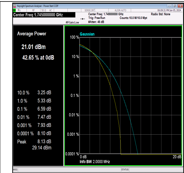
Band66-1.4MHz-64QAM-132322-6RB#0-PASS
