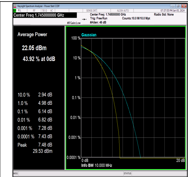
Band66-10MHz-16QAM-132322-50RB#0-PASS
