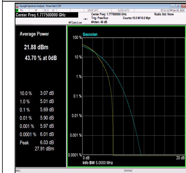
Band66-5MHz-64QAM-132647-1RB#0-PASS
