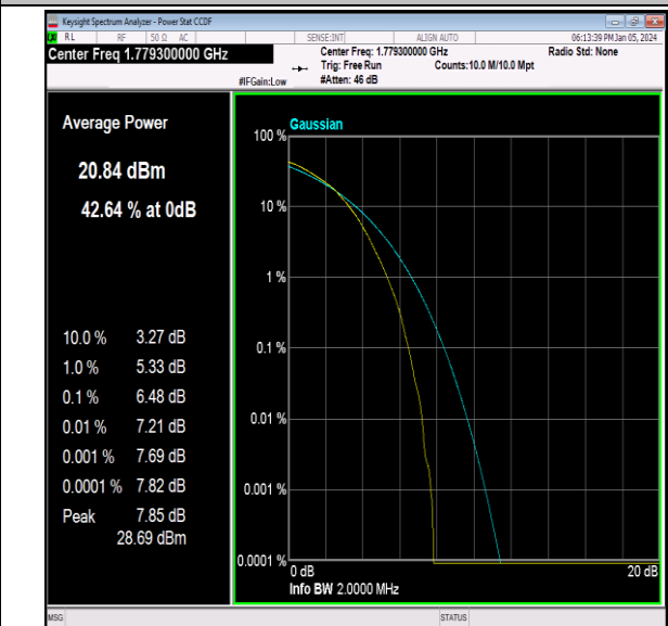
Band66-1.4MHz-64QAM-132665-6RB#0-PASS
