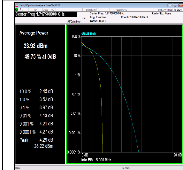
Band66-15MHz-QPSK-132047-1RB#0-PASS
