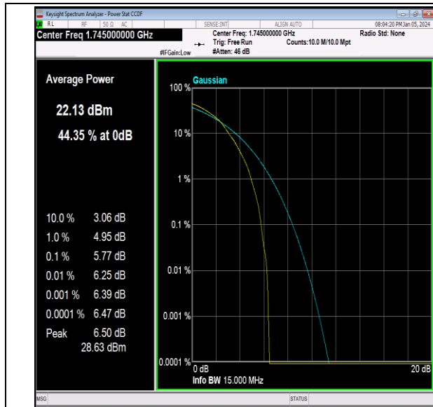
Band66-15MHz-64QAM-132322-1RB#0-PASS
