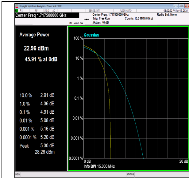
Band66-15MHz-16QAM-132047-1RB#0-PASS
