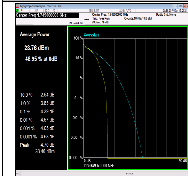
Band66-3MHz-QPSK-132322-1RB#0-PASS
