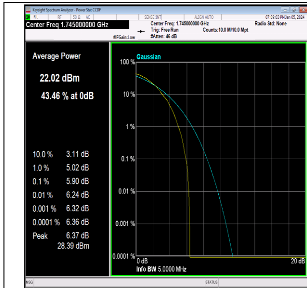
Band66-5MHz-64QAM-132322-1RB#0-PASS
