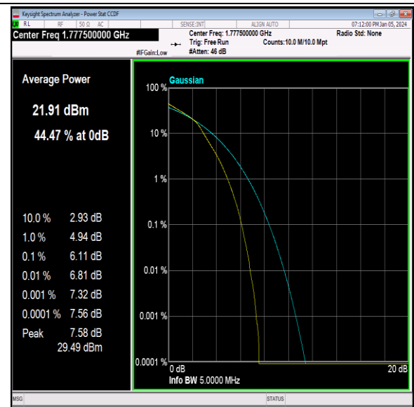
Band66-5MHz-16QAM-132647-25RB#0-PASS
