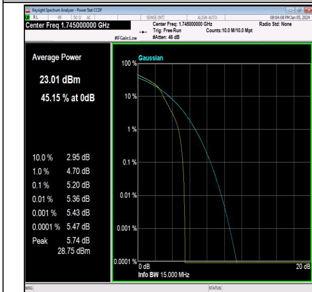
Band66-15MHz-16QAM-132322-1RB#0-PASS
