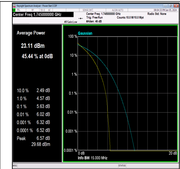
Band66-15MHz-QPSK-132322-75RB#0-PASS
