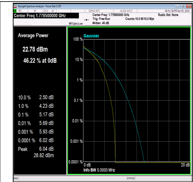
Band66-3MHz-QPSK-132657-15RB#0-PASS
