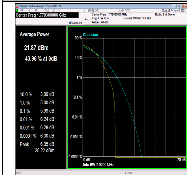
Band66-1.4MHz-64QAM-132665-1RB#0-PASS
