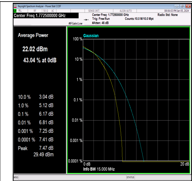
Band66-15MHz-16QAM-132597-75RB#0-PASS
