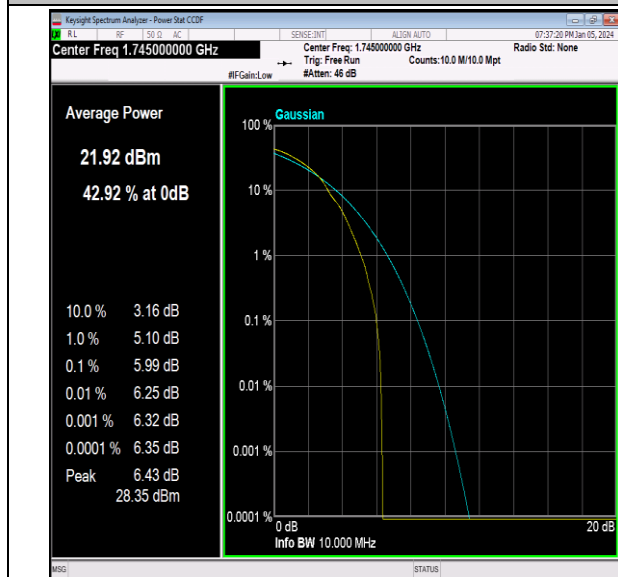
Band66-10MHz-64QAM-132322-1RB#0-PASS
