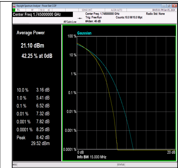
Band66-15MHz-64QAM-132322-75RB#0-PASS
