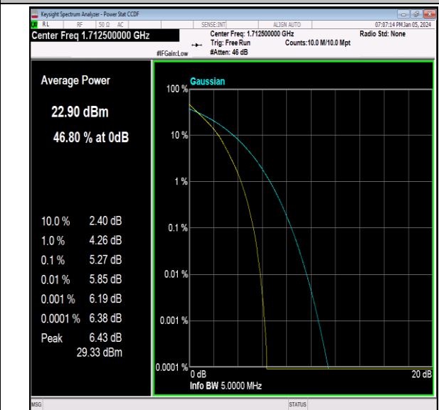
Band66-5MHz-QPSK-131997-25RB#0-PASS
