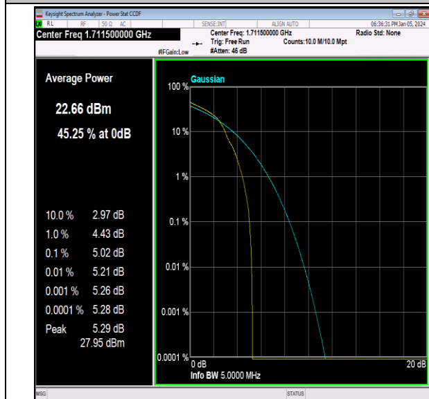
Band66-3MHz-16QAM-131987-1RB#0-PASS
