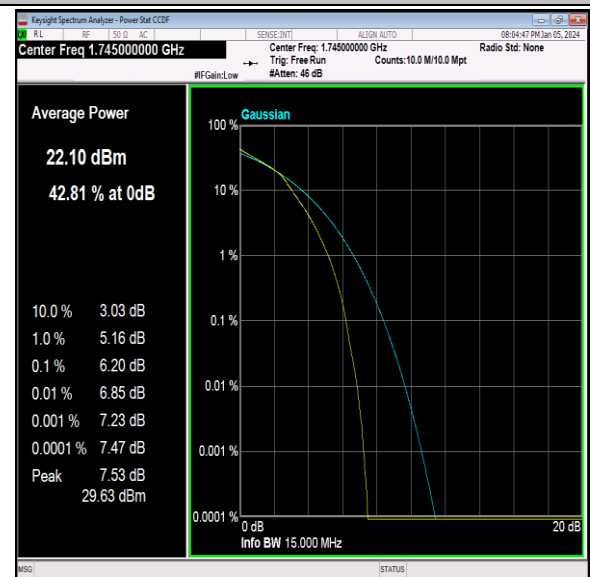
Band66-15MHz-16QAM-132322-75RB#0-PASS
