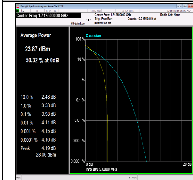
Band66-5MHz-QPSK-131997-1RB#0-PASS
