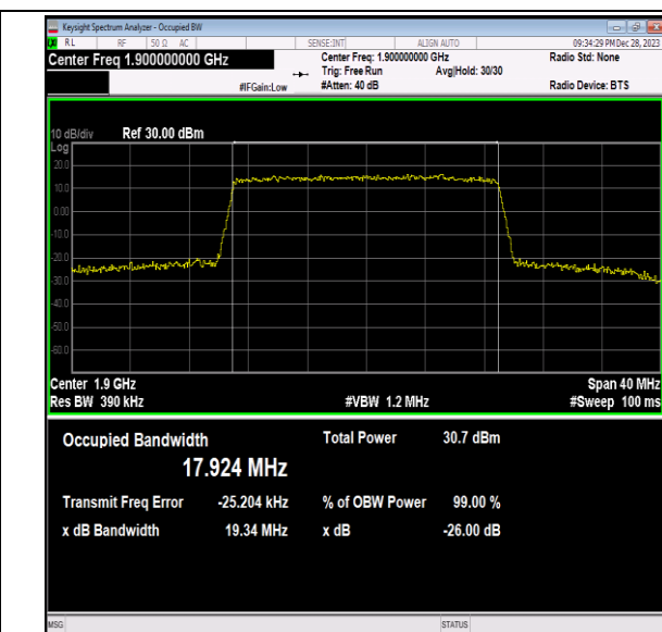
Band2-20MHz-64QAM-19100-100RB#0-PASS
