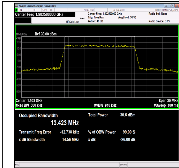
Band2-15MHz-64QAM-19125-75RB#0-PASS
