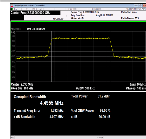
Band7-5MHz-QPSK-21100-25RB#0-PASS
