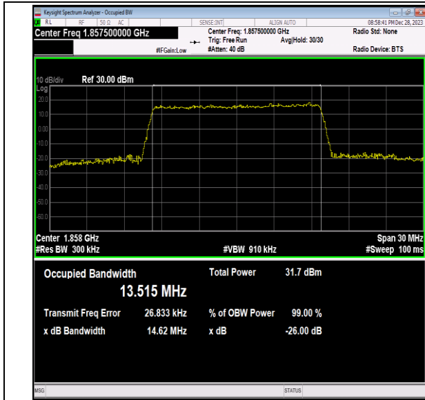
Band2-15MHz-QPSK-18675-75RB#0-PASS
