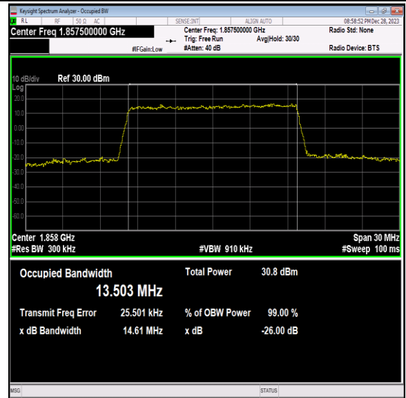
Band2-15MHz-16QAM-18675-75RB#0-PASS
