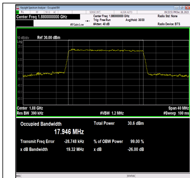
Band2-20MHz-64QAM-18900-100RB#0-PASS
