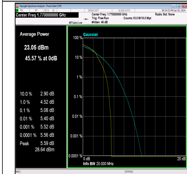
Band66-20MHz-16QAM-132572-1RB#0-PASS
