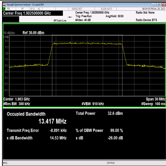
Band2-15MHz-QPSK-19125-75RB#0-PASS
