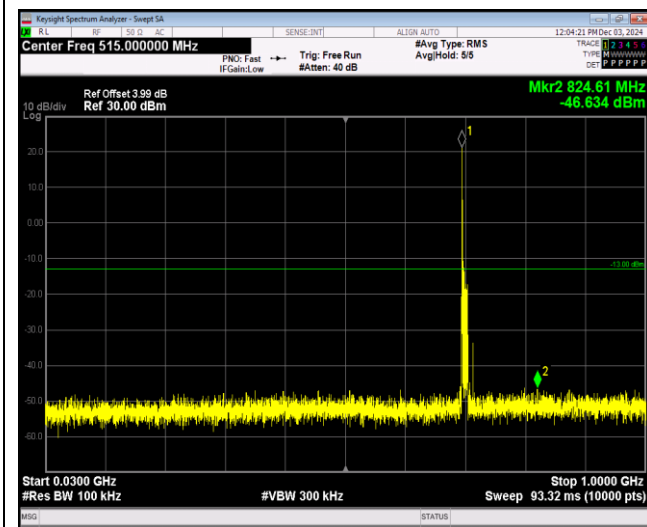
Band12-10MHz-64QAM-23130-1RB#0-Range1:30~1000MHz
