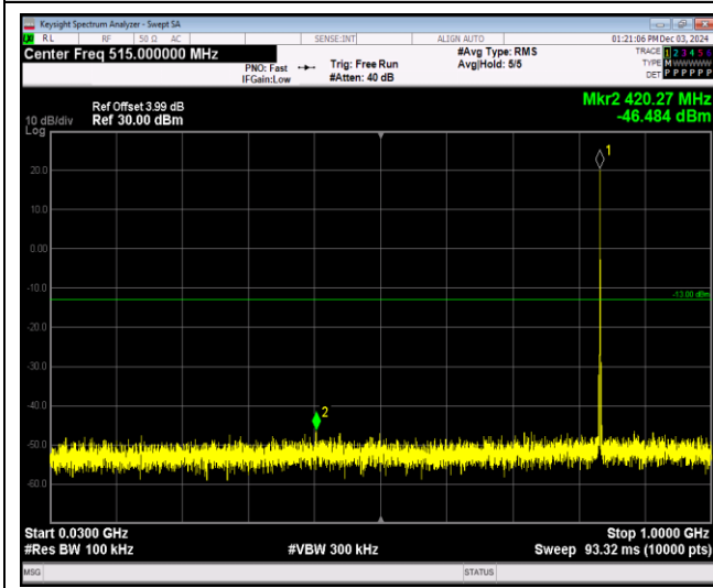
Band26-1.4MHz-64QAM-26915-1RB#0-Range1:30~1000MHz
