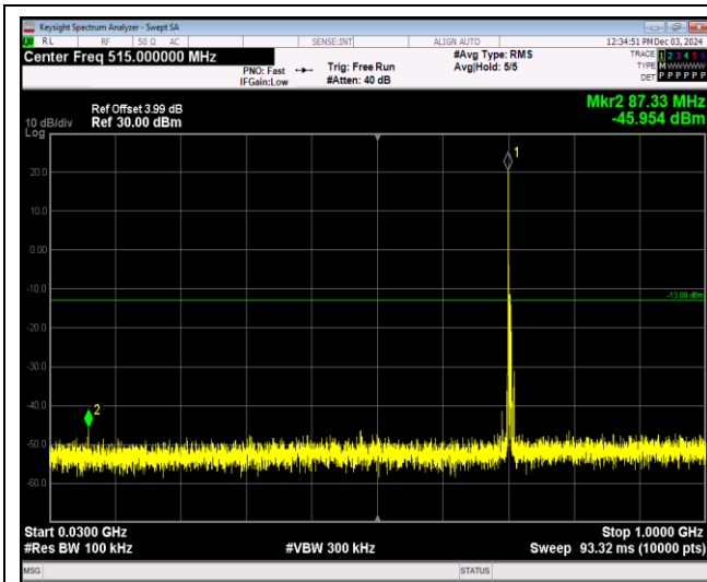
Band17-5MHz-64QAM-23825-1RB#0-Range1:30~1000MHz
