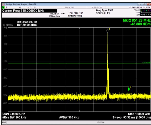
Band17-10MHz-QPSK-23800-1RB#0-Range1:30~1000MHz
