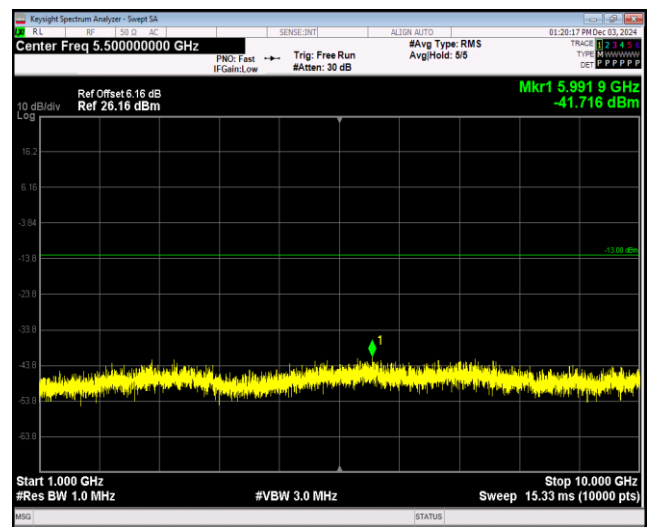
Band26-1.4MHz-64QAM-26915-1RB#0-Range2:1000~10000MHz
