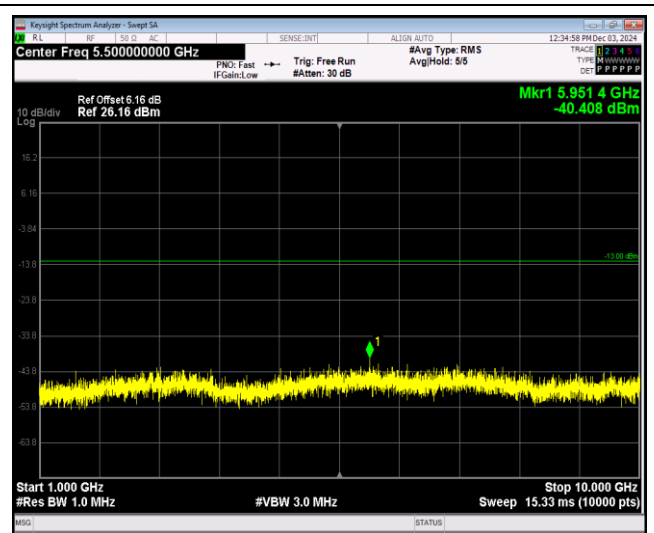
Band17-5MHz-64QAM-23825-1RB#0-Range2:1000~10000MHz
