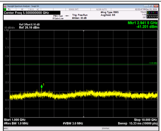
Band26-1.4MHz-64QAM-26797-1RB#0-Range2:1000~10000MHz
