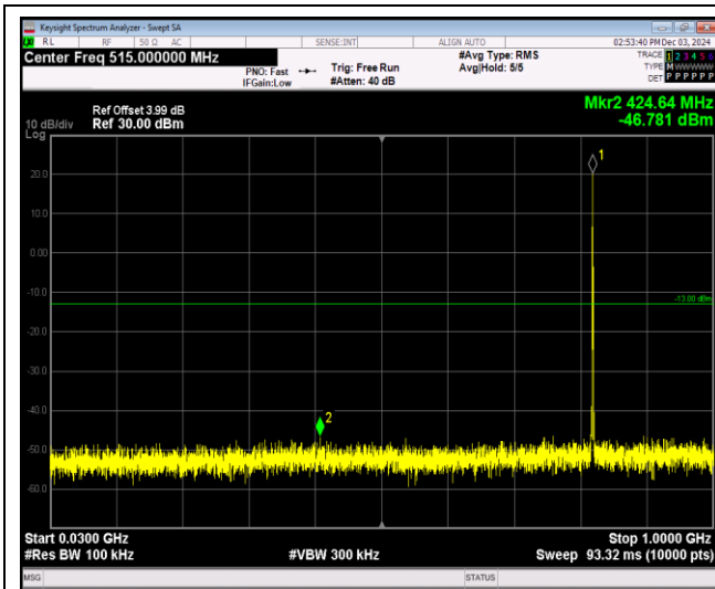
Band26-1.4MHz-64QAM-26797-1RB#0-Range1:30~1000MHz
