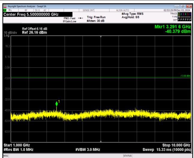
Band26-1.4MHz-16QAM-26797-1RB#0-Range2:1000~10000MHz
