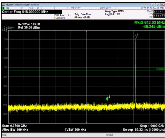
Band26-1.4MHz-16QAM-26783-1RB#0-Range1:30~1000MHz
