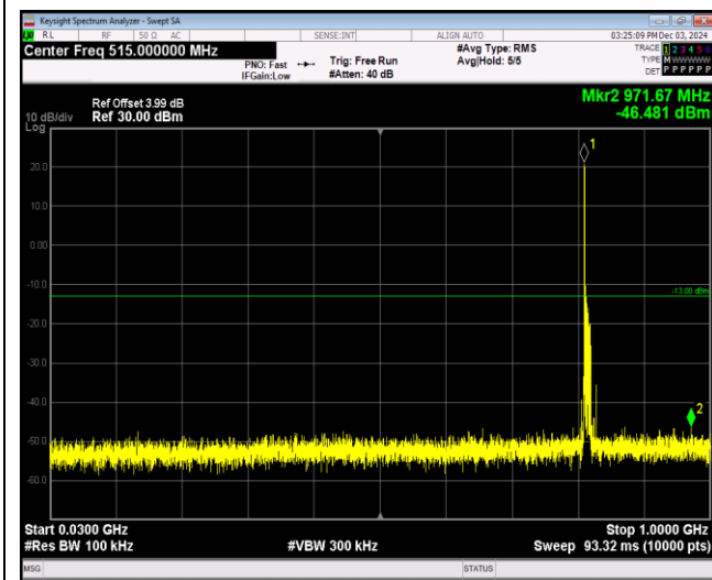
Band26-15MHz-QPSK-26865-1RB#0-Range1:30~-1000MHz
