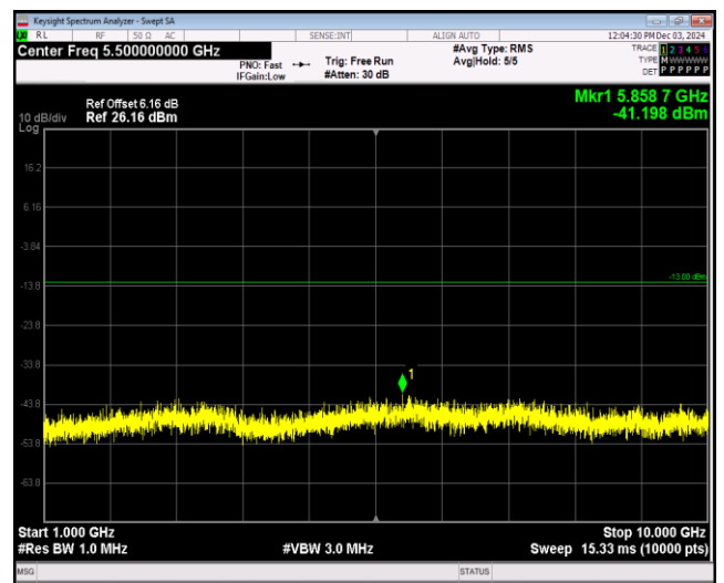
Band12-10MHz-64QAM-23130-1RB#0-Range2:1000~10000MHz
