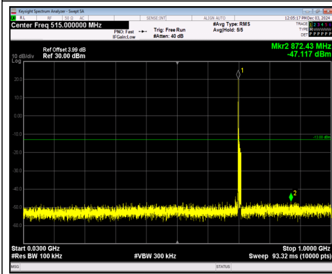
Band12-10MHz-64QAM-23130-1RB#0-Range1:30~1000MHz
