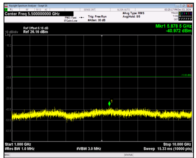
Band26-15MHz-QPSK-26865-1RB#0-Range2:1000~10000MHz
