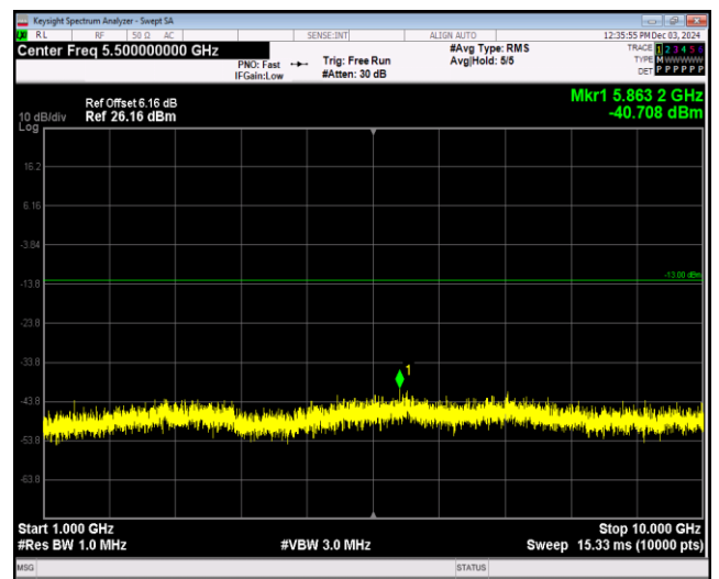
Band17-10MHz-QPSK-23780-1RB#0-Range2:1000~10000MHz
