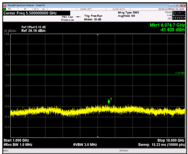
Band26-1.4MHz-QPSK-26797-1RB#0-Range2:1000 ~10000MHz
