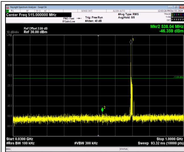
Band12-10MHz-64QAM-23095-1RB#0-Range1:30~1000MHz
