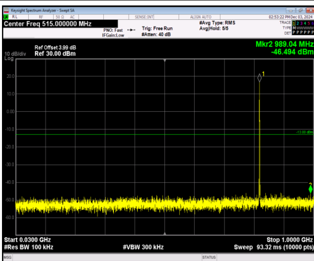
Band26-1.4MHz-16QAM-26797-1RB#0-Range1:30~1000MHz
