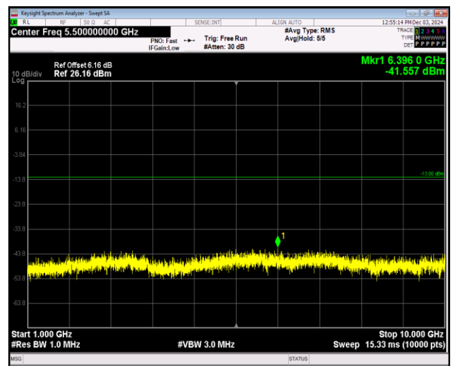
Band17-10MHz-16QAM-23800-1RB#0-Range2:1000~10000MHz
