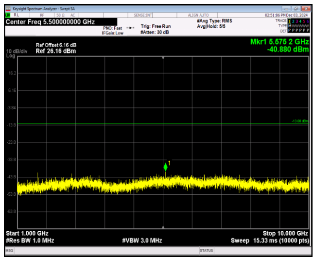
Band26-1.4MHz-64QAM-26740-1RB#0-Range2:1000~10000MHz
