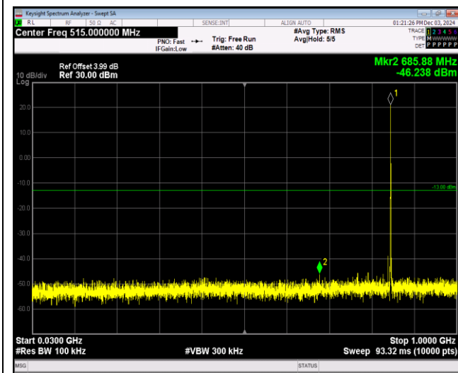
Band26-1.4MHz-16QAM-26697-1RB#0-Range1:30~1000MHz
