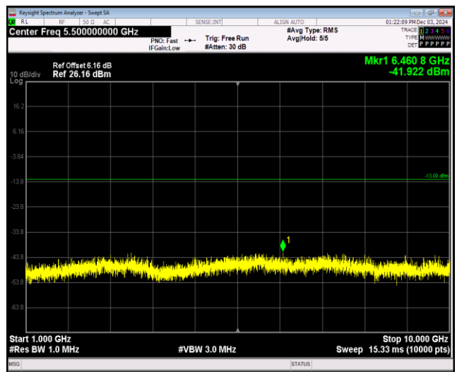
Band26-10MHz-QPSK-26740-1RB#0-Range2:1000~10000MHz
