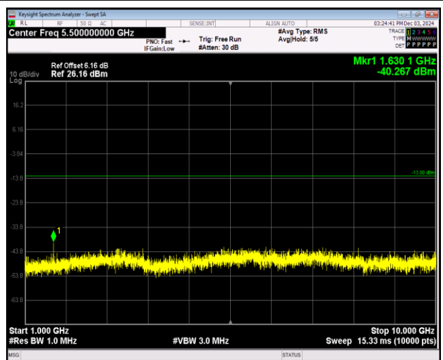
Band26-10MHz-16QAM-26740-1RB#0-Range2:1000~10000MHz
