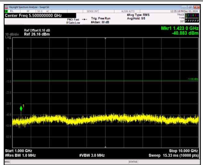
Band17-5MHz-16QAM-23755-1RB#0-Range2:1000~10000MHz
