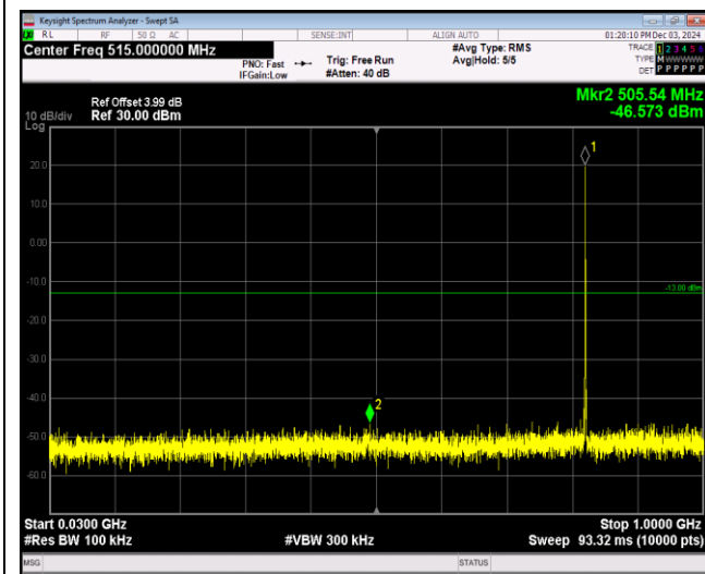
Band26-1.4MHz-64QAM-26915-1RB#0-Range1:30~1000MHz
