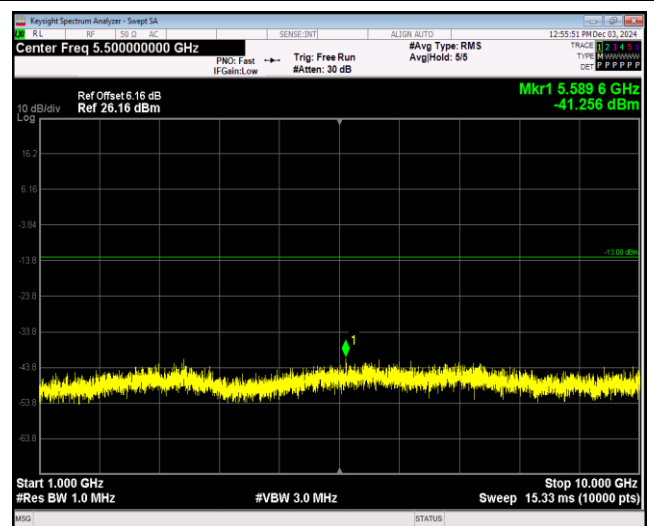
Band17-10MHz-16QAM-23780-1RB#0-Range2:1000~10000MHz
