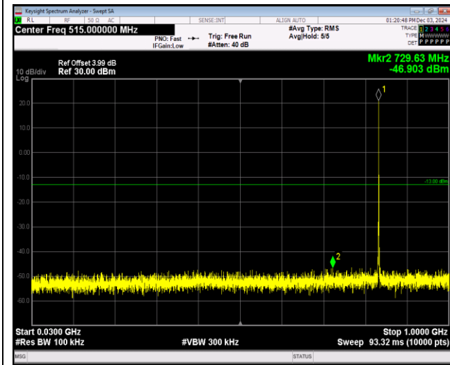
Band26-1.4MHz-16QAM-27033-1RB#0-Range1:30~1000MHz
