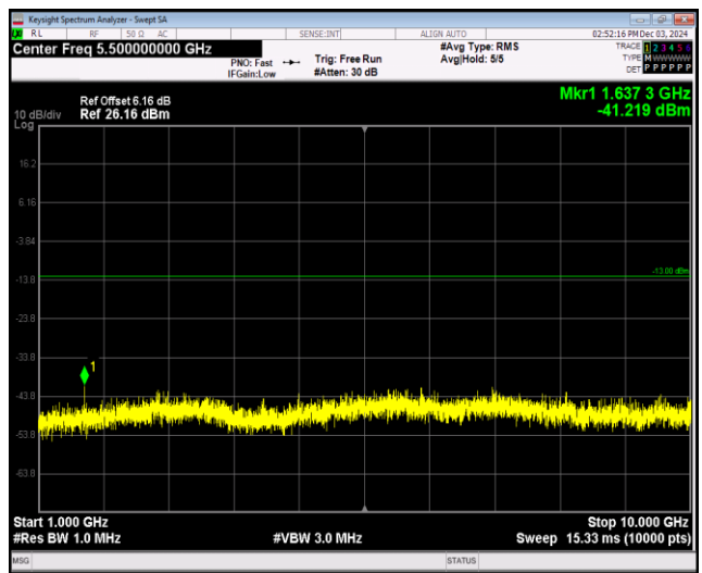
Band26-1.4MHz-16QAM-26783-1RB#0-Range2:1000~10000MHz
