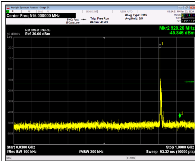
Band26-10MHz-64QAM-26740-1RB#0-Range1:30~-1000MHz
