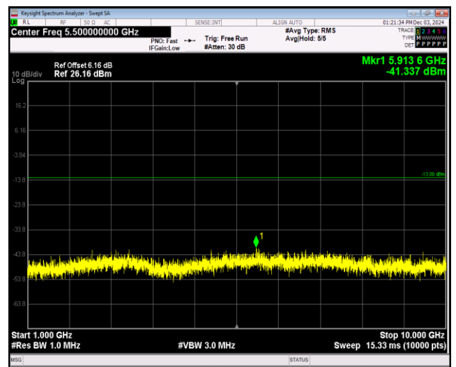
Band26-1.4MHz-16QAM-26697-1RB#0-Range2:1000~10000MHz
