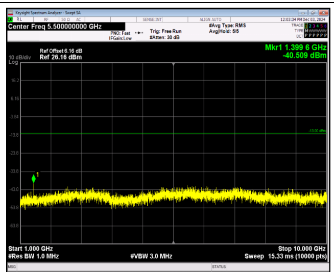
Band12-10MHz-64QAM-23095-1RB#0-Range2:1000~10000MHz
