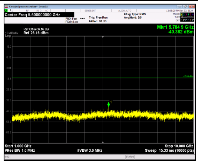
Band12-10MHz-64QAM-23130-1RB#0-Range2:1000~10000MHz
