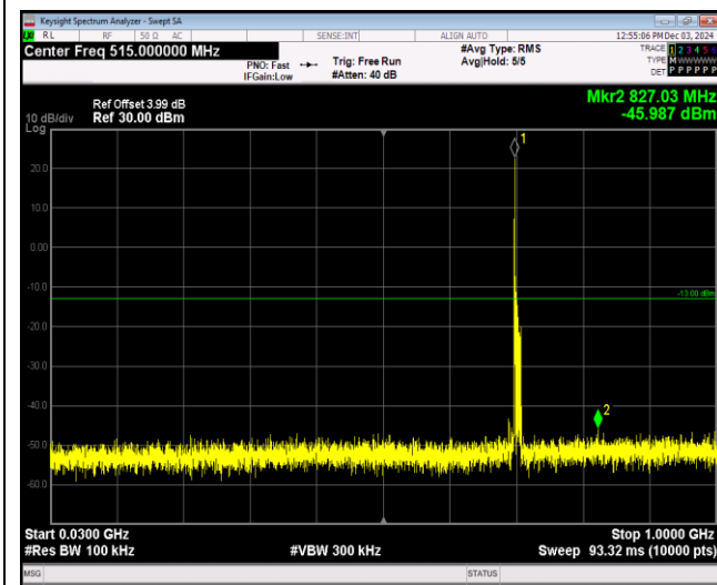
Band17-10MHz-16QAM-23800-1RB#0-Range1:30~1000MHz
