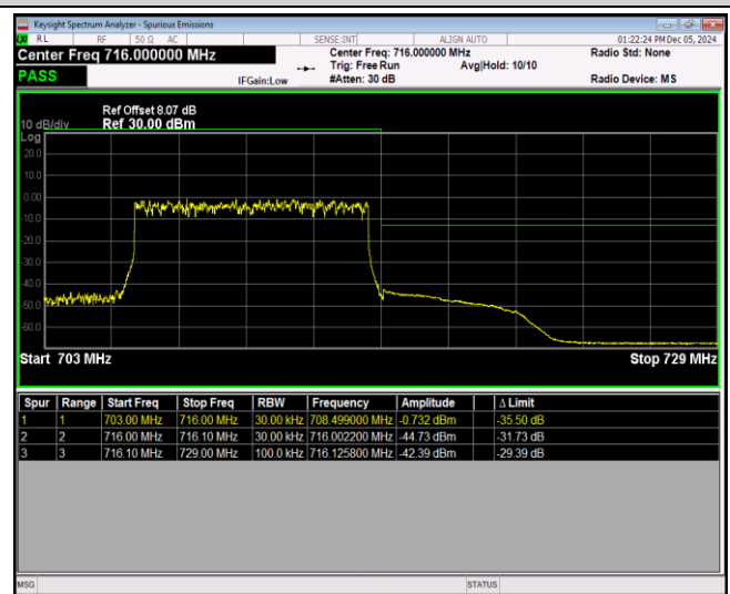
Band17-10MHz-64QAM-23780-1RB#49
