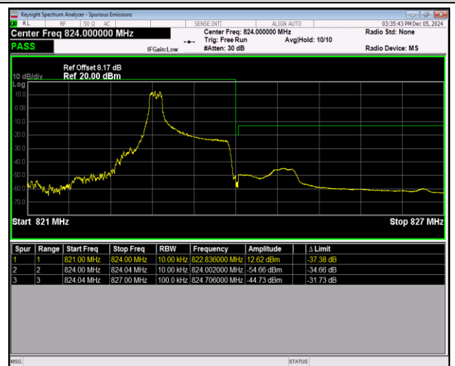
Band26-1.4MHz-QPSK-26783-6RB#0
