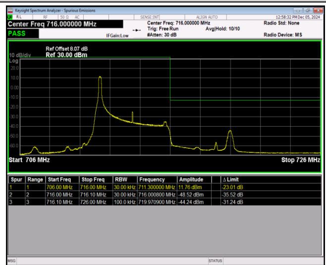
Band17-5MHz-64QAM-23825-25RB#0
