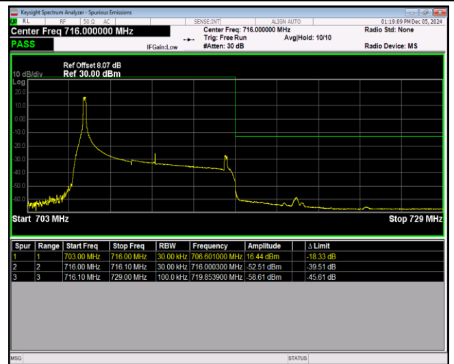
Band17-10MHz-QPSK-23800-50RB#0
