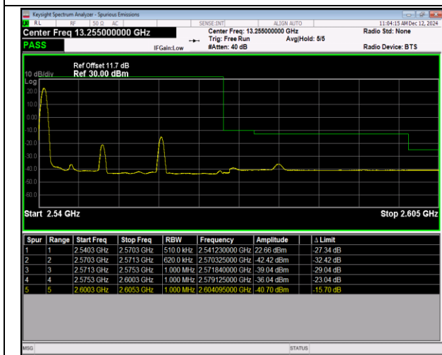
7-7-10MHz-20MHz-16QAM@16QAM-16QAM@16QAM-21206-21350-1RB#0@50RB#0-0RB#0@100RB#0-PASS
