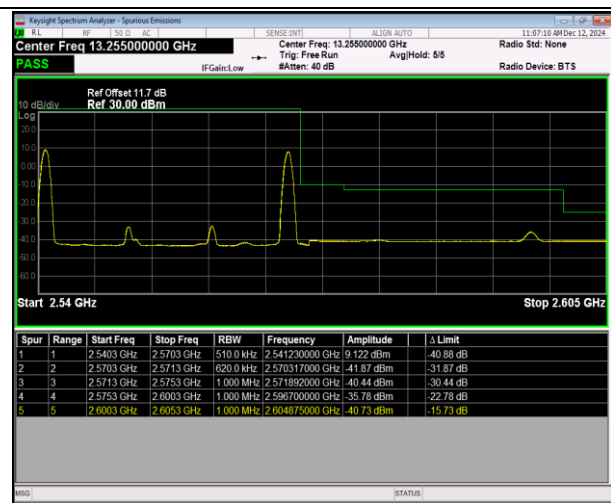
7-7-10MHz-20MHz-16QAM@16QAM-16QAM@16QAM-21206-21350-1RB#0@50RB#0-1RB#99@100RB#0-PASS
