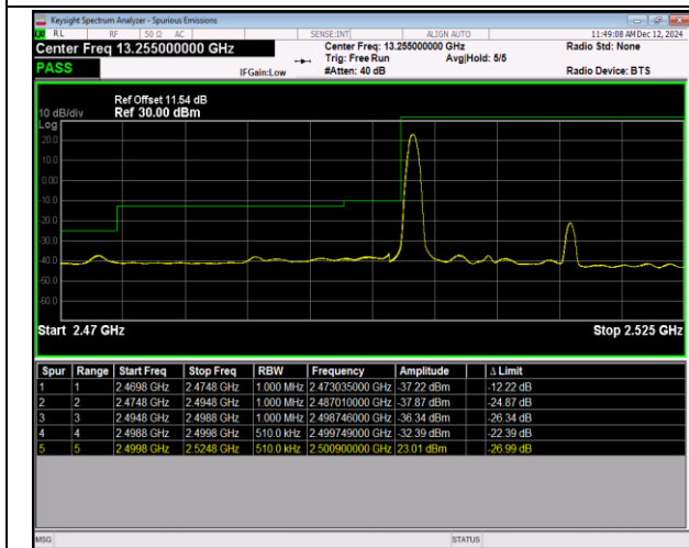
7-7-15MHz-10MHz-16QAM@16QAM-16QAM@16QAM-20825-20945-1RB#0@75RB#0-0RB#0@50RB#0-PASS
