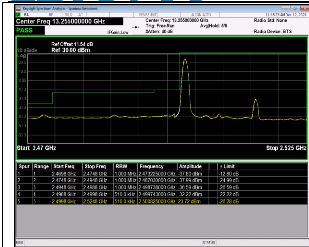
7-7-15MHz-10MHz-QPSK@QPSK-QPSK@QPSK-20825-20945-1RB#0@75RB#0-0RB#0@50RB#0-PASS
