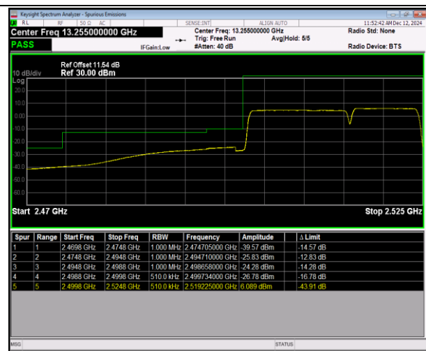
7-7-15MHz-10MHz-QPSK@QPSK-QPSK@QPSK-20825-20945-75RB#0@75RB#0-50RB#0@50RB#0-PASS
