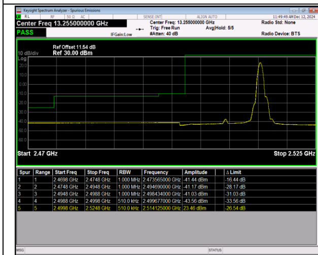
7-7-15MHz-10MHz-QPSK@QPSK-QPSK@QPSK-20825-20945-1RB#74@75RB#0-0RB#0@50RB#0-PASS
