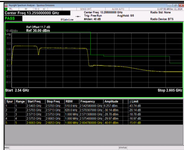
7-7-10MHz-20MHz-QPSK@QPSK-QPSK@QPSK-21206-21350-50RB#0@50RB#0-100RB#0@100RB#0-PASS
