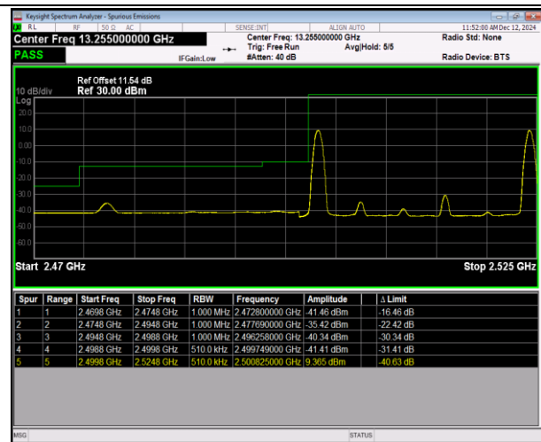
7-7-15MHz-10MHz-16QAM@16QAM-16QAM@16QAM-20825-20945-1RB#0@75RB#0-1RB#49@50RB#0-PASS
