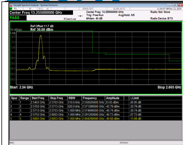
7-7-10MHz-20MHz-QPSK@QPSK-QPSK@QPSK-21206-21350-1RB#49@50RB#0-0RB#0@100RB#0-PASS
