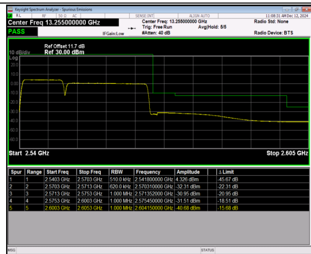
7-7-10MHz-20MHz-16QAM@16QAM-16QAM@16QAM-21206-21350-50RB#0@50RB#0-100RB#0@100RB#0-PASS
