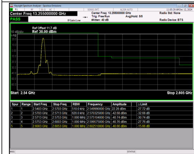
7-7-10MHz-20MHz-16QAM@16QAM-16QAM@16QAM-21206-21350-1RB#49@50RB#0-0RB#0@100RB#0-PASS
