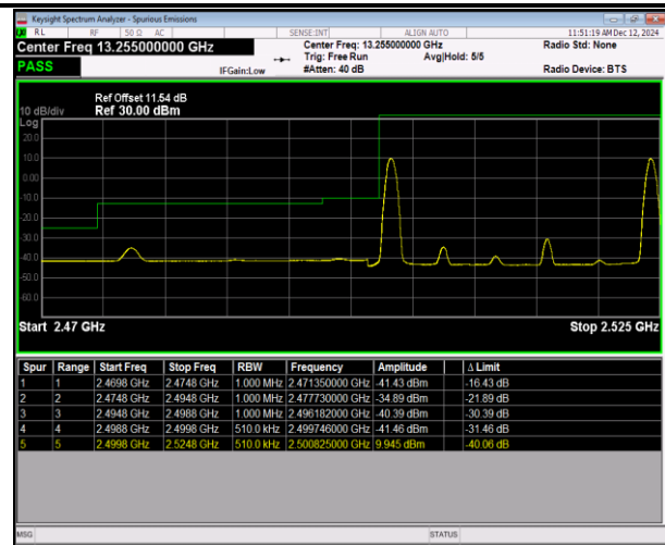
7-7-15MHz-10MHz-QPSK@QPSK-QPSK@QPSK-20825-20945-1RB#0@75RB#0-1RB#49@50RB#0-PASS
