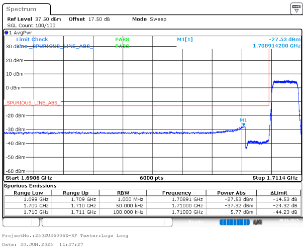
1.4MHz_Low_QPSK_6@0
