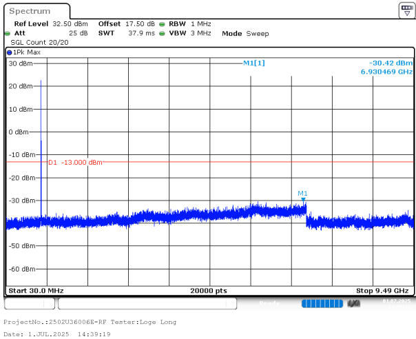
15MHz_Middle_QPSK_1@0(30MHz~9.49GHz)
