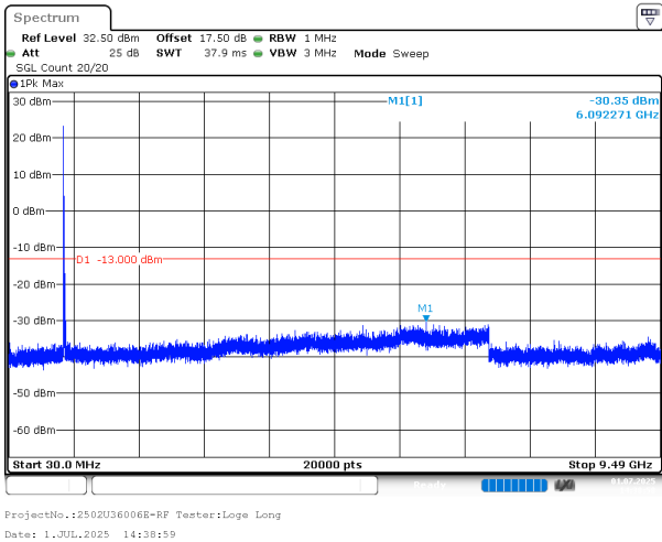
15MHz_High_QPSK_1@0(30MHz~9.49GHz)
