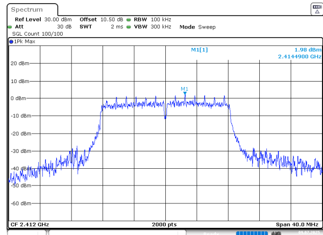
802.11g_2412MHz
