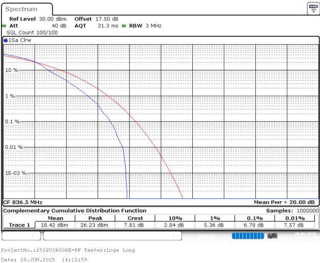
5MHz_Middle_QPSK_1@0
