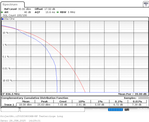
5MHz_Middle_16QAM_1@0
