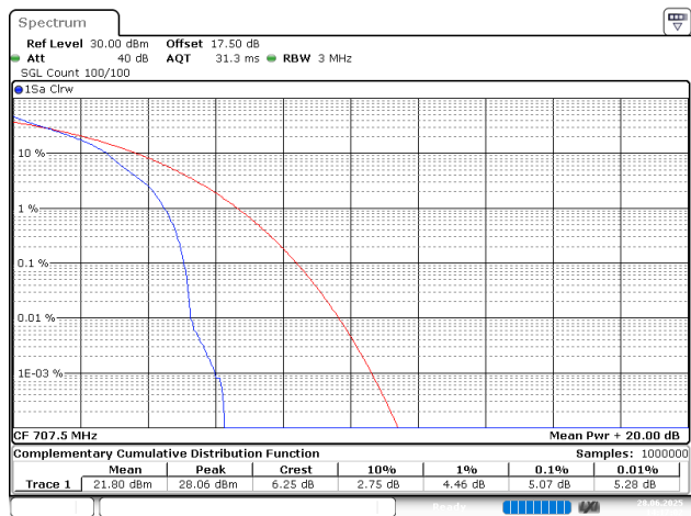
3MHz_Middle_QPSK_1@0
