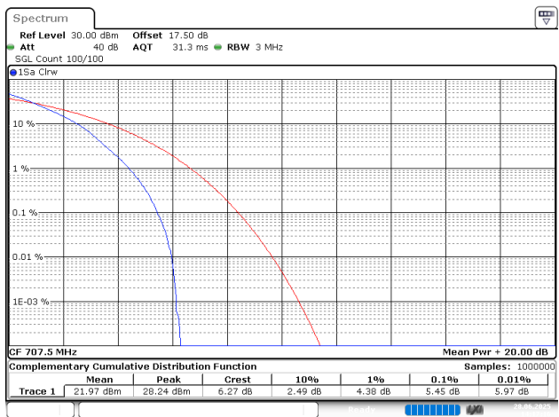
3MHz_Middle_QPSK_15@0
