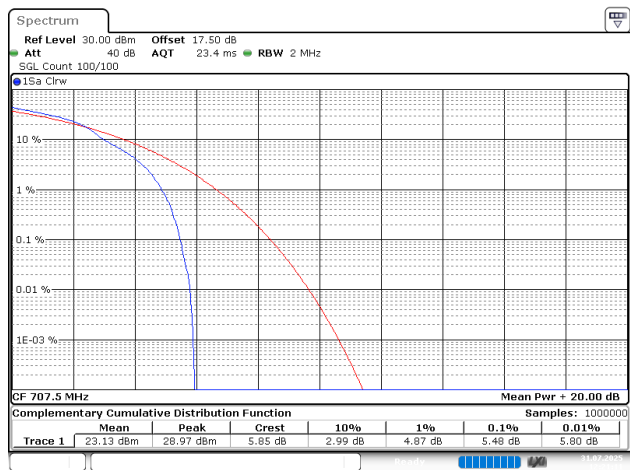
1.4MHz_Middle_16QAM_1@0
