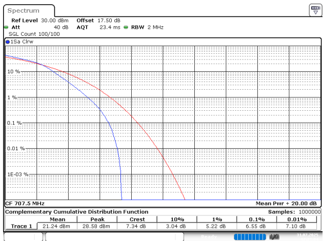
1.4MHz_Middle_16QAM_6@0
