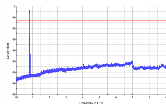
CDMA 1XRTT BC0 CH1013 30MHz~9GHz
