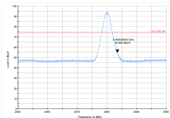
3DH5-Channel 78: Peak
