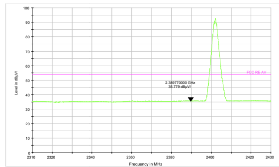
DH5-Channel 0: Average
