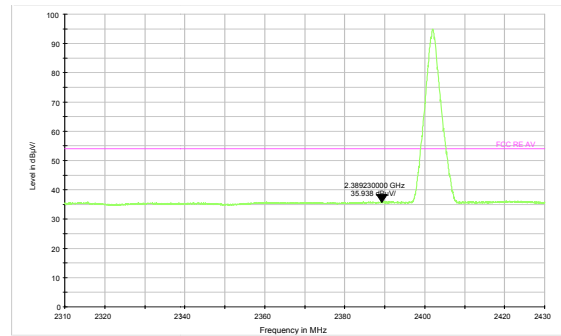
3DH5-Channel 0: Average
