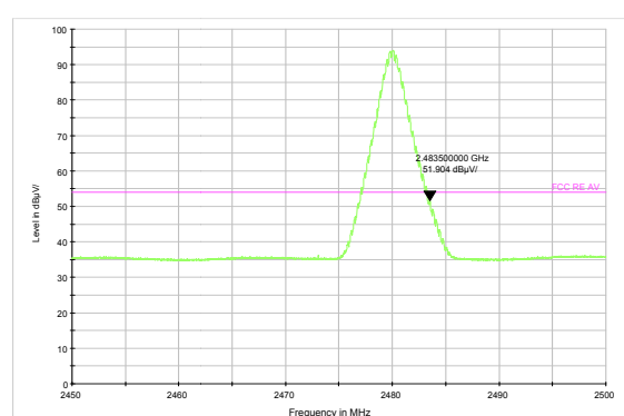
3DH5-Channel 78: Average
