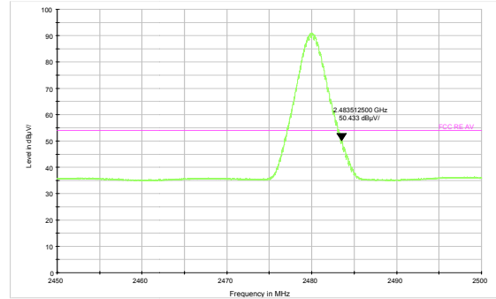
DH5-Channel 78: Average
