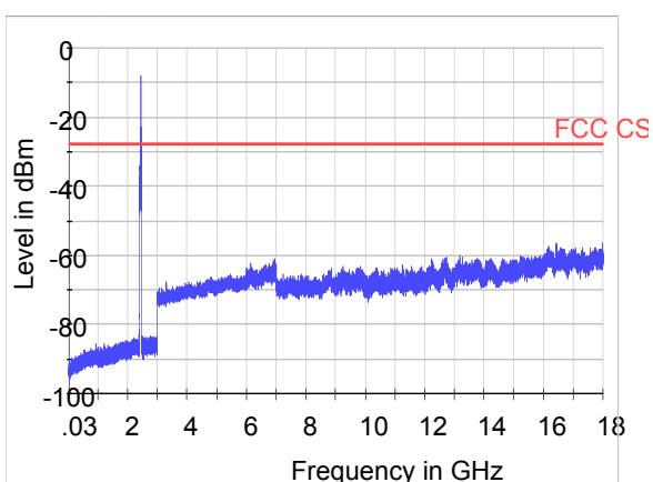
GFSK-CH39 30MHz to 18GHz
