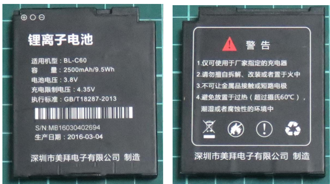
b: Battery
