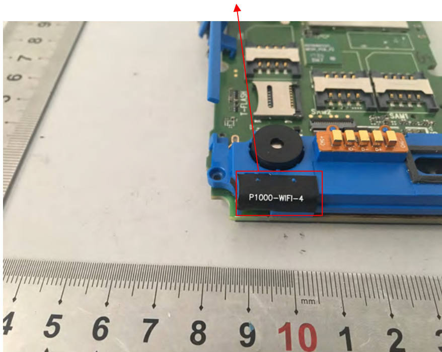
EUT – BT&2.4G WIFI Antenna View
