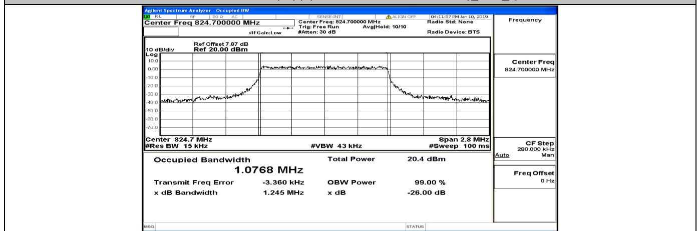
EBW &amp; OBW Test Graph(s) (Channel Bandwidth: 1.4 MHz)_LCH_QPSK
