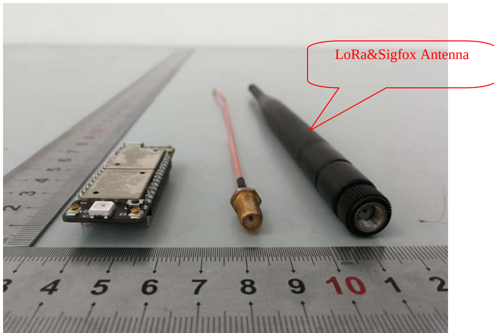
EUT – Antenna Port View
