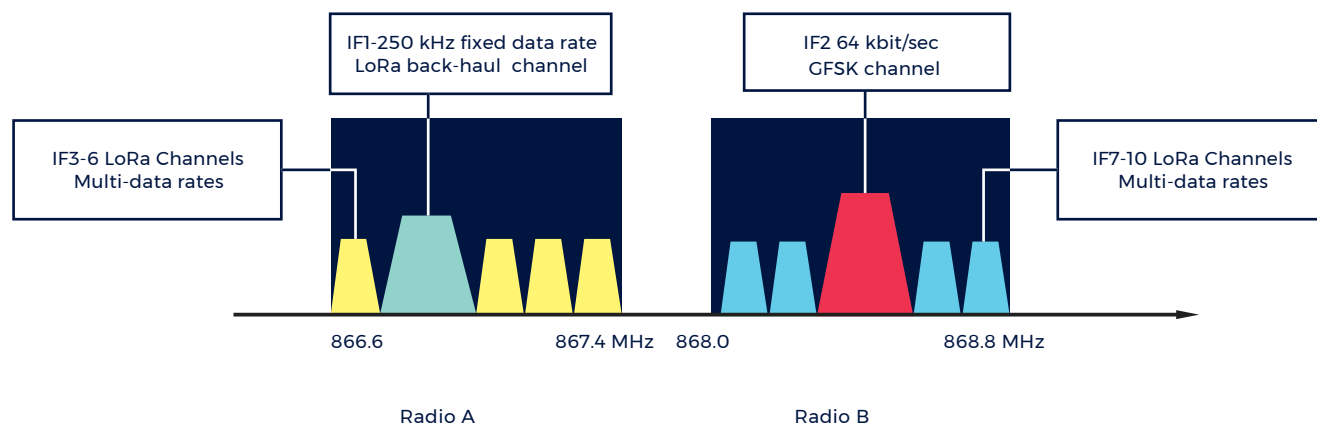
Figure 10 - Radio Spectrum
