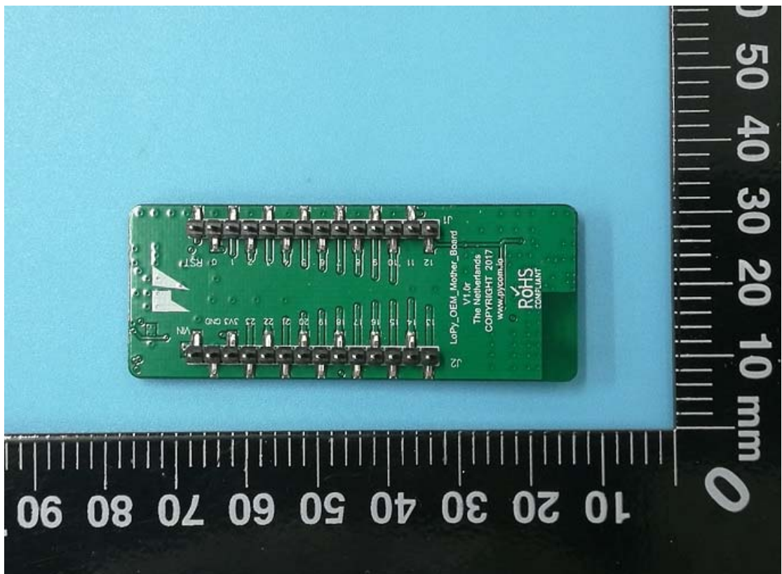
2. EUT rear view
