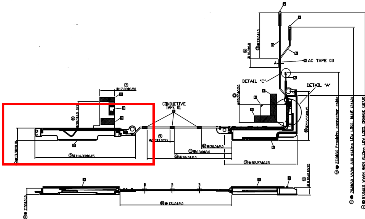
Aux Antenna Dimensioned Drawing:
