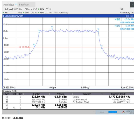
1-N5--15-5-L-4-DFT-64QAM-Outer_Full-25@0-Ant0- 4.478-5.100-≤5-PASS
