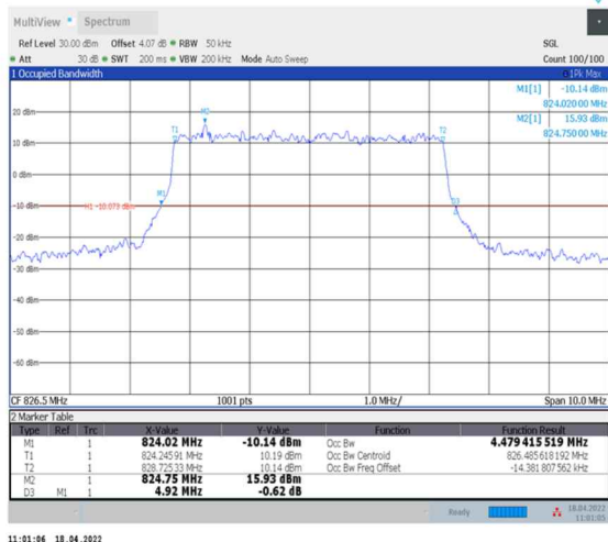
1-N5--15-5-L-1-DFT-QPSK-Outer_Full-25@0-Ant0- 4.479-4.920-≤5-PASS
