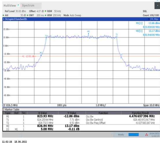
1-N5--15-5-L-3-DFT-16QAM-Outer_Full-25@0-Ant0- 4.477-5.080-≤5-PASS
