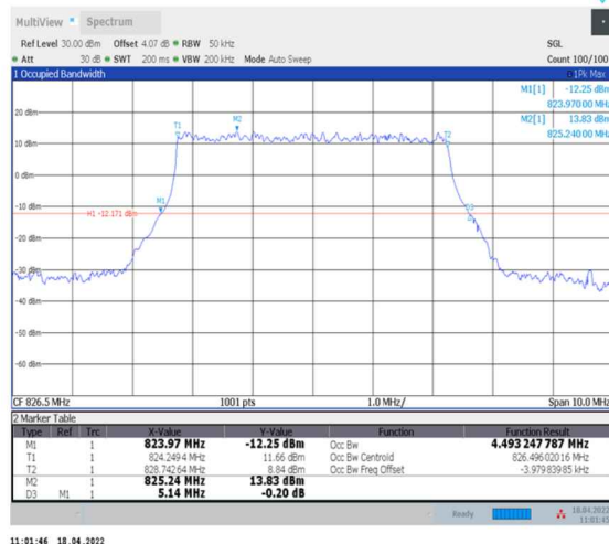
1-N5--15-5-L-2-DFT-PI2BPSK-Outer_Full-25@0-Ant0- 4.493-5.140-≤5-PASS
