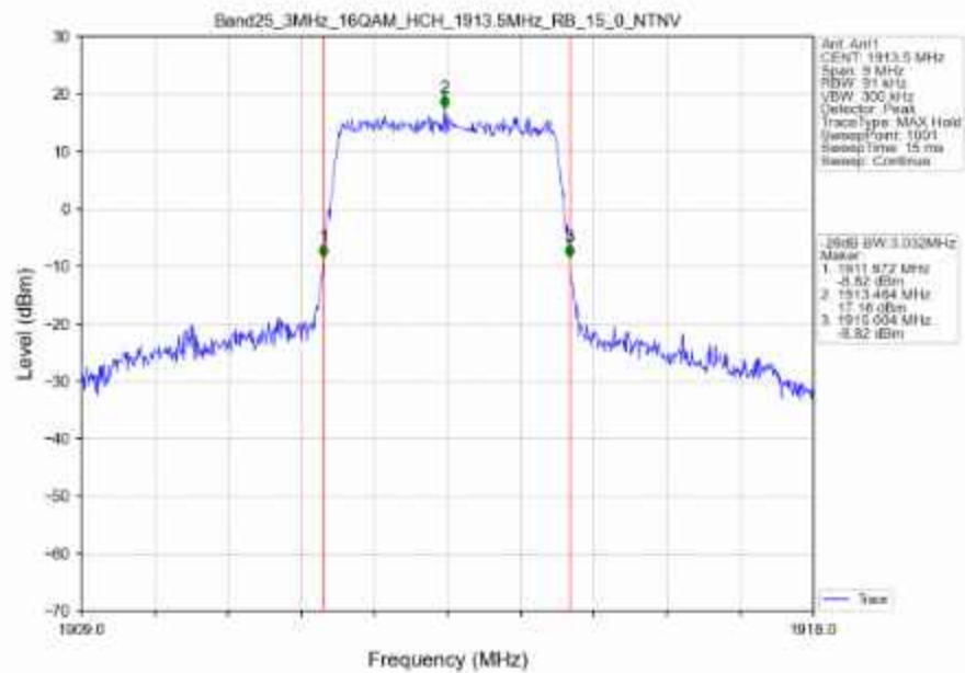
Band25_3MHz_16QAM_HCH_1913.5MHz_RB_15_0_NTNV
