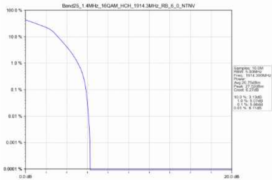
Band25_1.4MHz_16QAM_HCH_1914.3MHz_RB_6_0_NTNV
