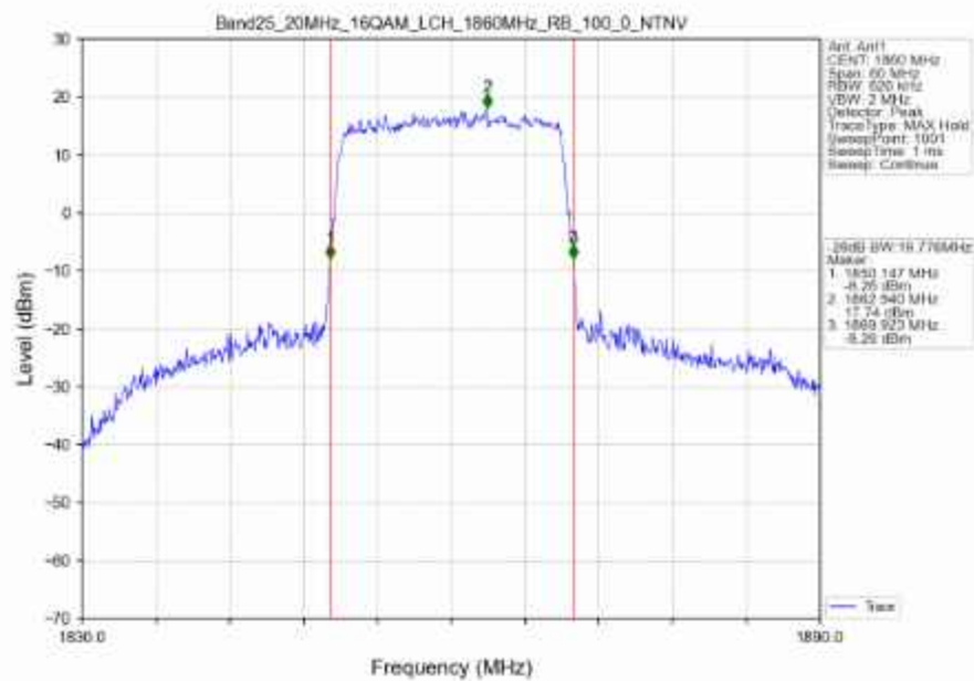
Band25_20MHz_16QAM_LCH_1860MHz_RB_100_0_NTNV
