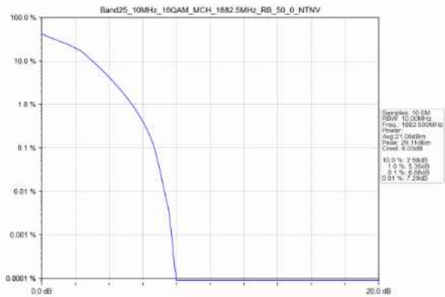
Band25_10MHz_16QAM_MCH_1882.5MHz_RB_50_0_NTNV
