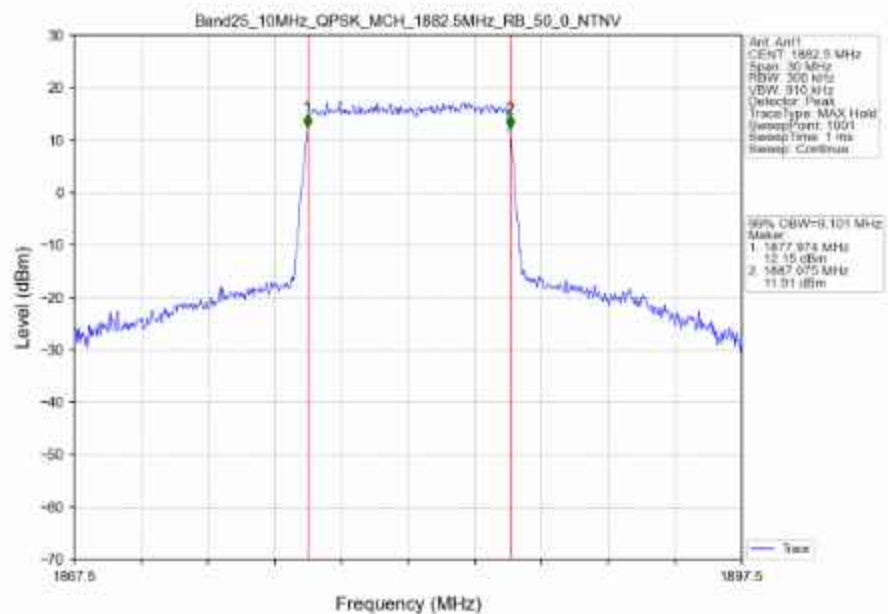
Band25_10MHz_QPSK_MCH_1882.5MHz_RB_50_0_NTNV
