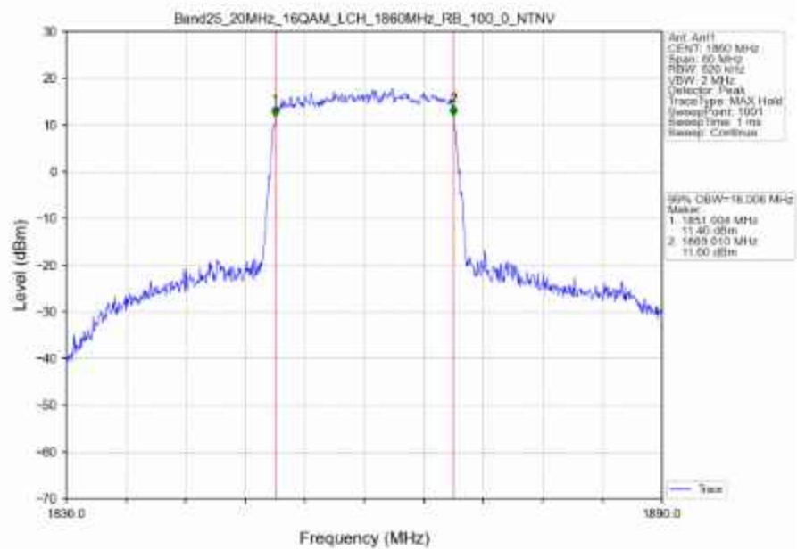
Band25_20MHz_16QAM_LCH_1860MHz_RB_100_0_NTNV
