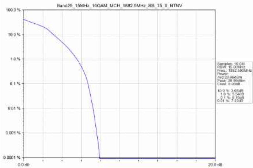
Band25_15MHz_16QAM_MCH_1882.5MHz_RB_75_0_NTNV
