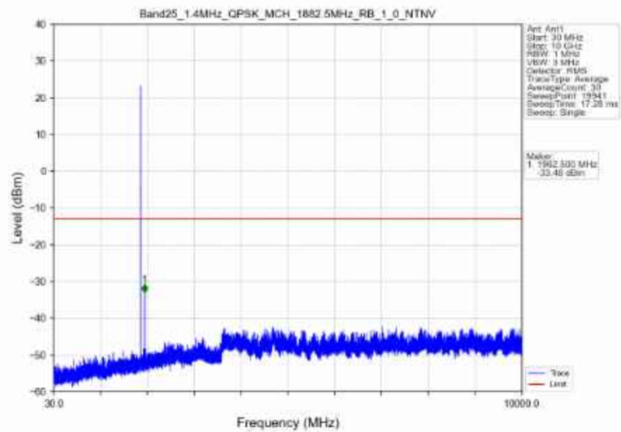
Band25_1.4MHz_QPSK_MCH_1882.5MHz_RB_1_0_NTNV
