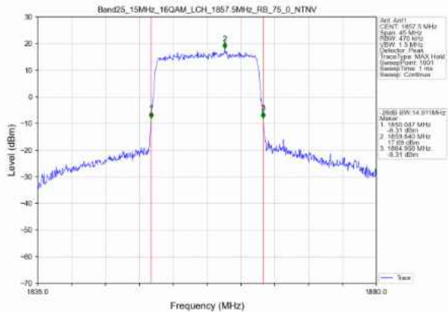
Band25_15MHz_16QAM_LCH_1857.5MHz_RB_75_0_NTNV
