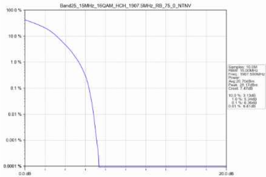
Band25_15MHz_16QAM_HCH_1907.5MHz_RB_75_0_NTNV
