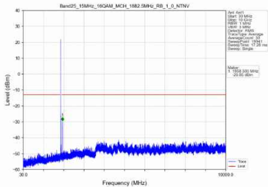
Band25_15MHz_16QAM_MCH_1882.5MHz_RB_1_0_NTNV
