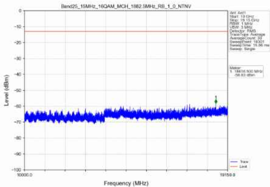
Band25_15MHz_16QAM_MCH_1882.5MHz_RB_1_0_NTNV
