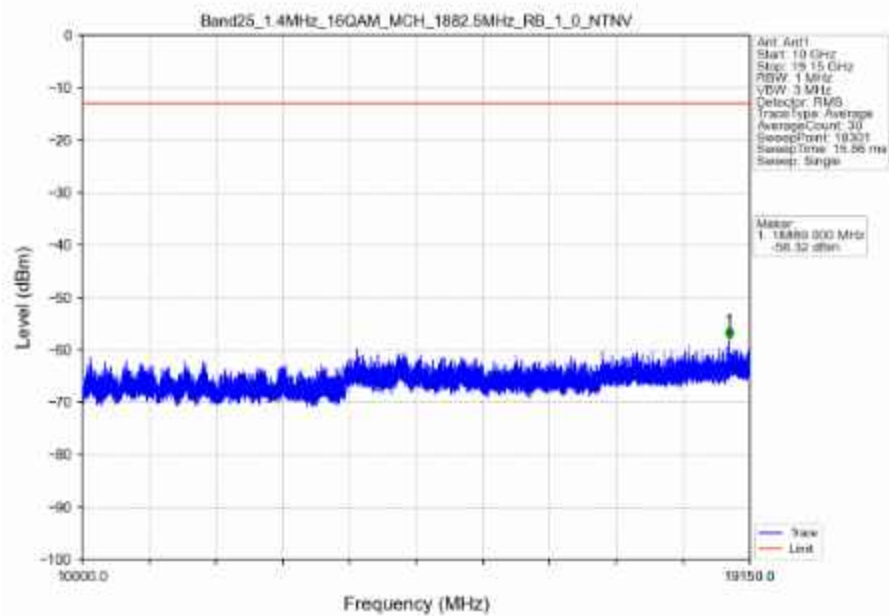
Band25_1.4MHz_16QAM_MCH_1882.5MHz_RB_1_0_NTNV
