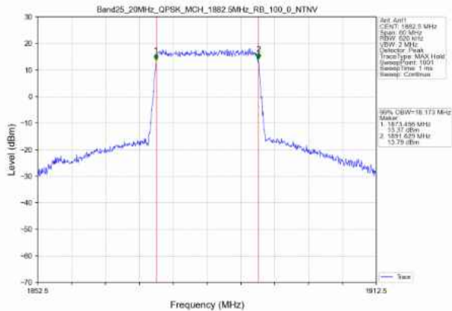
Band25_20MHz_QPSK_MCH_1882.5MHz_RB_100_0_NTNV
