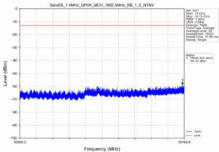
Band25_1.4MHz_QPSK_MCH_1882.5MHz_RB_1_0_NTNV
