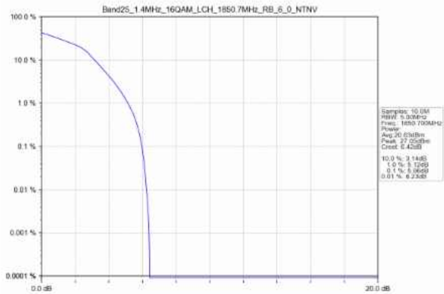
Band25_1.4MHz_16QAM_LCH_1850.7MHz_RB_6_0_NTNV
