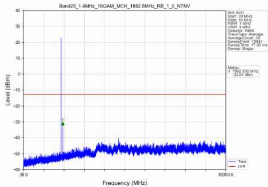
Band25_1.4MHz_16QAM_MCH_1882.5MHz_RB_1_0_NTNV
