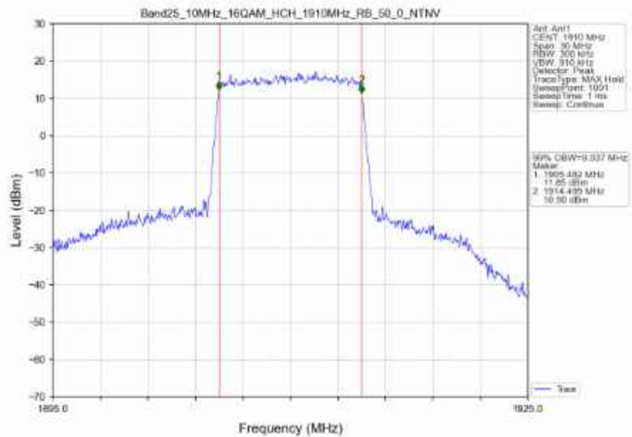
Band25_10MHz_16QAM_HCH_1910MHz_RB_50_0_NTNV
