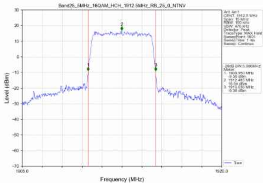
Band25_5MHz_16QAM_HCH_1912.5MHz_RB_25_0_NTNV
