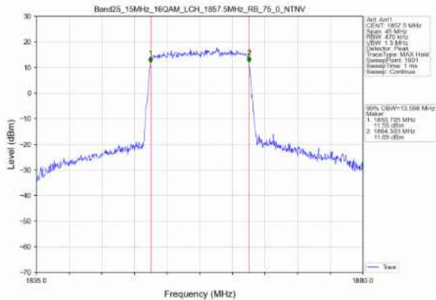
Band25_15MHz_16QAM_LCH_1857.5MHz_RB_75_0_NTNV
