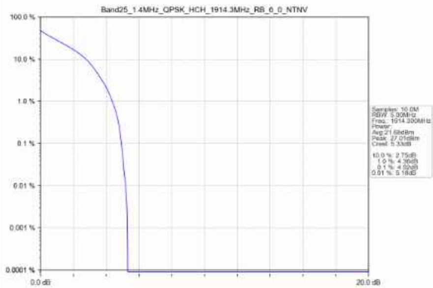
Band25_1.4MHz_QPSK_HCH_1914.3MHz_RB_6_0_NTNV
