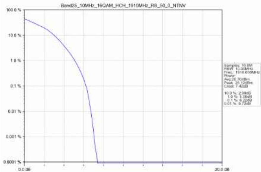
Band25_10MHz_16QAM_HCH_1910MHz_RB_50_0_NTNV
