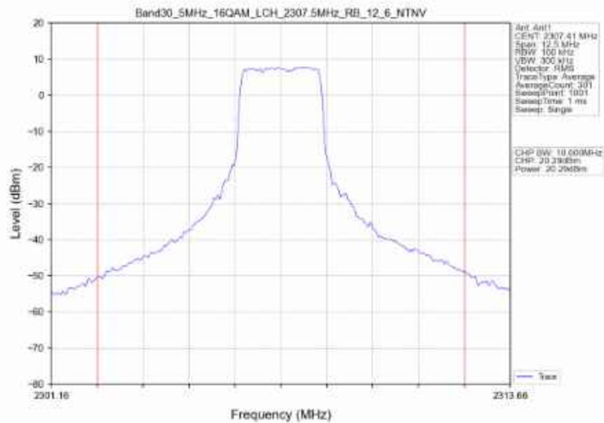
Band30_5MHz_16QAM_LCH_2307.5MHz_RB_12_6_NTNV
