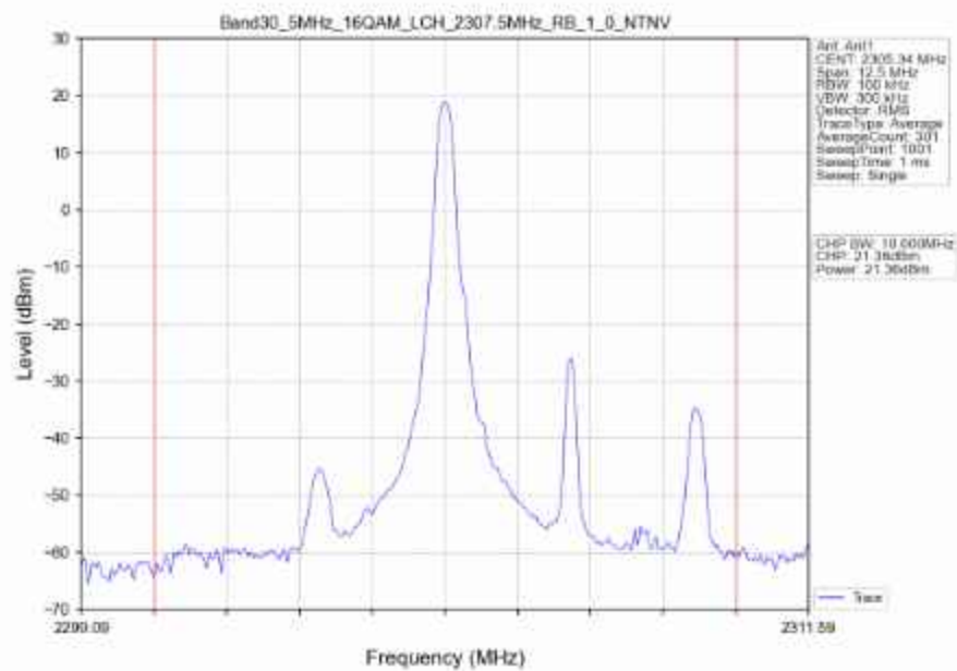
Band30_5MHz_16QAM_LCH_2307.5MHz_RB_1_0_NTNV
