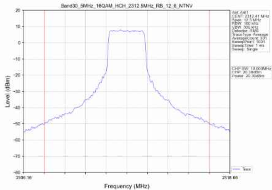
Band30_5MHz_16QAM_HCH_2312.5MHz_RB_12_6_NTNV
