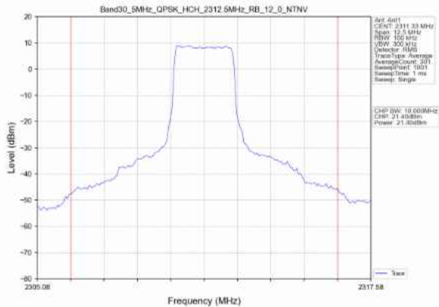
Band30_5MHz_QPSK_HCH_2312.5MHz_RB_12_0_NTNV
