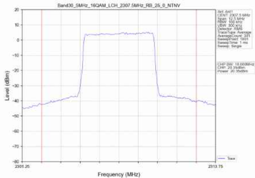
Band30_5MHz_16QAM_LCH_2307.5MHz_RB_25_0_NTNV
