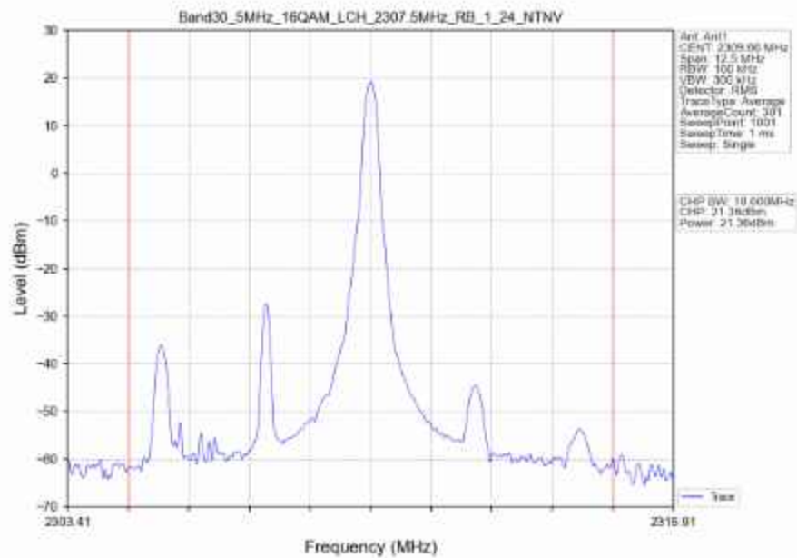
Band30_5MHz_16QAM_LCH_2307.5MHz_RB_1_24_NTNV
