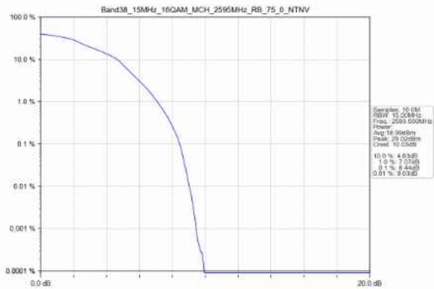
Band38_15MHz_16QAM_MCH_2595MHz_RB_75_0_NTNV
