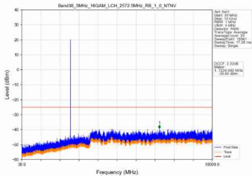
Band38_5MHz_16QAM_LCH_2572.5MHz_RB_1_0_NTNV
