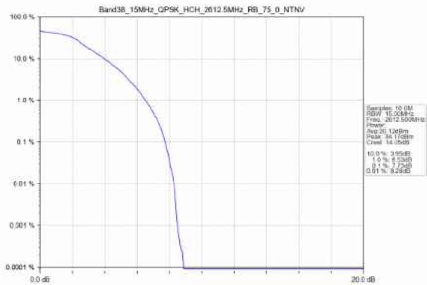
Band38_15MHz_QPSK_HCH_2612.5MHz_RB_75_0_NTNV
