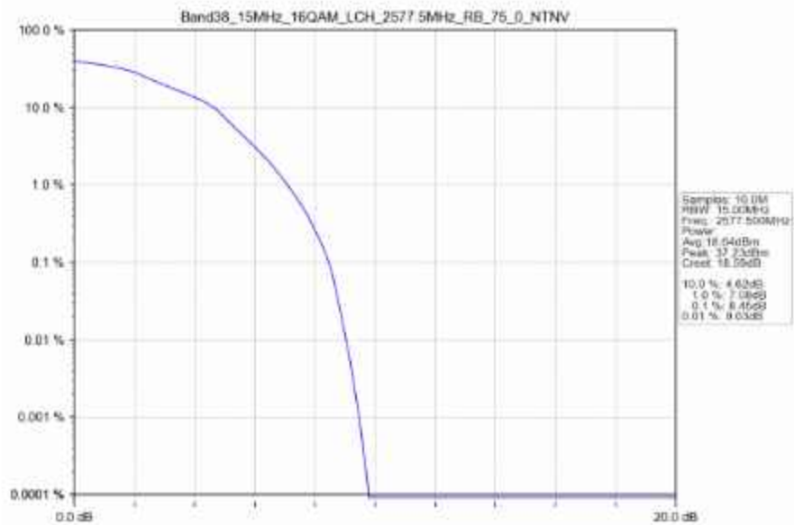
Band38_15MHz_16QAM_LCH_2577.5MHz_RB_75_0_NTNV
