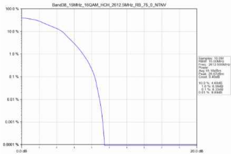
Band38_15MHz_16QAM_HCH_2612.5MHz_RB_75_0_NTNV
