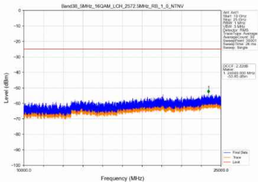
Band38_5MHz_16QAM_LCH_2572.5MHz_RB_1_0_NTNV
