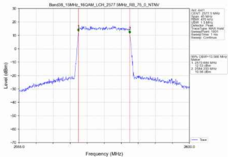
Band38_15MHz_16QAM_LCH_2577.5MHz_RB_75_0_NTNV
