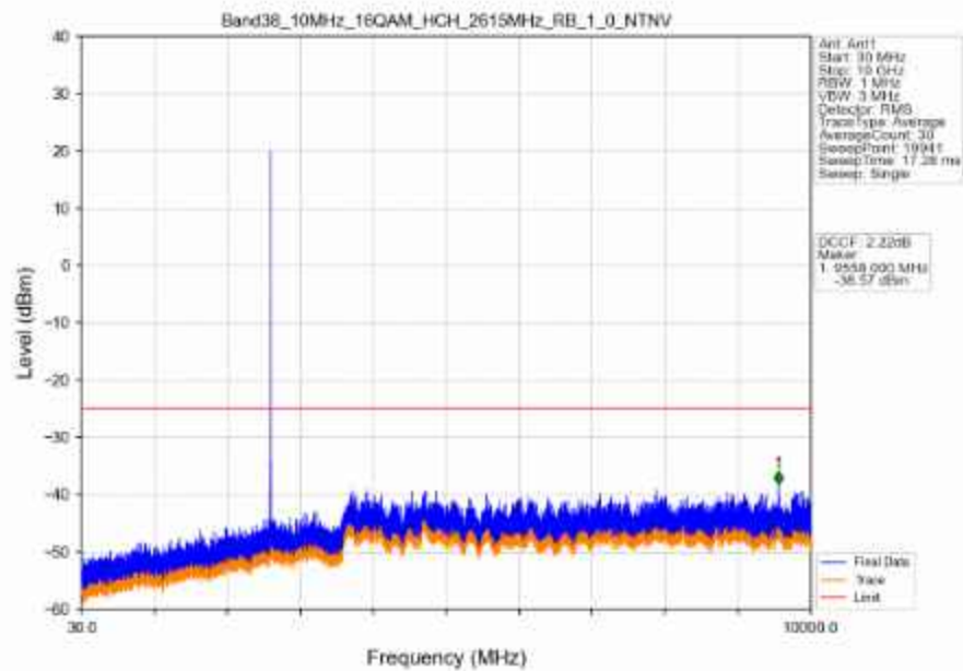
Band38_10MHz_16QAM_HCH_2615MHz_RB_1_0_NTNV
