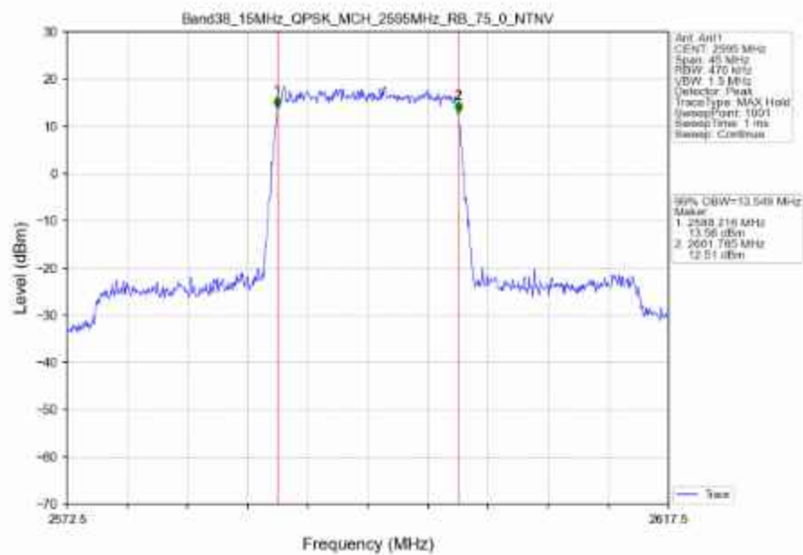
Band38_15MHz_QPSK_MCH_2595MHz_RB_75_0_NTNV
