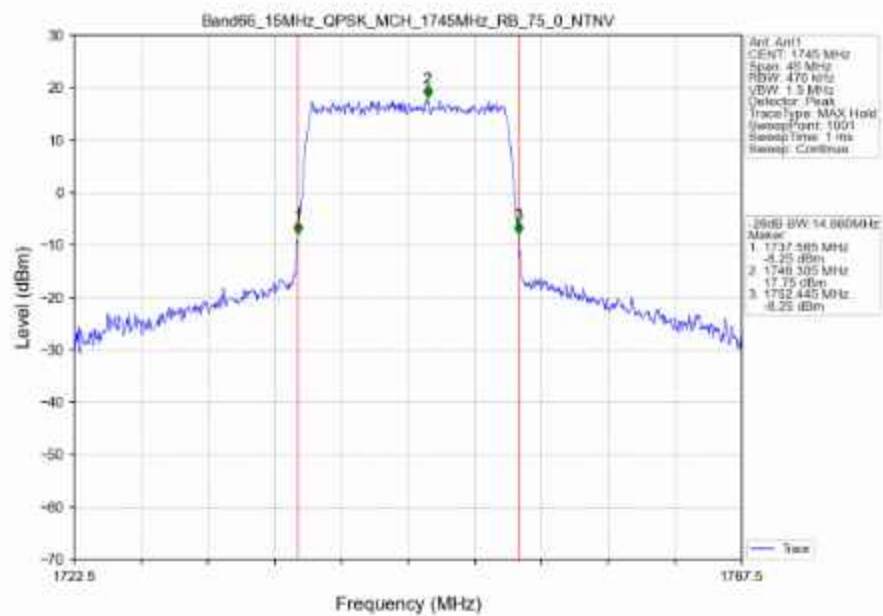
Band66_15MHz_QPSK_MCH_1745MHz_RB_75_0_NTNV
