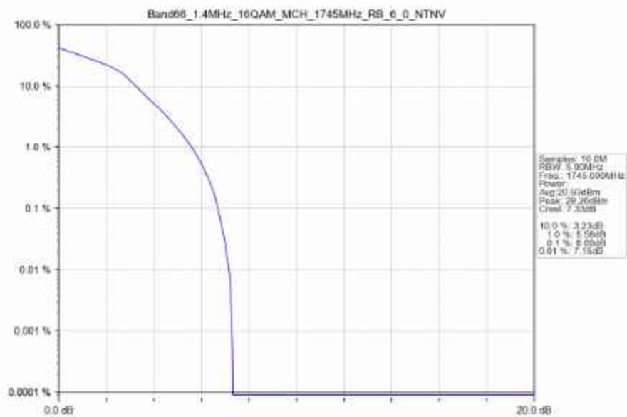
Band66_1.4MHz_16QAM_MCH_1745MHz_RB_6_0_NTNV
