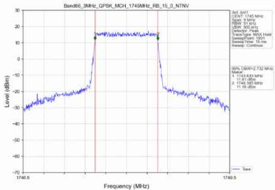
Band66_3MHz_QPSK_MCH_1745MHz_RB_15_0_NTNV
