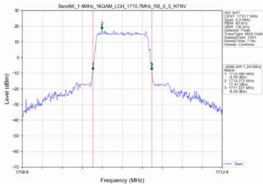
Band66_1.4MHz_16QAM_LCH_1710.7MHz_RB_6_0_NTNV
