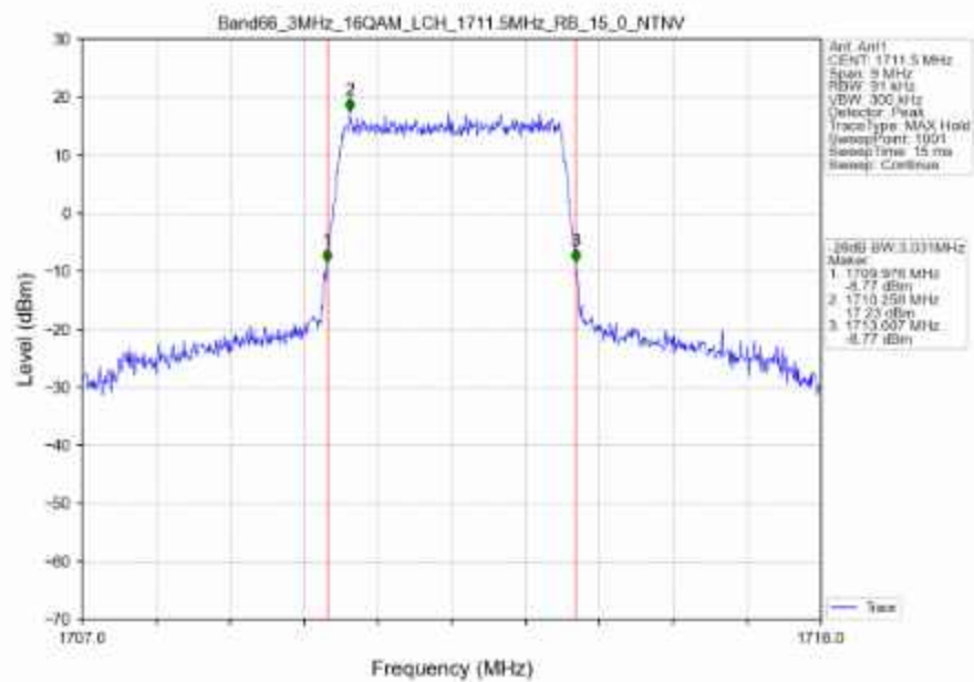
Band66_3MHz_16QAM_LCH_1711.5MHz_RB_15_0_NTNV
