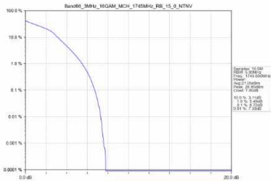
Band66_3MHz_16QAM_MCH_1745MHz_RB_15_0_NTNV
