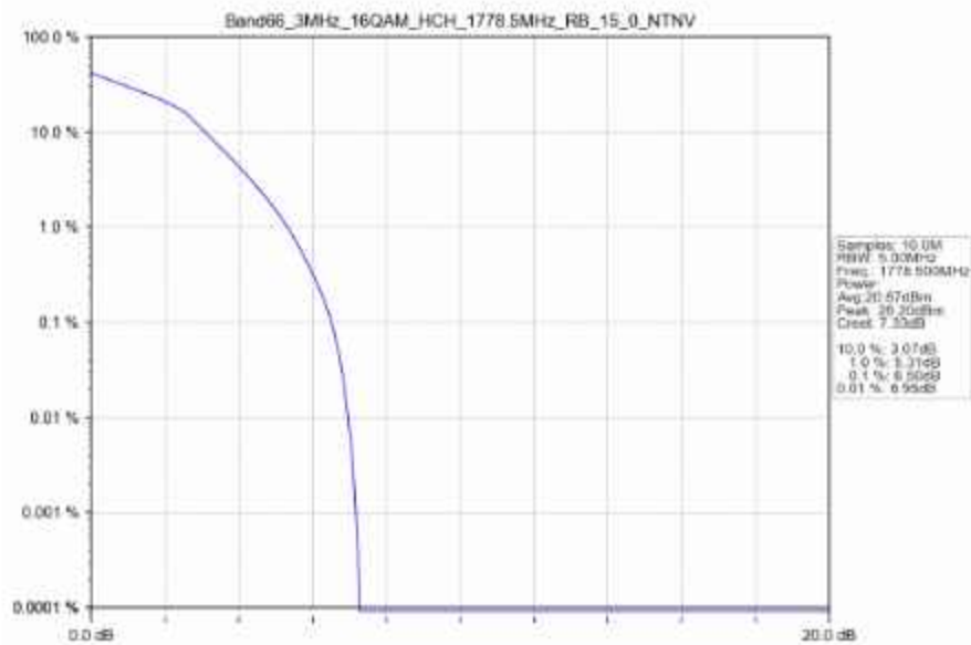
Band66_3MHz_16QAM_HCH_1778.5MHz_RB_15_0_NTNV
