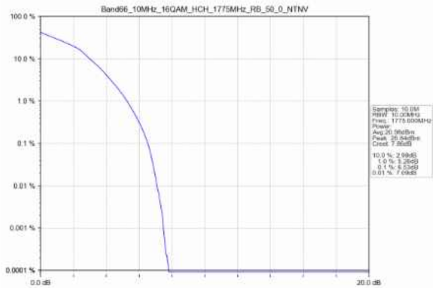
Band66_10MHz_16QAM_HCH_1775MHz_RB_50_0_NTNV
