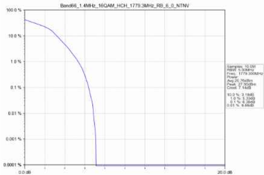
Band66_1.4MHz_16QAM_HCH_1779.3MHz_RB_6_0_NTNV
