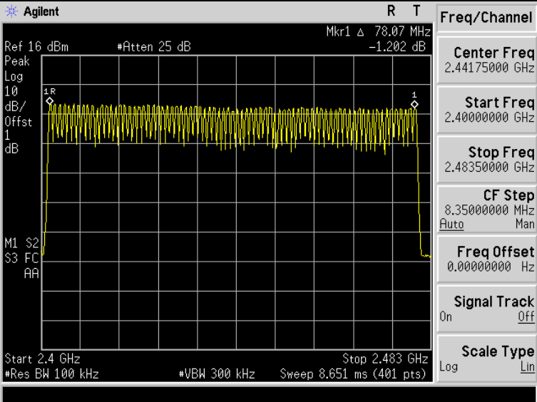
GFSK Modulation
