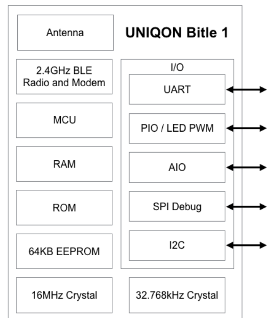
Fig 2. Block Diagram
