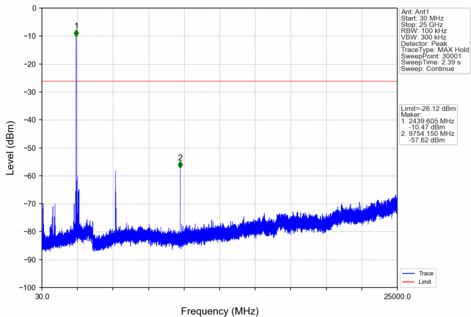
GFSK_MCH_2440MHz_Ant1_NTNV
