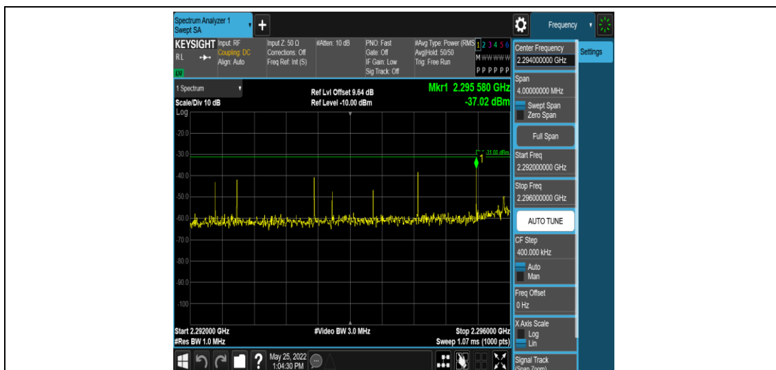
Band40-5MHz-16QAM-38725-1RB#0-Range6:2292~2296MHz
