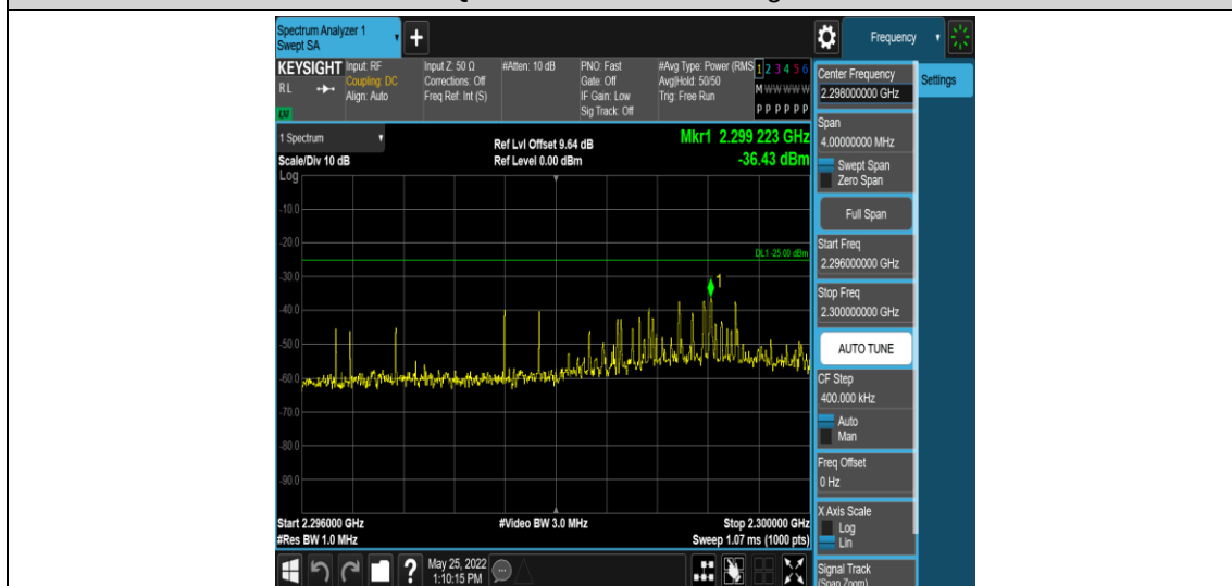
Band40-5MHz-16QAM-38750-1RB#0-Range7:2296~2300MHz
