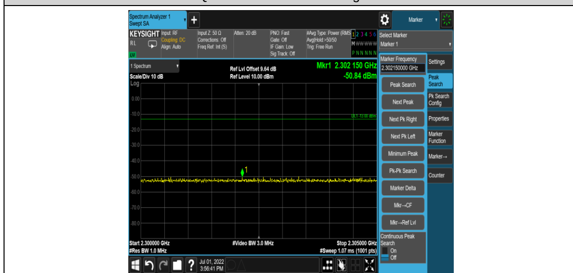
Band40-5MHz-QPSK-38750-1RB#0-Range8:2300~2305MHz
