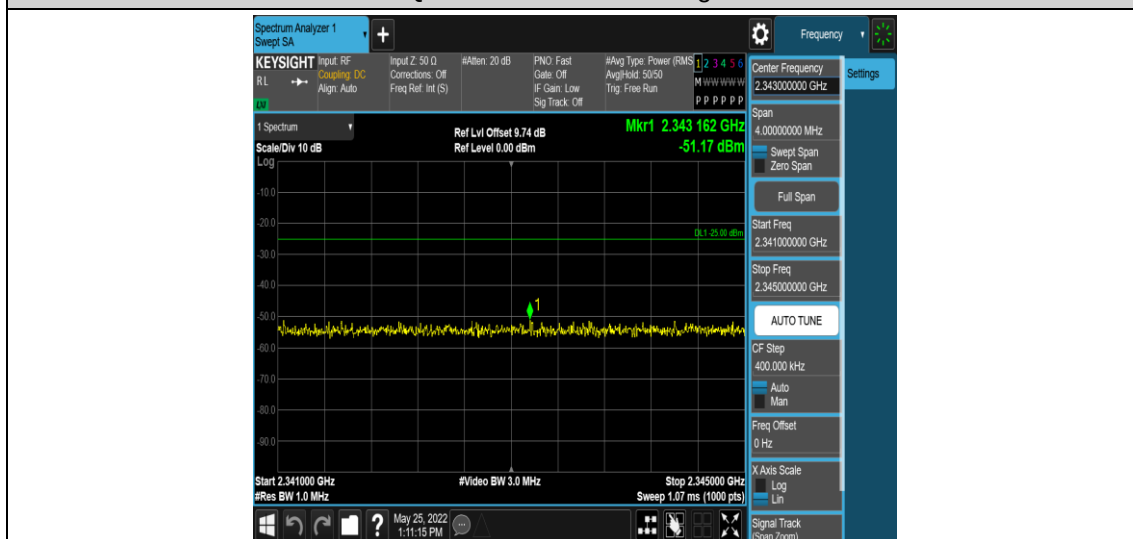
Band40-5MHz-16QAM-38750-1RB#0-Range13:2341~2345MHz
