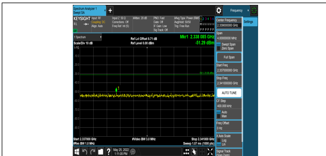
Band40-5MHz-16QAM-38750-1RB#0-Range12:2337~2341MHz
