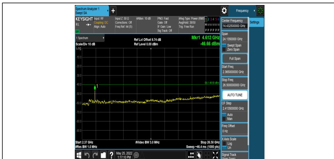
Band40-5MHz-16QAM-38775-1RB#0-Range15:2365~26500MHz
