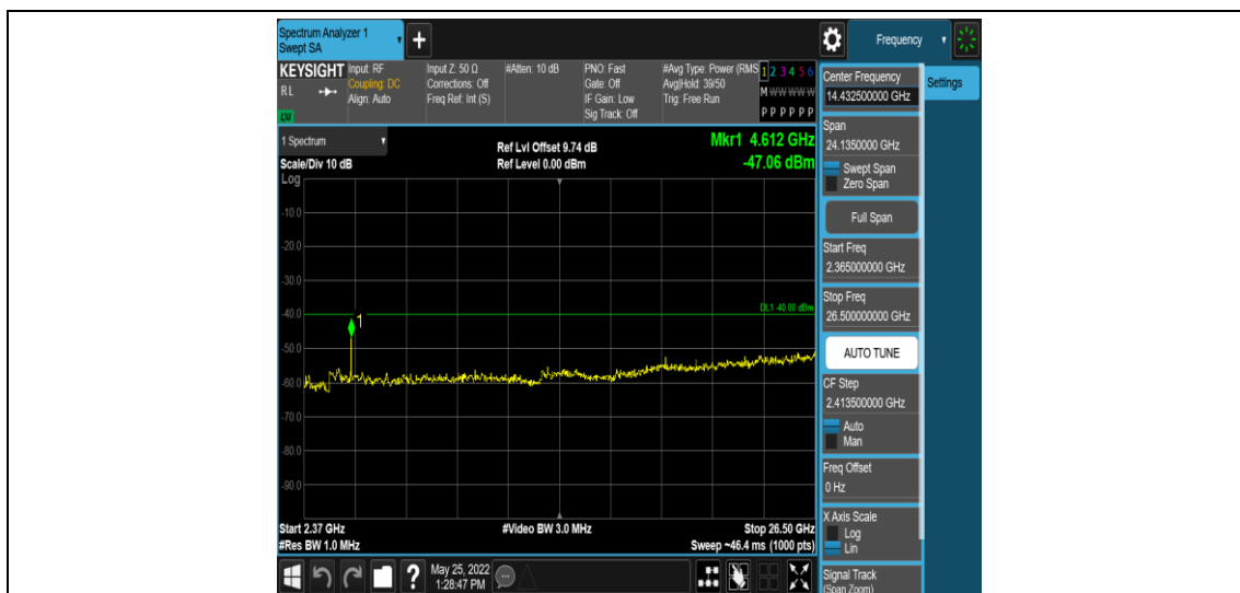
Band40-10MHz-QPSK-38750-1RB#0-Range15:2365~26500MHz
