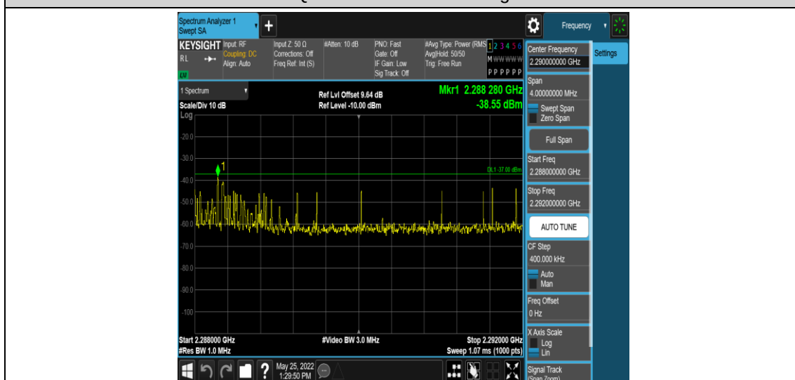
Band40-10MHz-16QAM-38750-1RB#0-Range5:2288~2292MHz
