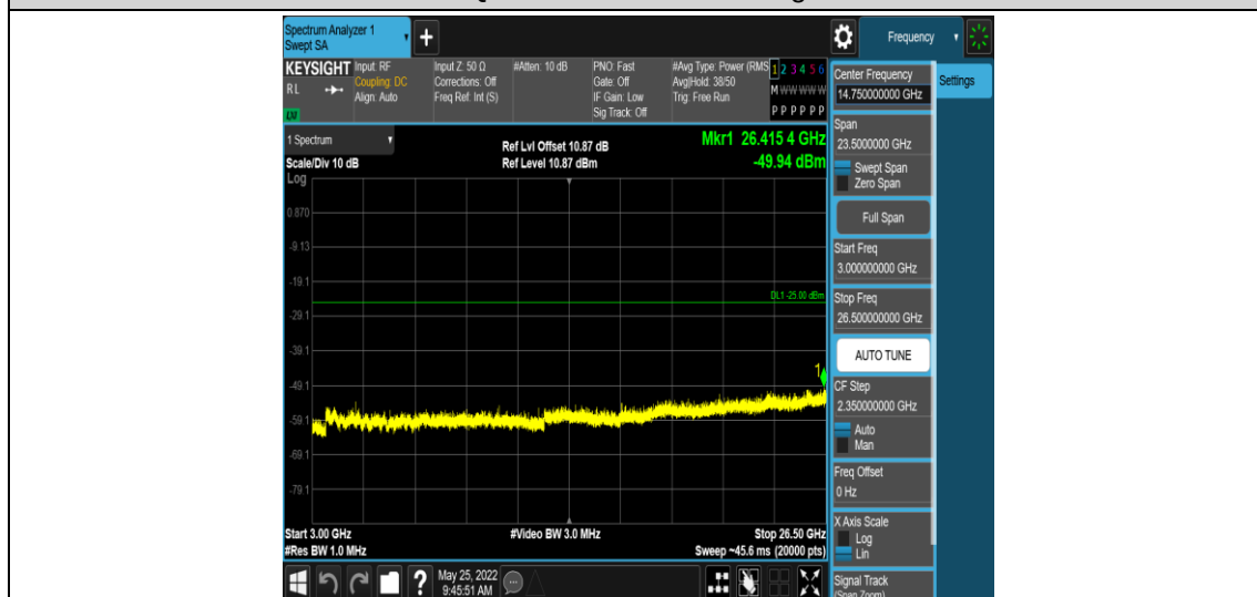
Band41-15MHz-16QAM-39725-1RB#0-Range5:3000~26500MHz
