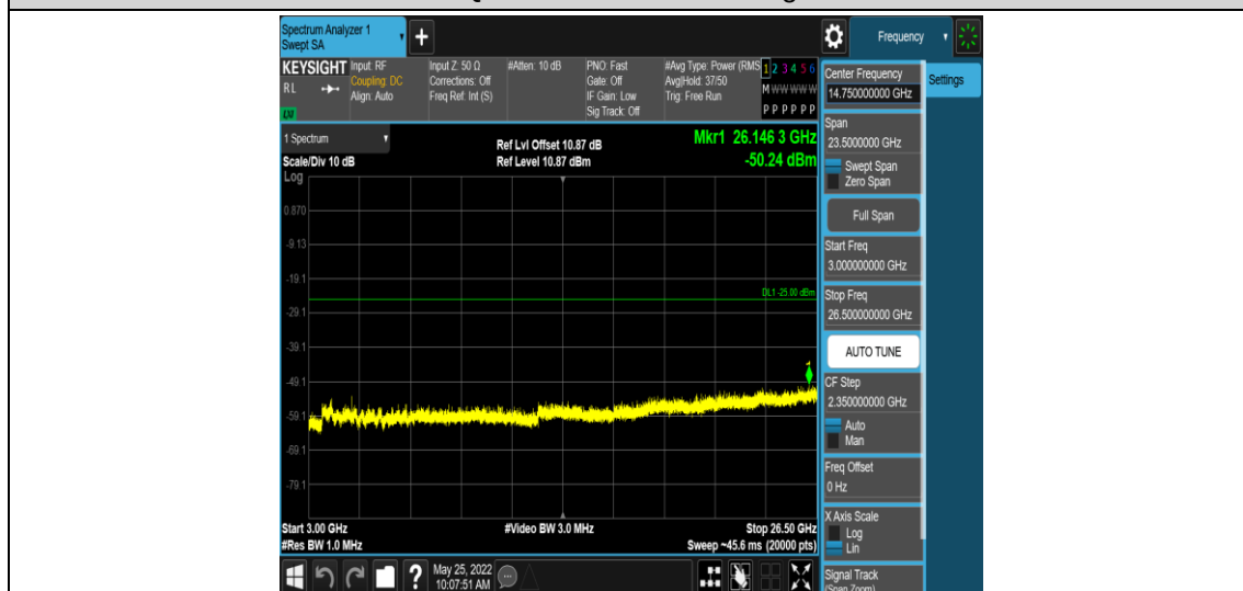
Band41-20MHz-16QAM-39750-1RB#0-Range5:3000~26500MHz
