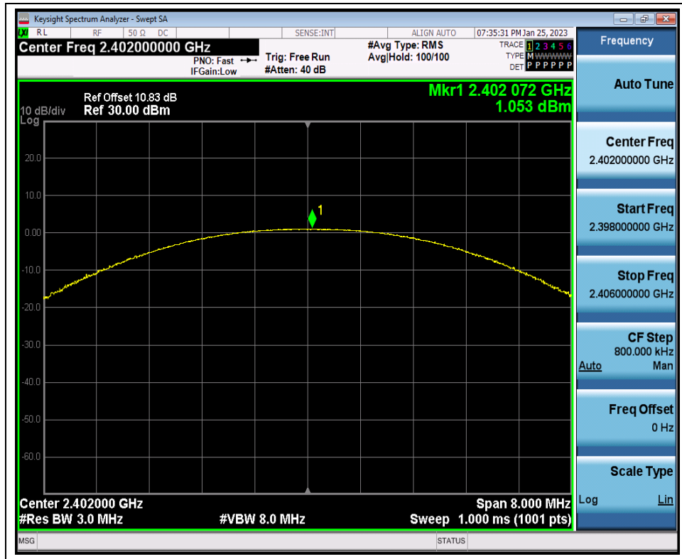
(Channel 0, GFSK)
