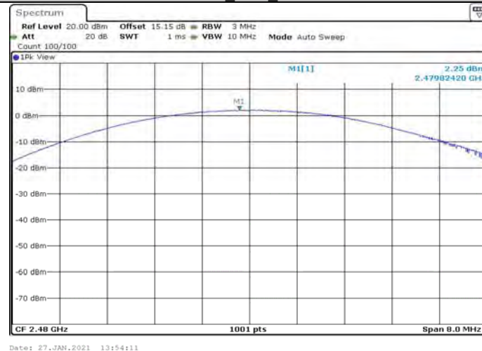
2DH1_Ant1_2480
