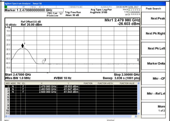
Channel 39 / 2480 MHz – Average
