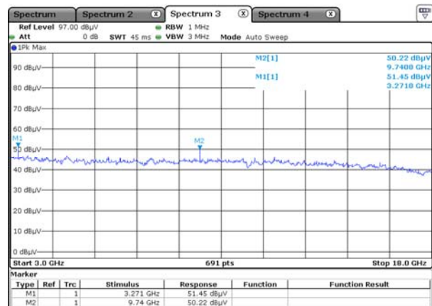
Vertical // Peak for 3 GHz to 18 GHz
