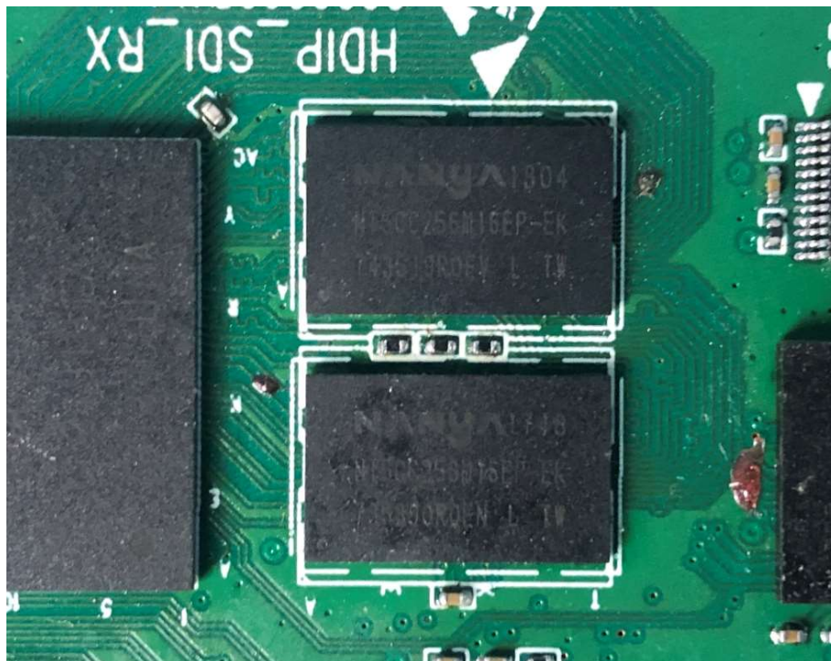
Photo 12(Receiver)
