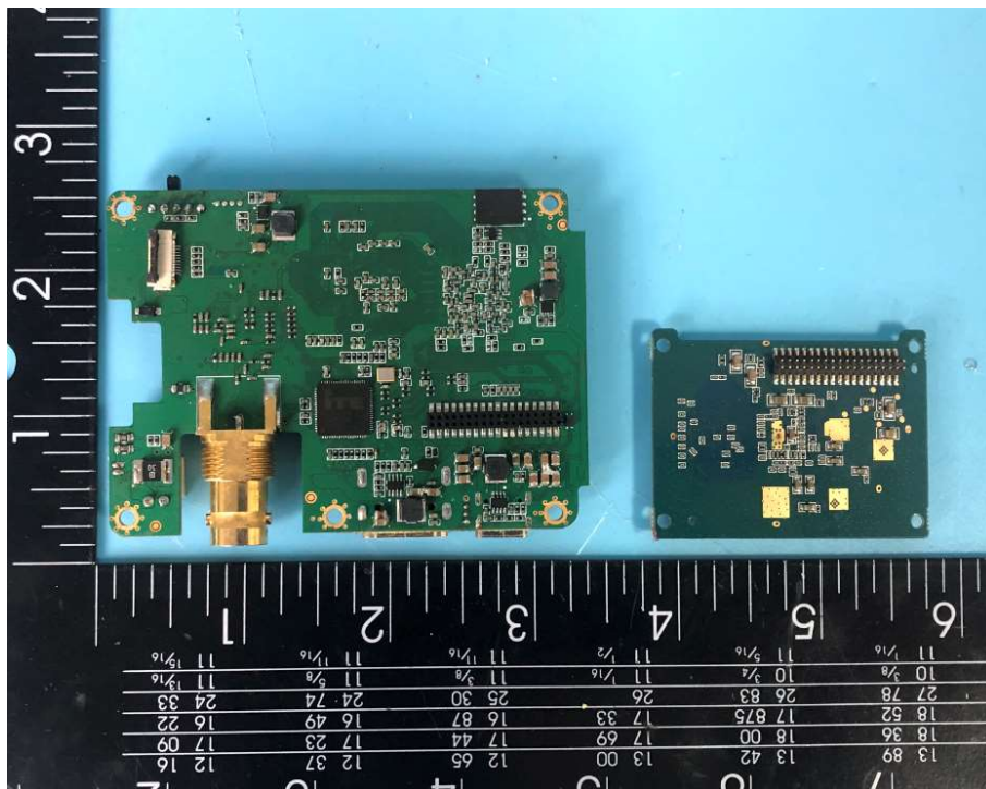
Photo 7(Receiver)
