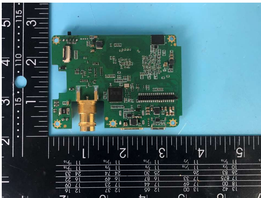
Photo 8(Receiver)
