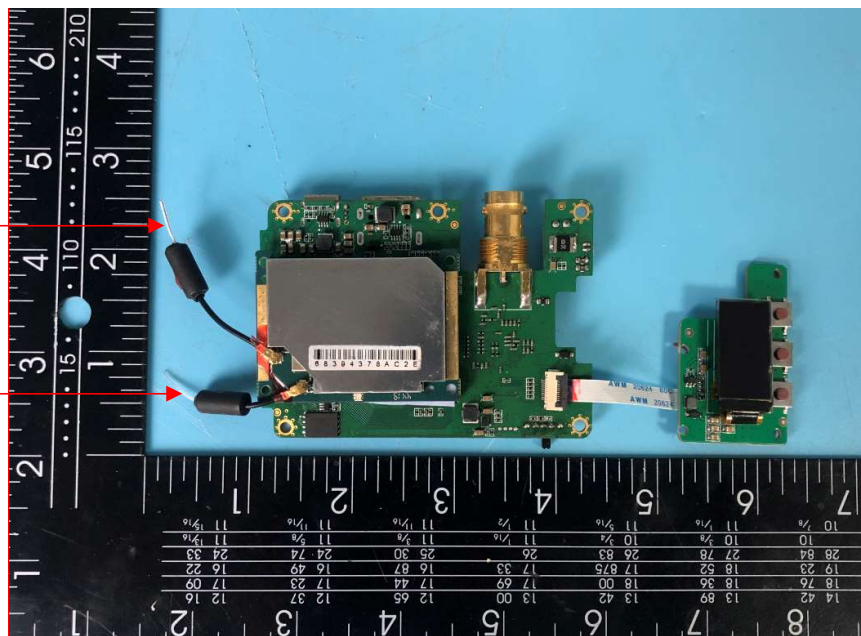
Photo 2(Receiver)
