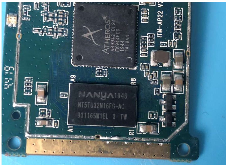
Photo 17(Receiver)
