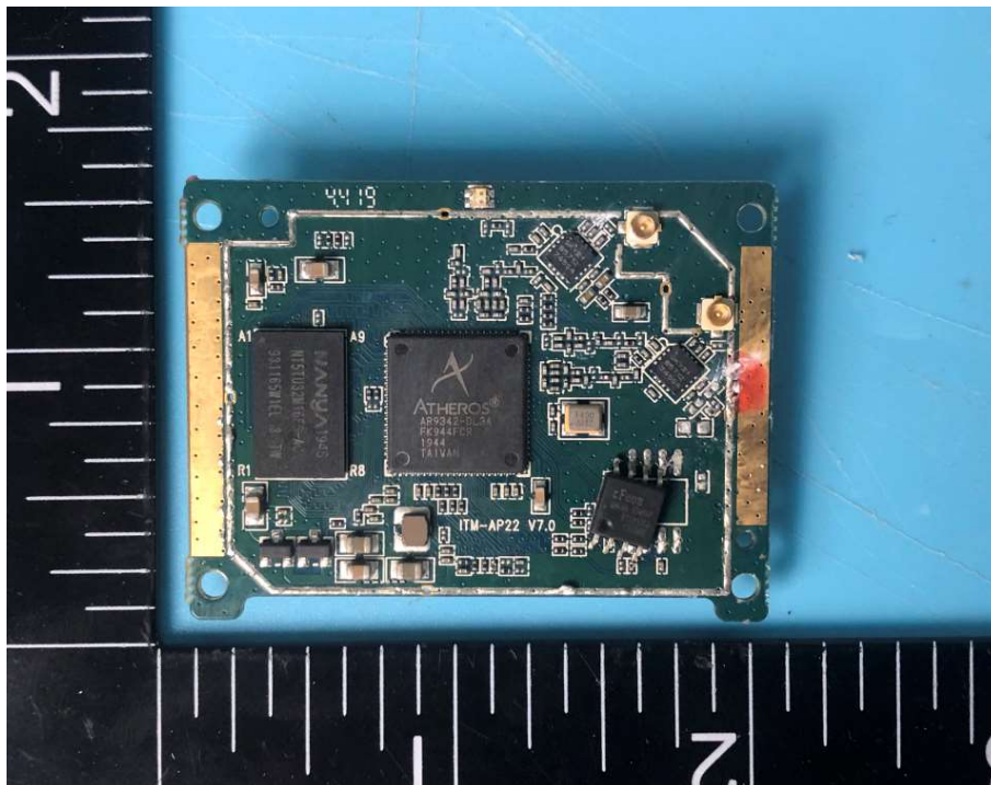
Photo 16(Receiver)
