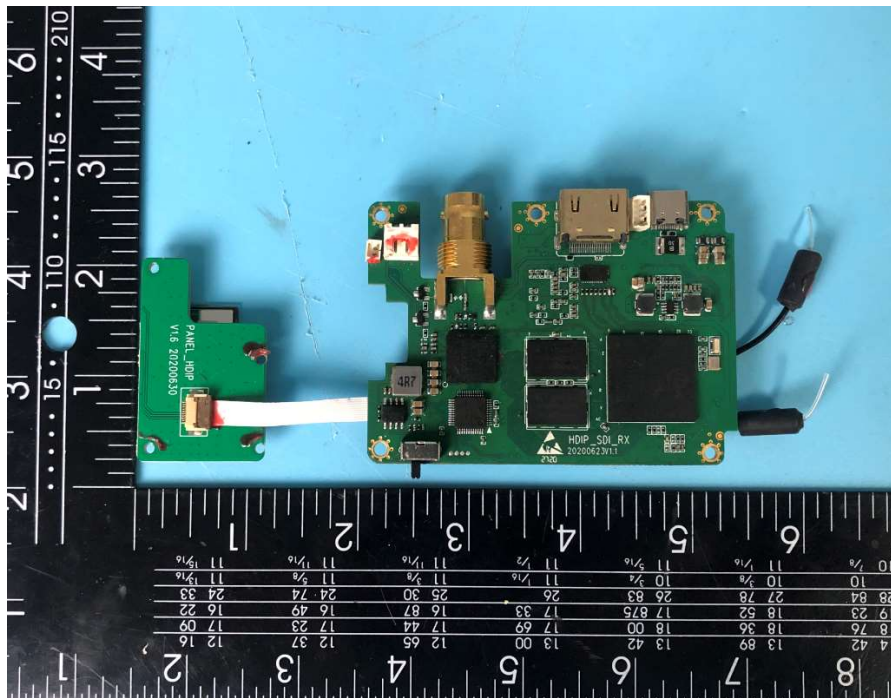
Photo 3(Receiver)
