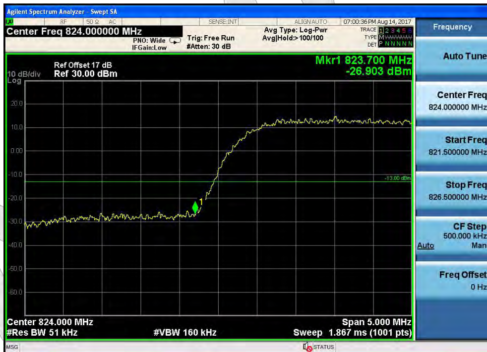
Test Mode: Band V - Low Channel
