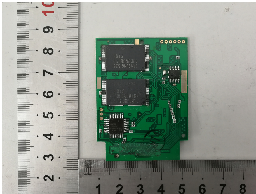
EUT –PCB-4(No Shielding) Bottom View
