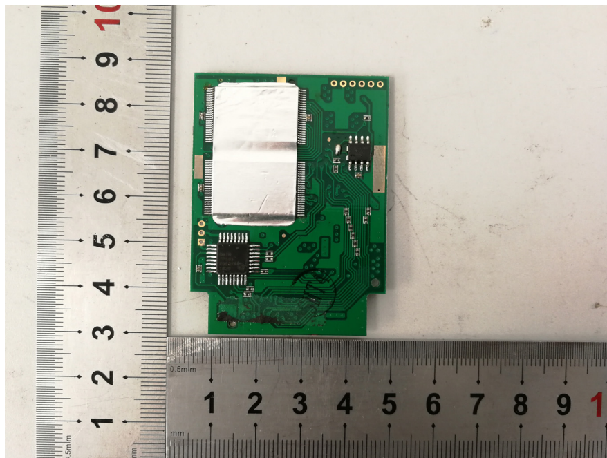
EUT-PCB-4(Shielding) Bottom View
