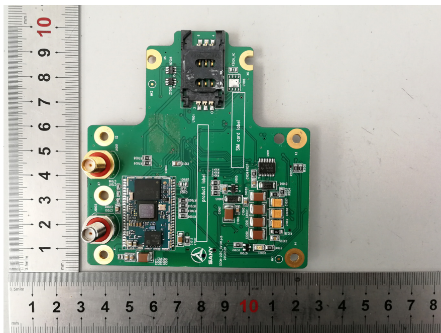
EUT-PCB-1 (No Shielding) Top View
