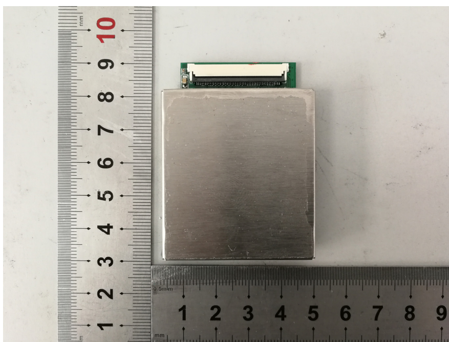
EUT-PCB-4(Shielding) Top View
