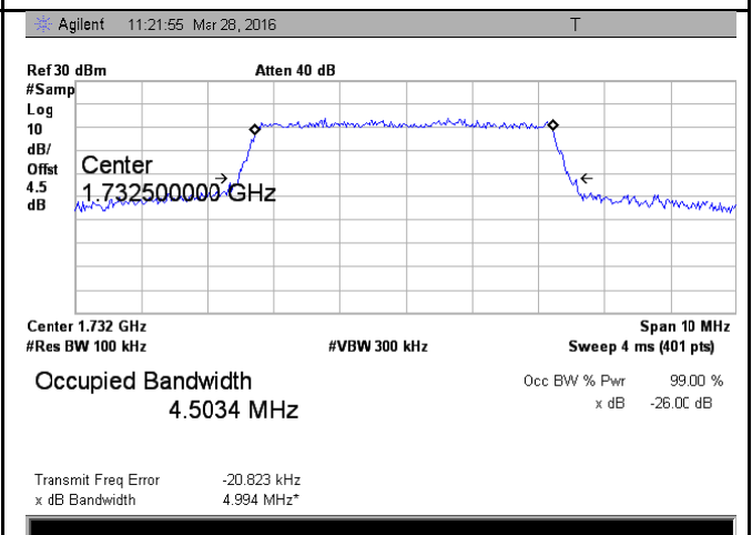
LTE band 4- MiddleCH 16QAM-5
