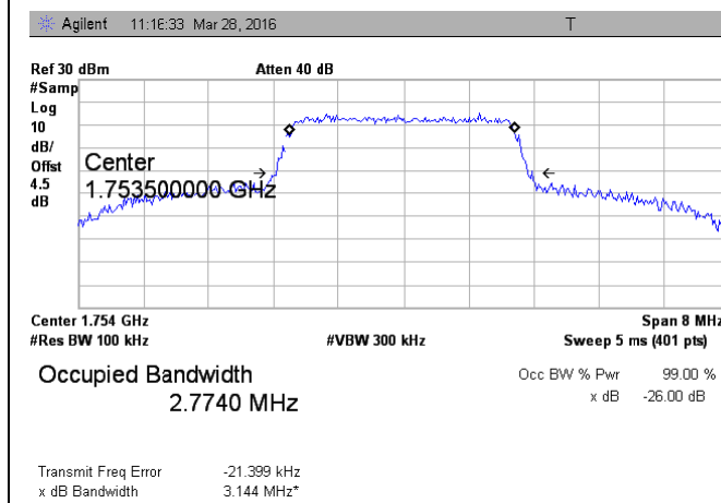
LTE band 4- HighCH QPSK-3
