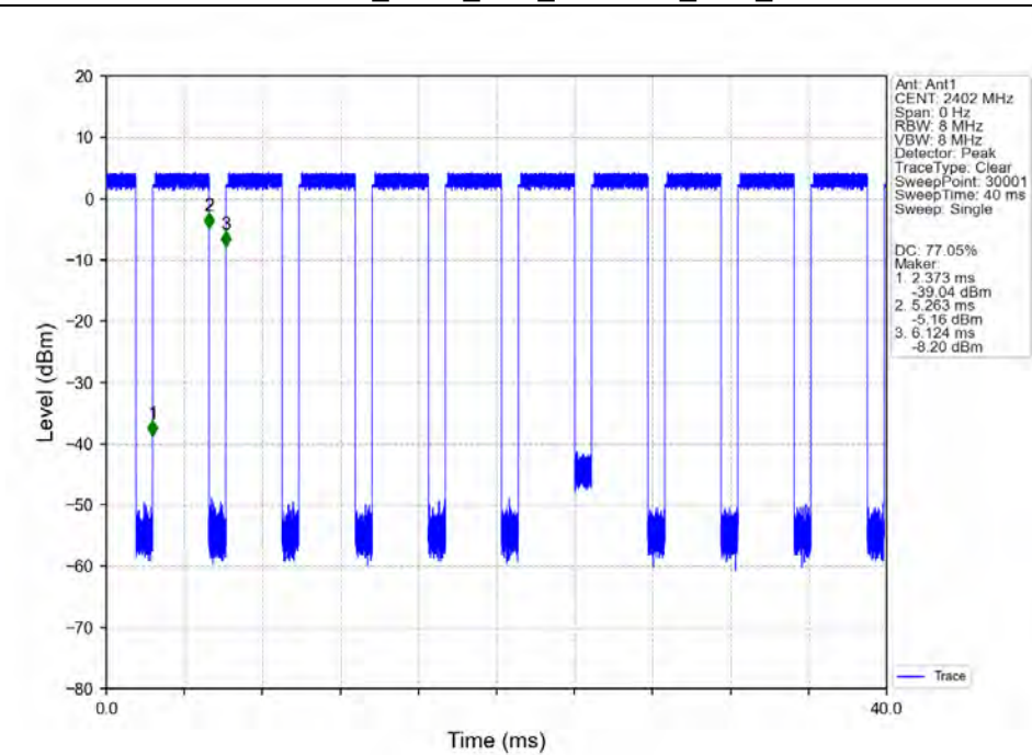
Pi/4DQPSK_2DH5_LCH_2402MHz_Ant1_NTNV
