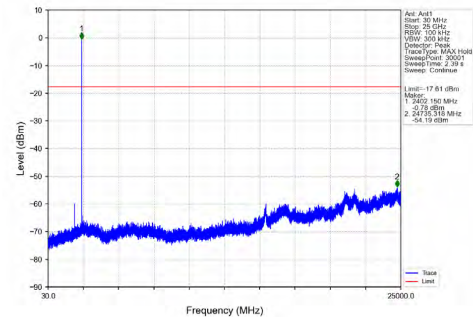
8DPSK_3DH5_LCH_2402MHz_Ant1_NTNV
