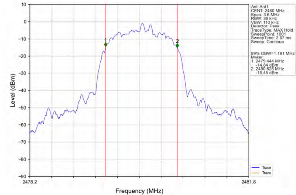
8DPSK_3DH5_HCH_2480MHz_Ant1_NTNV
