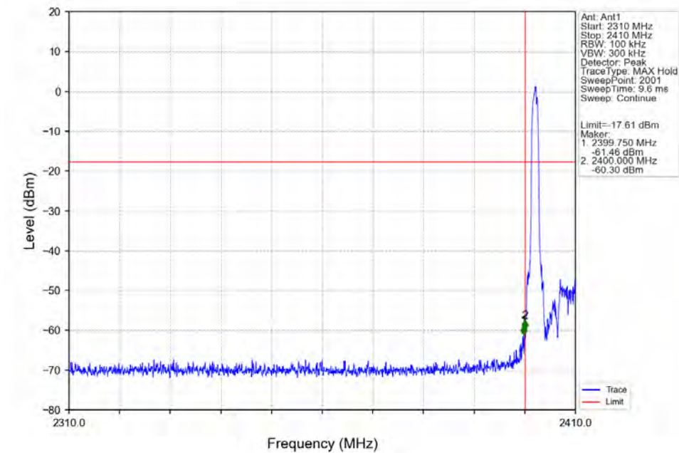
8DPSK_3DH5_LCH_2402MHz_Ant1_NTNV
