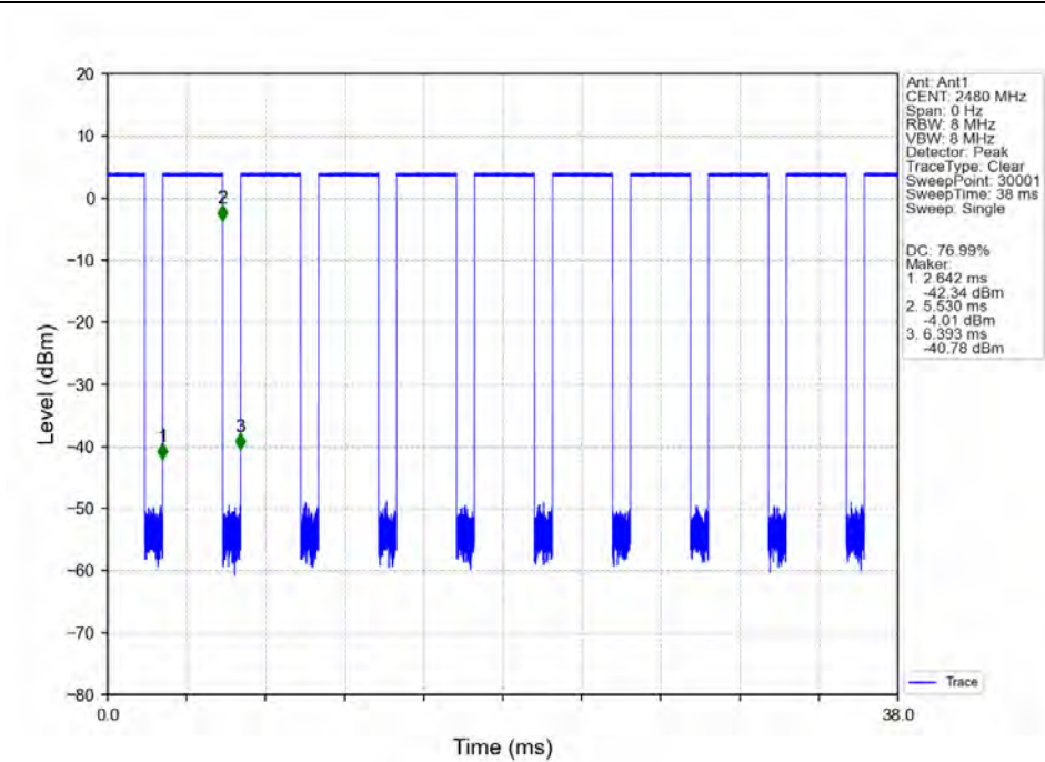
GFSK_DH5_HCH_2480MHz_Ant1_NTNV
